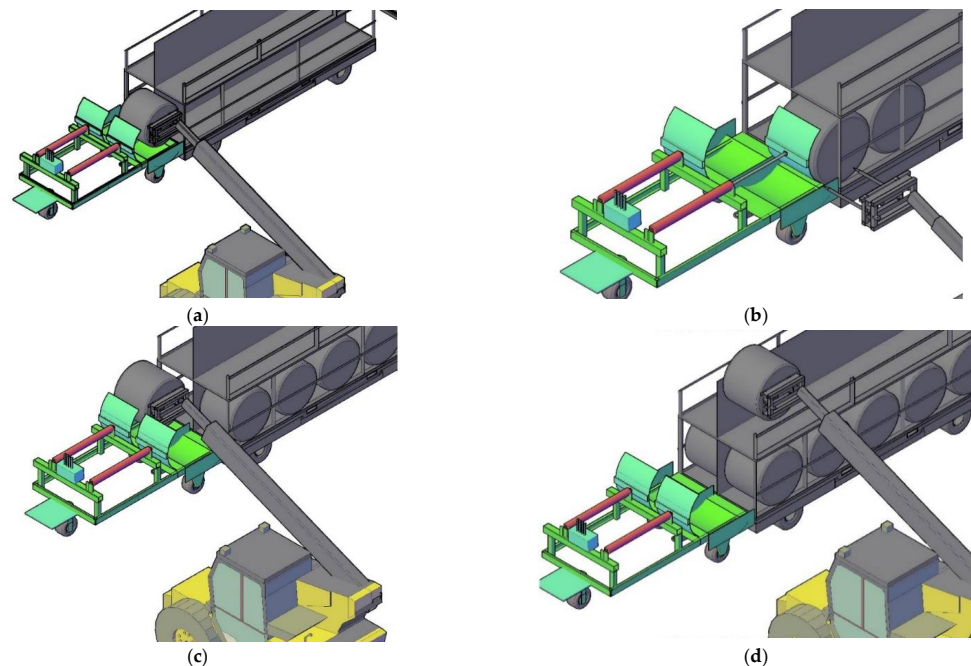
Figure 5. (a) Telehandler placing bale into bale loader used to load bales into bottom tier chamber of rack, (b) Bale loader shown inserting a second bale into the bottom tier chamber of rack. (c) Filling back lower-tier chamber. (d) Concept for telehandler loading bales in top tier chambers.
