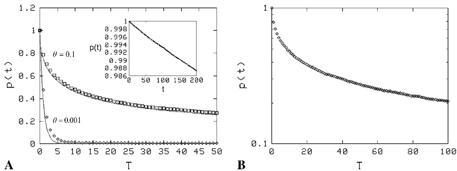
FIGURE 3 (A) Receptor density impacts ligand dissociation for a uniform distribution of receptors. The value p(t) versus scaled time T = \beta t ( t is measured in number of Monte Carlo time steps) is plotted for \theta = 0.001 and \theta = 0.1 . The former displays exponential decay, whereas the latter is clearly nonexponential over the timescales shown. The lines are theoretical fits: e^{-k_+ t} in the former case and the function in Eq. 11b in the latter case with c = 0.08 (the theoretical value from Eq. 11 is 0.06). The early time behavior of the high-density case ( \theta = 0.1 ) plotted in the inset does indicate
