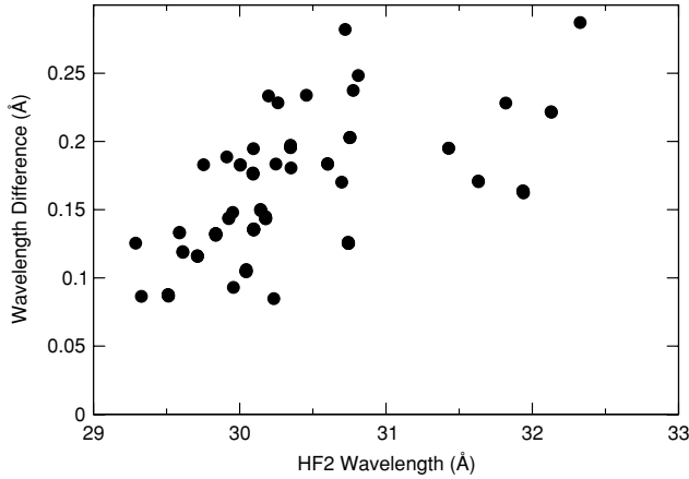
Figure 3. Wavelength differences between MCDF (Chen & Crasemann 1987) and HF2 for N IV. An average difference of 155 \pm 45 \text{ m\AA} is observed.
