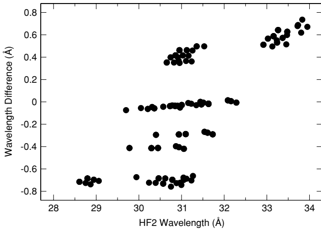
Figure 4. Wavelength differences between MCDF (Chen et al. 1997) and HF2 for N II. Differences as large as 800 \text{ m\AA} are observed.
