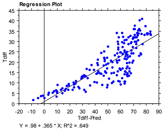
Figure V-6 Plot of the regression output for C1-3's predictability
