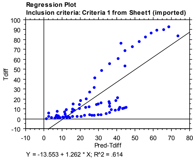
Figure V-16 Plot of the regression output for C3-2's predictability
