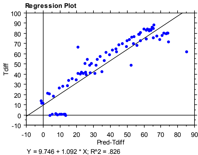
Figure V-8 Plot of the regression output for C2-1's predictability
