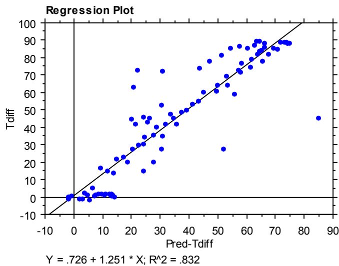
Figure V-14 Plot of the regression output for C3-1's predictability
