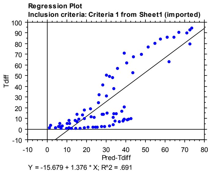
Figure V-10 Plot of the regression output for C2-2's predictability
