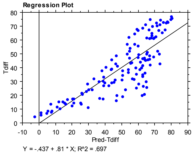
Figure V-18 Plot of the regression output for C3-3's predictability
