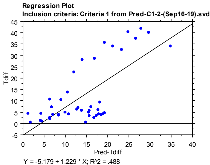
Figure V-4 Plot of the regression output for C1-2's predictability
