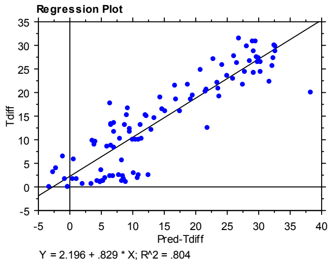
Figure V-2 Plot of the regression output for C1-1's predictability
