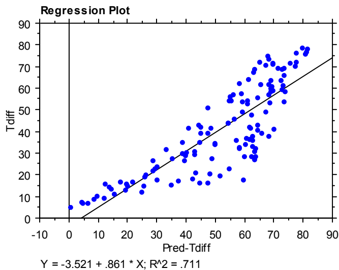
Figure V-12 Plot of the regression output for C2-3's predictability
