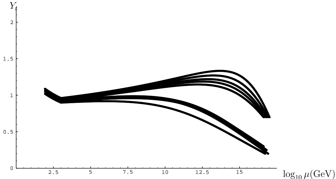
Figure 6: The running of the top Yukawa coupling for typical values of (\alpha_{\text{GUT}}, M_{\text{GUT}}) shown in Fig. 2. The value of \alpha_{\text{GUT}} is varied between 0.3 and 0.8 while Y_t(M_{\text{GUT}}) = Y_{\text{GUT}} is varied between 0.2 and 0.7. The Yukawa coupling is multiplied by \sin \beta below M_{\text{SUSY}} .
