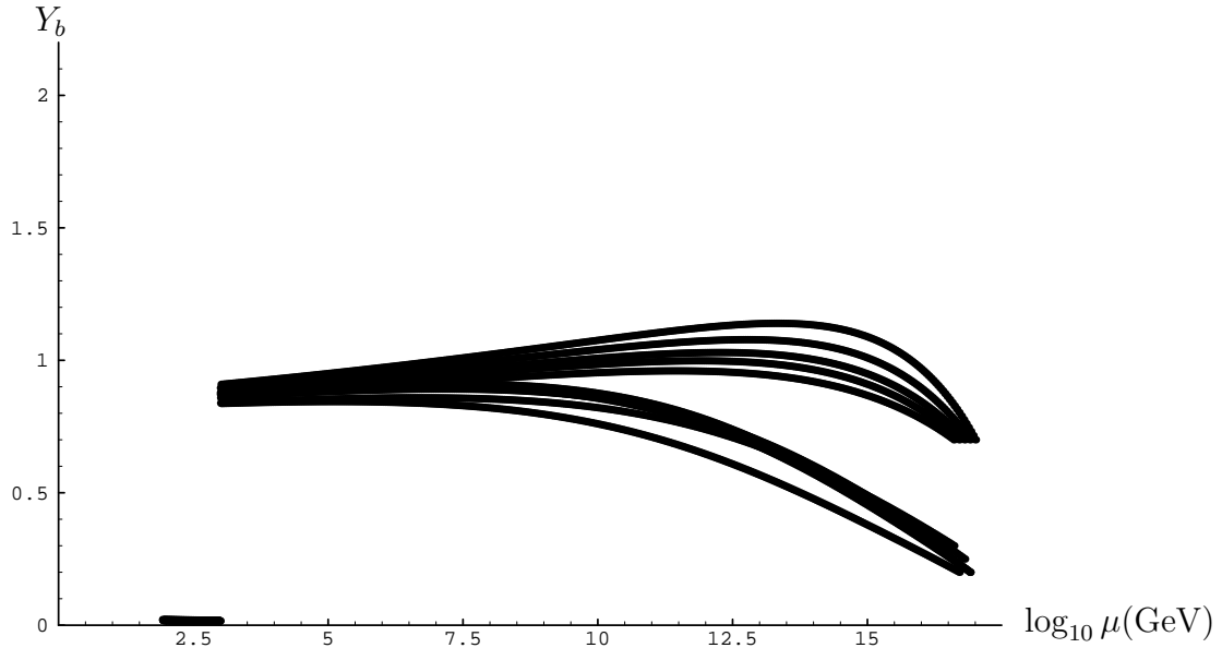
Figure 5: The running of the bottom Yukawa coupling for typical values of (\alpha_{\text{GUT}}, M_{\text{GUT}}) shown in Fig. 2. The value of \alpha_{\text{GUT}} is varied between 0.3 and 0.8 while Y_b(M_{\text{GUT}}) = Y_{\text{GUT}} is varied between 0.2 and 0.7. The Yukawa coupling is multiplied by \cos \beta below M_{\text{SUSY}} .
