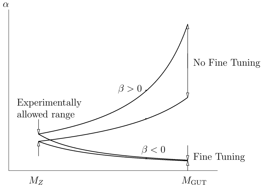
Figure 1: The difference between asymptotically free and non-free theories.
