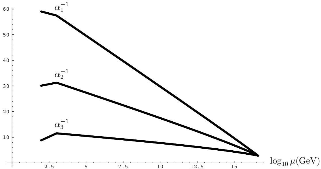
Figure 3: Typical \mu dependence of \alpha_1(\mu) , \alpha_2(\mu) and \alpha_3(\mu) . The parameter values for this plot were (\alpha_{\text{GUT}}, Y_{\text{GUT}}, M_{\text{GUT}}, \tan\beta) = (0.35, 0.3, 10^{16.6}\text{GeV}, 57.5) .
