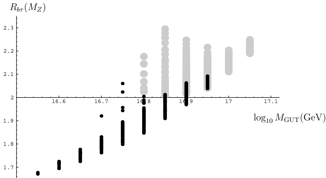
Figure 7: The dependence of R_{b\tau}(M_Z) on M_{\text{GUT}} and \alpha_{\text{GUT}} . The small-black, and large-gray circles indicate the ranges 0.3 < \alpha_{\text{GUT}} \leq 0.6 , and 0.6 < \alpha_{\text{GUT}} < 1 , respectively. The dependence of R_{b\tau}(M_Z) on Y_{\text{GUT}} is negligible.
