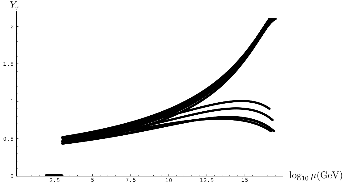
Figure 4: The running of the \tau -lepton Yukawa coupling for typical values of (\alpha_{\text{GUT}}, M_{\text{GUT}}) shown in Fig. 2. The value of \alpha_{\text{GUT}} is varied between 0.3 and 0.8 while Y_\tau(M_{\text{GUT}}) = 3Y_{\text{GUT}} is varied between 0.6 and 2.1. The Yukawa coupling is multiplied by \cos \beta below M_{\text{SUSY}} .
