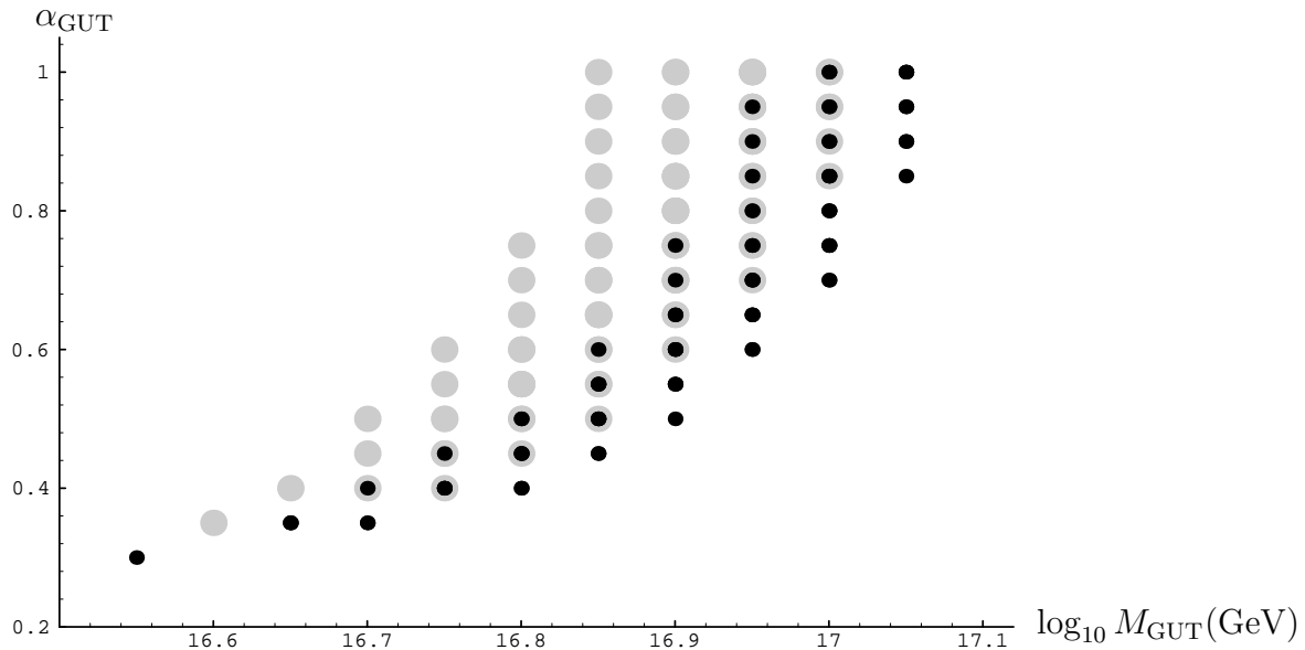
Figure 2: The allowed region in the plane (\alpha_{\text{GUT}}, M_{\text{GUT}}) . The small-black, and large-gray circles indicate the ranges 0.4 \leq Y_{\text{GUT}} < 0.7 , and 0.1 < Y_{\text{GUT}} < 0.4 , respectively.
