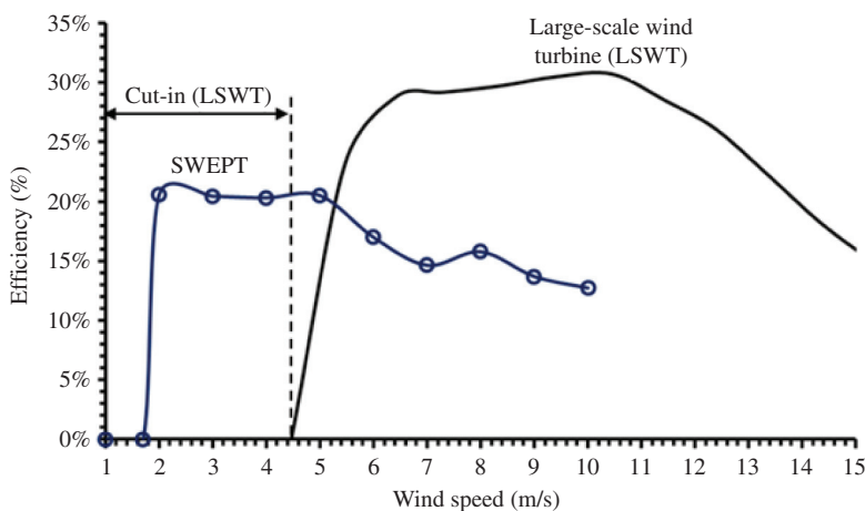
Figure 23 Power efficiency curve of SWEPT vs a conventional LSWT
