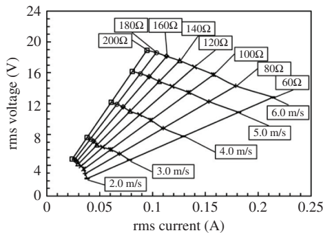
Figure 16 Voltage vs current at various loading conditions and wind speeds
