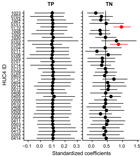
FIG. 4. Effect of watershed land use ( \gamma_j ) for individual regions in the top-ranked lake N and P models. Values shown are posterior medians (solid circles) and 95% credible intervals (solid lines) for individual hydrologic units (HUC4s) ordered from top to bottom according to longitude (west to east). Also shown is a comparison to a zero effect (solid vertical line). Values that are different from the population level effect are shaded in red.
