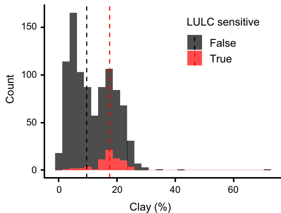
FIG. 6. Histograms showing the distribution of soil clay content for watersheds in regions sensitive to watershed land use (see highlighted credible intervals in Fig. 4) relative to watersheds all other regions. Medians for each group are shown as vertical dashed lines.
