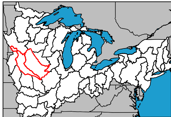
FIG. 5. Location of hydrologic regions sensitive to watershed land-use cover corresponding to highlighted credible intervals in Fig. 4.
