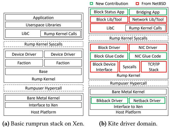
(a) Basic rumprun stack on Xen.
