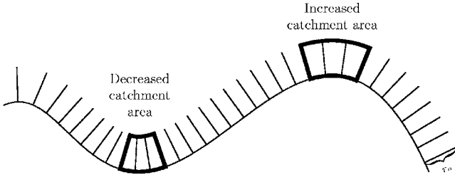
FIG. 2. Schematic representation of the growth inhibition and amplification by either finite adatom radii ( r_o ) or steering. In both cases, the flux contributing to growth at some point on the surface is to be measured a distance r_o normal to the surface. The left box shows the reduced effective surface in valleys, the right one the corresponding effect on peaks [19,20].
