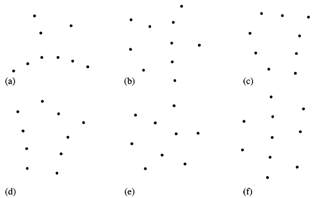
FIG. 4. Asymmetric relative equilibria of N identical point vortices, N=9,10,11 , determined by the method of “ghost” vortices, Eqs. (49). From an analytical point of view these configurations remain a mystery.
