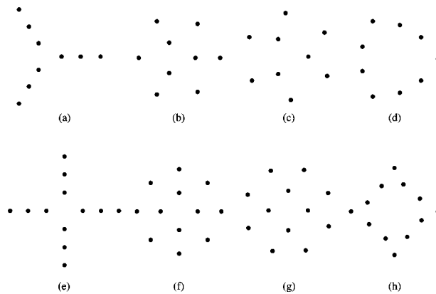
FIG. 2. Examples of relative equilibria of N identical point vortices that are understood analytically: [(a)–(d)] N=9 ; [(e)–(h)] N=12 (cf. Ref. 5).
