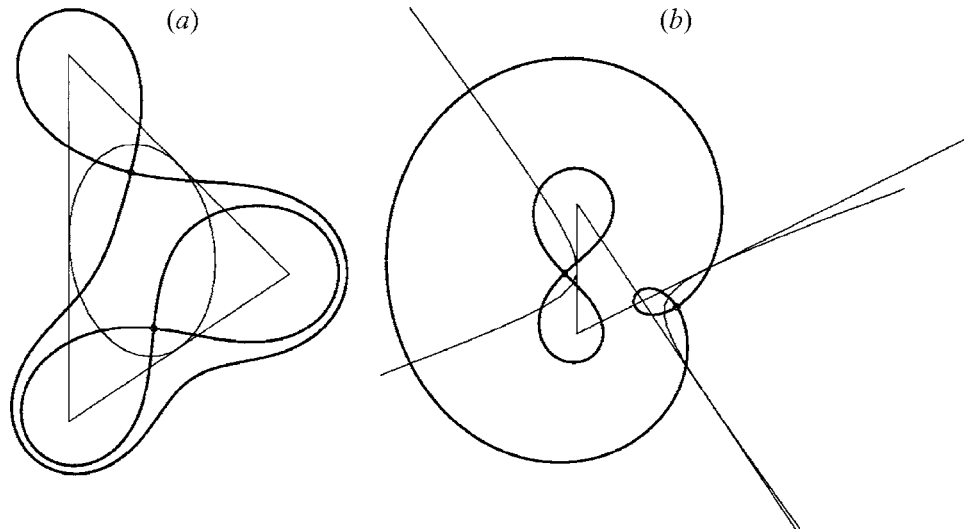
FIG. 5. Stagnation points for three-vortex flow as foci of the Siebeck conic. (a) Identical vortices; (b) vortices with strength ratio 1:1:-1.
