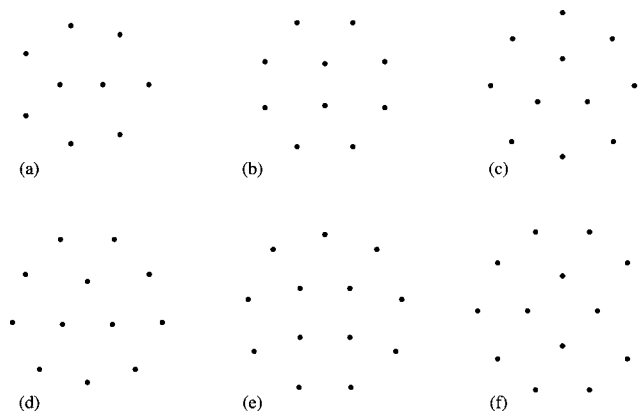
FIG. 3. Examples of relative equilibria of N identical point vortices with an axis of symmetry, N=9, \dots, 14 . These are determined to high precision numerically but poorly/not understood analytically. These configurations first appeared in the Los Alamos Catalog (Refs. 17 and 18).
