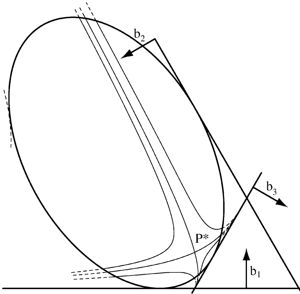
FIG. 1. An example of the trilinear coordinate representation of relative motion of three vortices of strengths 2, 1, and -4 (see the text for details).
