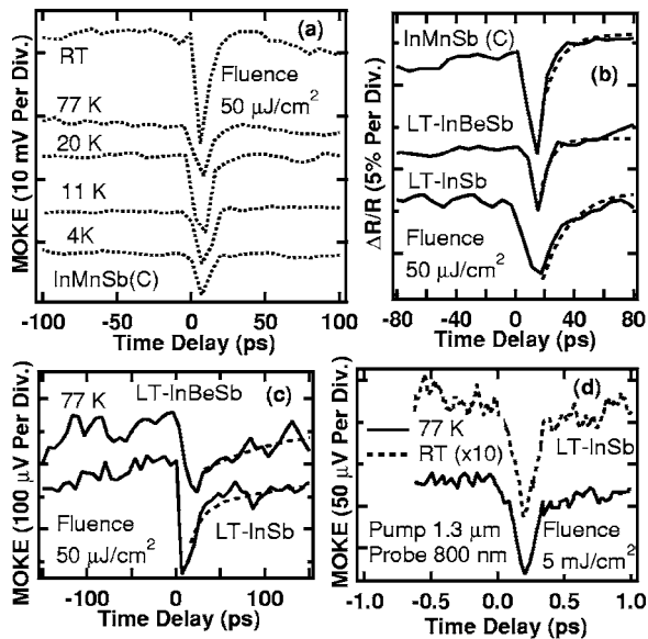
FIG. 3. (a) Photoinduced MOKE in InMnSb (sample C) at different temperatures. There is no significant difference between the relaxation above and below T_C . (b) Differential reflectivities of InMnSb, LT-InBeSb, and LT-InSb at 77 K (the dashed lines are exponential fits to the relaxations after the timing zero). (c) MOKE measurements on LT-InBeSb and LT-InSb using the degenerate pump/probe scheme at 77 K (the dashed lines are the sum of two exponential functions to the relaxations after the timing zero). (d) MOKE measurements on LT-InSb using the two-color scheme at room temperature and at 77 K.
