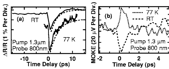
FIG. 1. Two-color measurements with pump fluence of \sim 5 \text{ mJ/cm}^2 of InMnSb (sample B). (a) Differential reflectivity (the dashed lines are exponential fits to the relaxations after the timing zero; for clarity the fits are displaced from the experimental traces). The differential reflectivity demonstrates an initial decrease lasting about 5 ps followed by an increase in reflectivity which shows a slow decay to its original value in the negative time delay. (b) MOKE at 77 K and room temperature. For clarity MOKE traces are plotted for two different circular polarizations of the pump.
