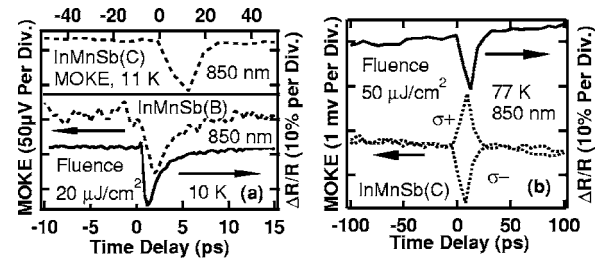
FIG. 2. (a) Differential reflectivity and MOKE of InMnSb (sample B) in the degenerate configuration at 10 K. In addition, for comparison, the MOKE signal of sample C is plotted at 11 K. (b) MOKE signal of InMnSb (sample C) for two different circularly polarized pump beams and differential reflectivity at 77 K.
