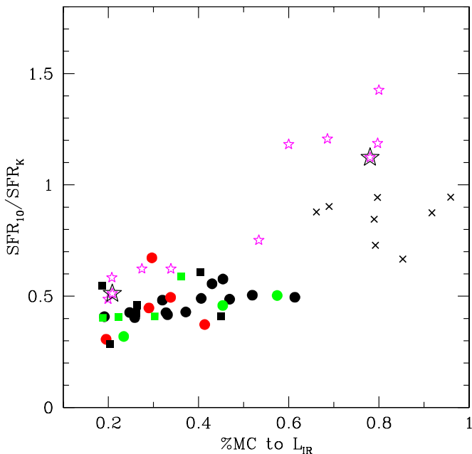
Figure 4. Correlation between the \text{SFR}_{10}/\text{SFR}_K ratio and the fractional contribution of MC emission to the total L_{\text{IR}} . Points are the same as in Figure 3. Here we show the eight local (U)LIRGs for which the fractional contributions of MC and cirrus emission have been already computed by us. Black stars are the two representative cases of R11 off-MS star-forming galaxies shown in Figure 5. We can see here that on average galaxies with higher \text{SFR}_{10}/\text{SFR}_K ratios have total IR luminosity mostly contributed by MC emission with all of our (U)LIRGs lying on the lower relation. Of course the scatter we see in this figure as well as in Figure 3 is due to the wide range of ages of stellar populations.
