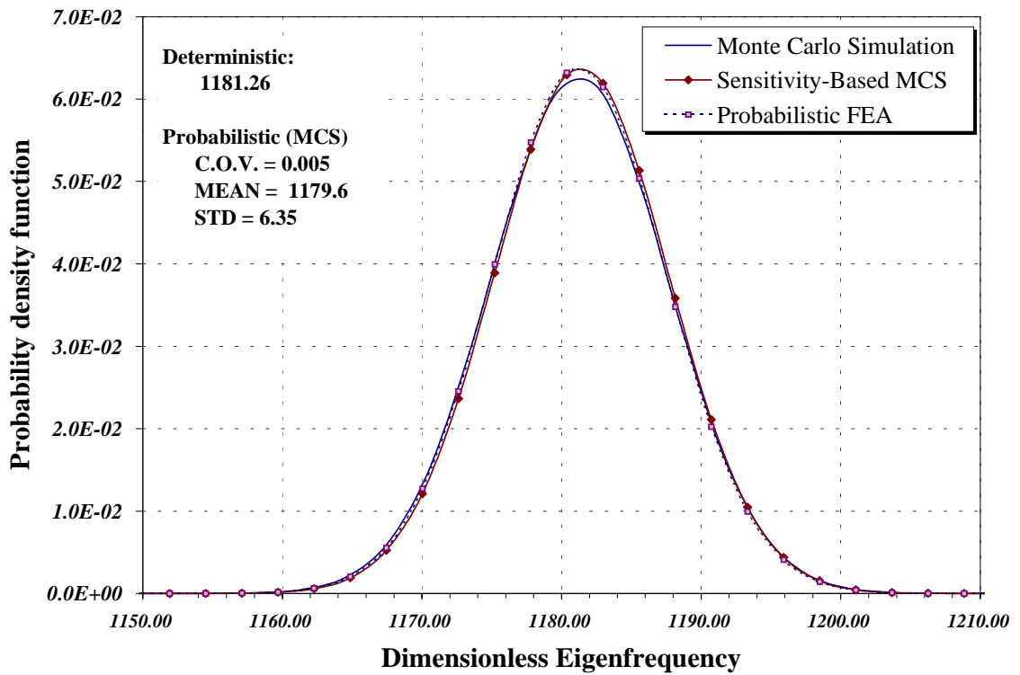
Figure 6.22: Probability density function of the dimensionless eigenfrequency, \tilde{\lambda} , for a simply-supported laminated beam ( [0^\circ/90^\circ/90^\circ/0^\circ] ) with uncertain ply orientations.
