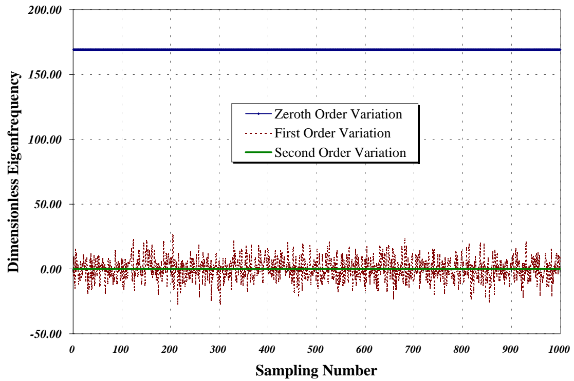
Figure 6.11: Effect of the order of the sensitivity derivatives on the dimensionless eigenfrequency, \tilde{\lambda} , for a cantilevered unidirectional laminated beam ( 0^\circ ) with uncertain Young's modulus in the x -direction.
