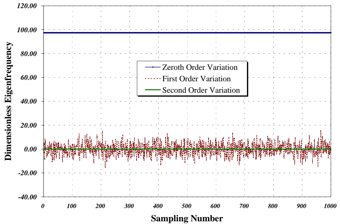
Figure 6.7: Effect of the order of the sensitivity derivatives on the dimensionless eigenfrequency, \tilde{\lambda} , for a simply-supported isotropic beam with uncertain Young's modulus in the x -direction.
