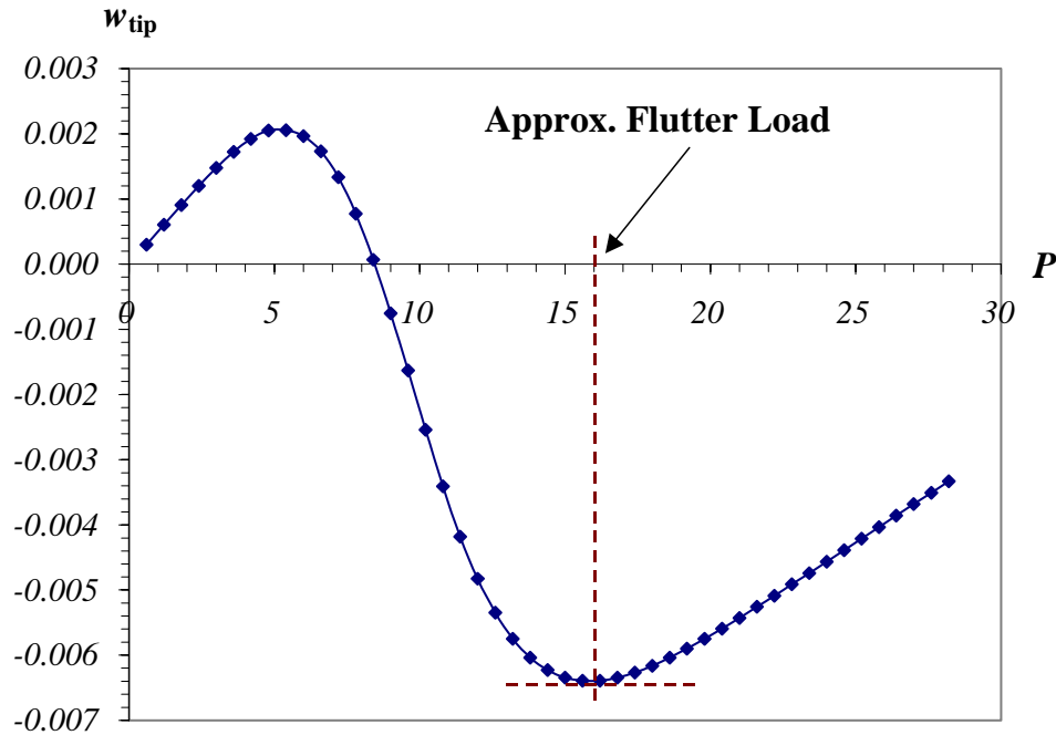
Figure 4.2: Approximating the flutter load in ABAQUS.
