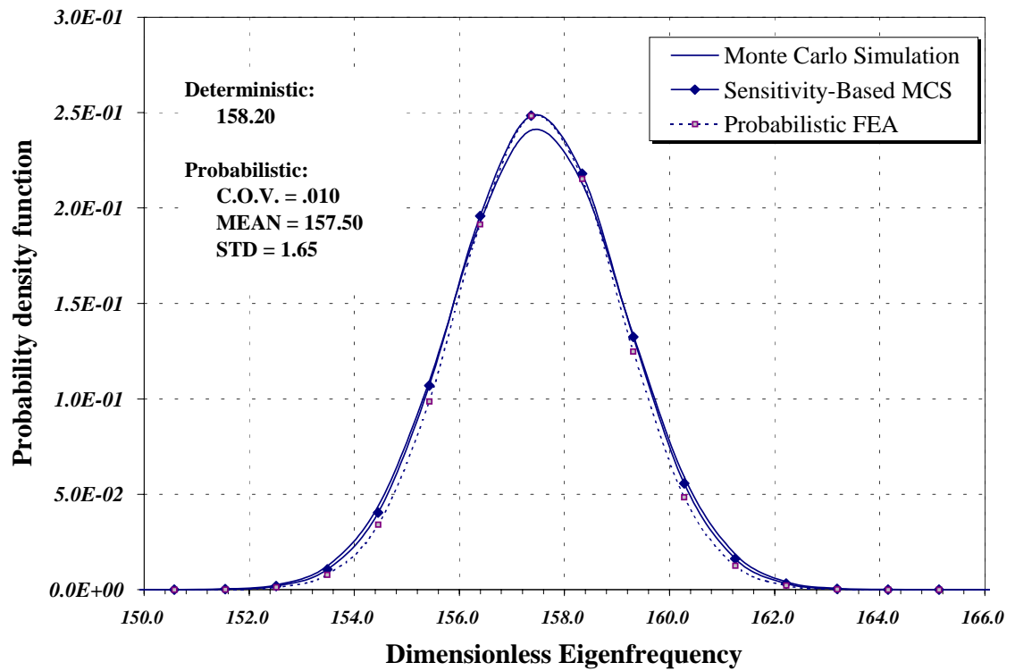
Figure 6.19: Probability density function of the dimensionless eigenfrequency, \tilde{\lambda} , for a cantilevered laminated beam ( [0^\circ/30^\circ/30^\circ/0^\circ] ) with uncertain ply orientations.
