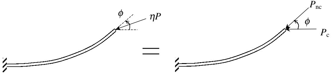
Figure 3.6: Subtangential Loading.
