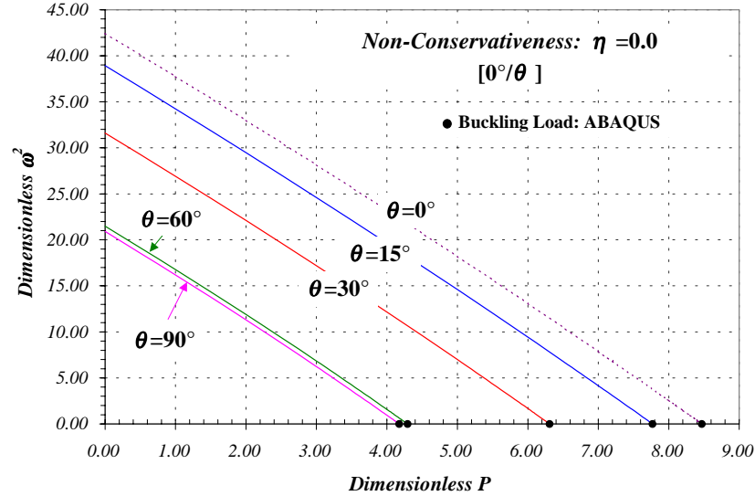
Figure 4.16: Characteristic curves for the fundamental buckling load \tilde{P} for unsymmetrical cantilevered laminated beams subject to a conservative loading.
