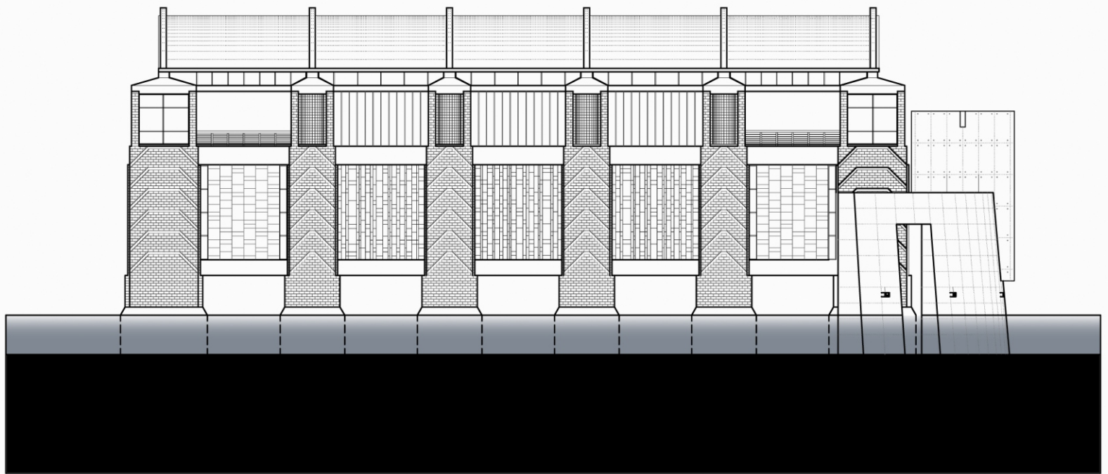
South Elevation
