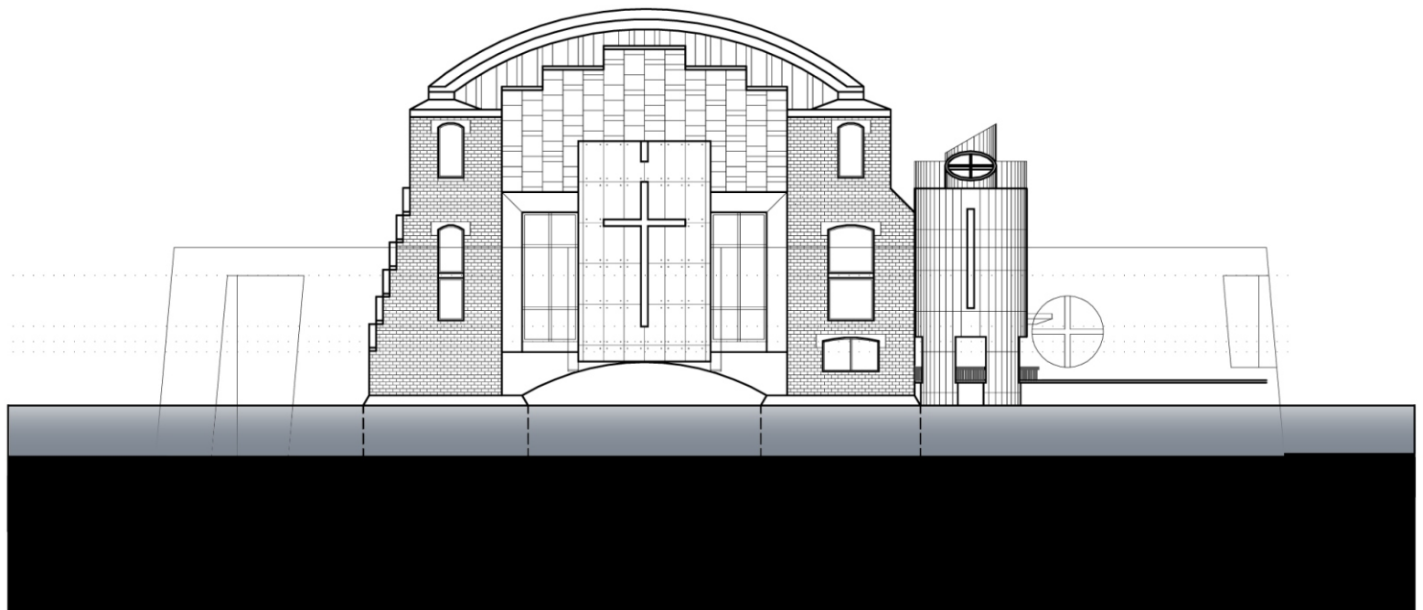
East Elevation-Inside Outer Walls
