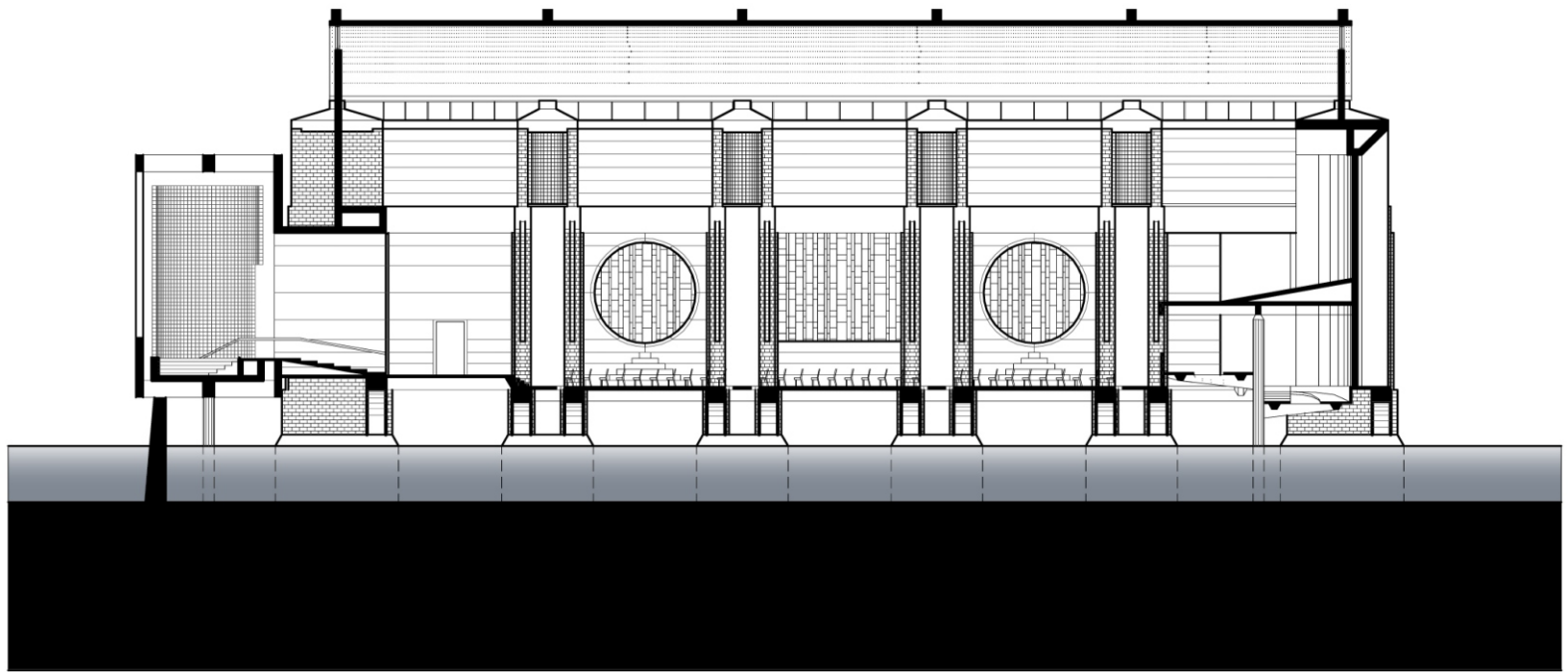
Transverse Section Looking South
