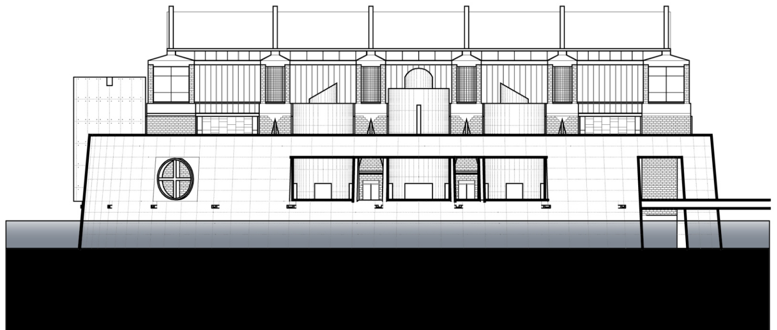
North Elevation
