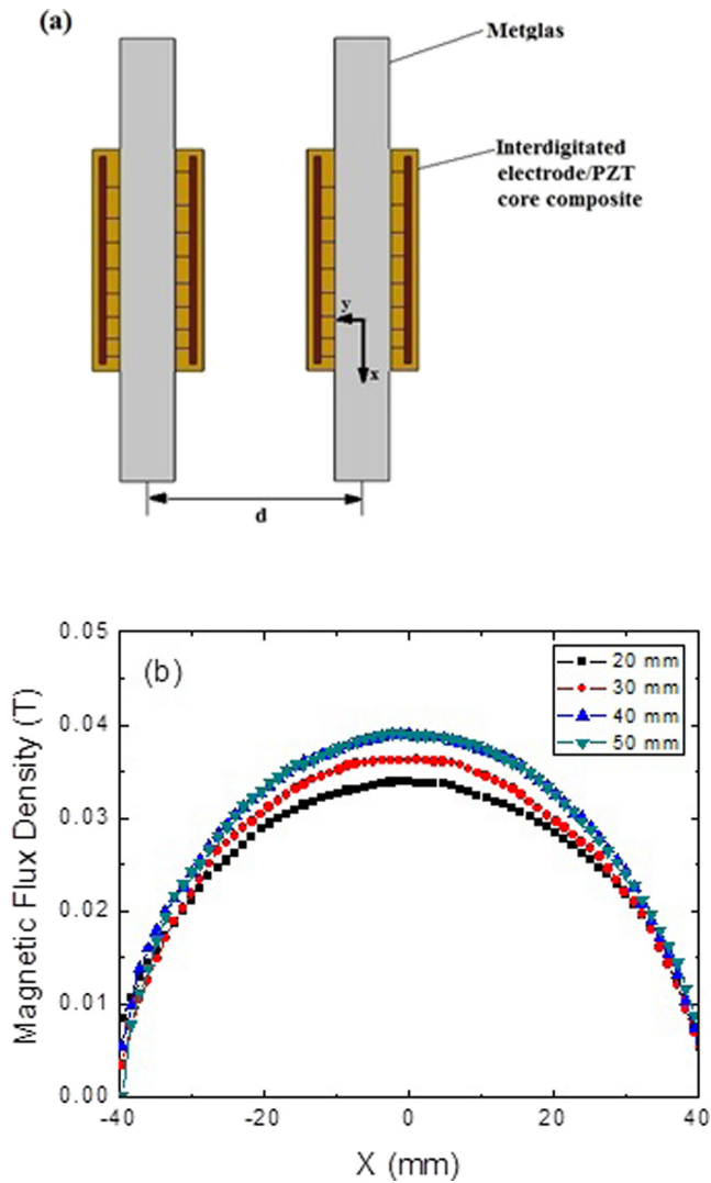
FIG. 1. (Color online) (a) Schematic representation of a pair of Metglas/PZT L-L mode ME laminates separated by a distance d . (b) Magnetic flux density of the Metglas foil along the x -axis (length direction) at y=0 , z=0 (the origin was at the center of the Metglas foil) when another identical foil was placed at various distances from it. The external magnetic field was 0.1 Oe.
