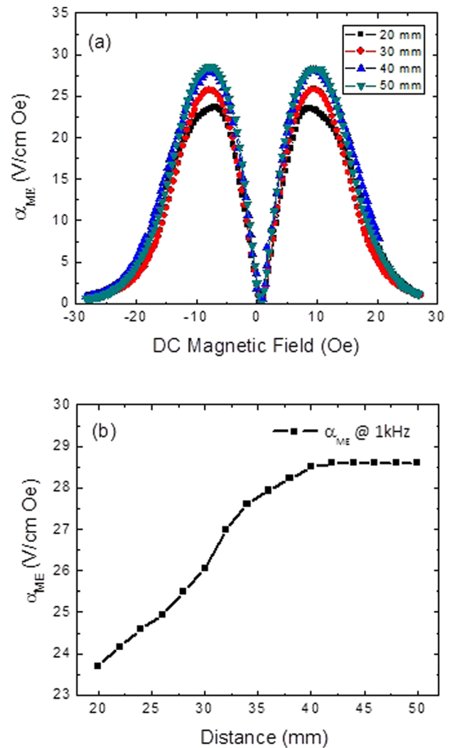
FIG. 2. (Color online) (a) The value of \alpha_{ME} as a function of dc bias field for one Metglas/PZT laminate when another one was placed at different distances from it. (b) The maximum value of \alpha_{ME} as a function of distance between two Metglas/PZT laminates. The data were measured at 1 kHz and H_{ac}=0.1 Oe.
