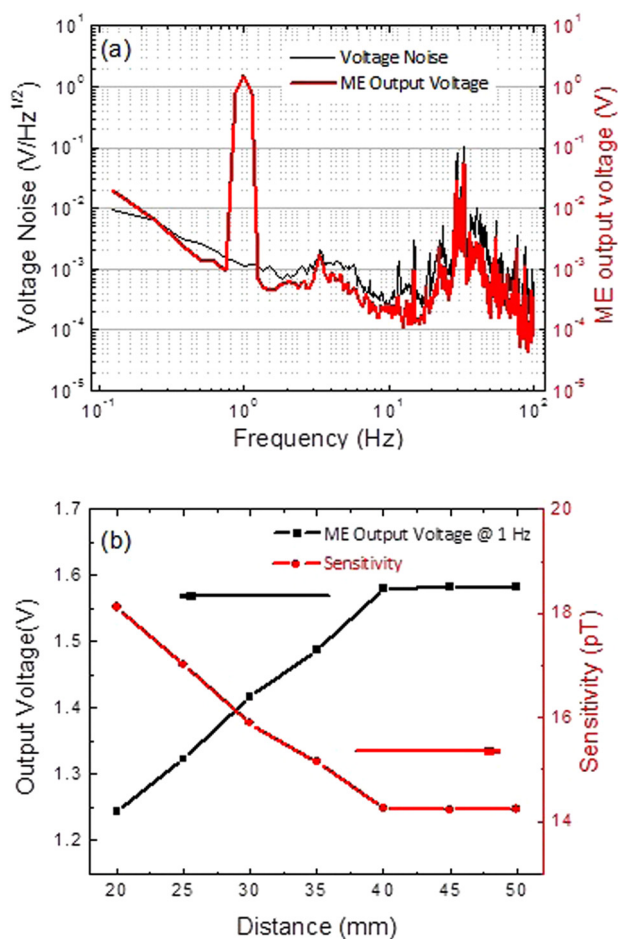
FIG. 3. (Color online) (a) ME output signal of the ME sensor unit and background voltage noise in the absence of intentional excitation. (b) The output signal and sensitivity of the sensor unit when the two laminates were placed at various distances. The incident AC magnetic field was 10 nT at 1 Hz.
