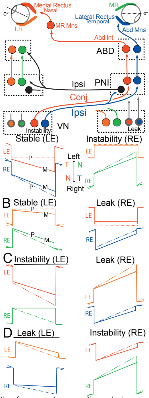
Figure 3-9: Schematic of neuronal connections during monocular time constant modifications. Similar to Figure 3-5; however this vignette is based on the the profile of activity within the left versus right PNI rather than vestibular nuclei.
