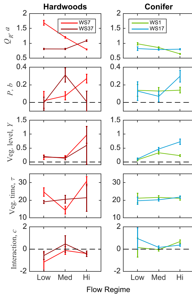
Figure 2. Values of regression model parameters to predict streamflow in equation (1) for four management treatments at annual low, medium, and high flows. The parameter a is the regression coefficient for Q_R , which is measured flow from reference watershed; b is the regression coefficient for P , which is the precipitation index; c is the regression coefficient for the interaction term; Y is the magnitude of change in flow due to management; and \tau is number of years to vegetation recovery. Maroon and red lines represent hardwood clear-cut watersheds, and blue and green lines represent conifer-converted watersheds. Parameters are considered significant contributors to the model if 95% confidence error bars do not cross the zero line (dashed).
