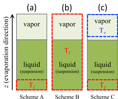
Figure 1. Schematics of three types of thermalizations during solvent evaporation: (a) Only a thin layer of the liquid solvent adjacent to the bottom wall is thermalized at T_l ; (b) All liquid and vapor are thermalized at T_l ; (c) A thin layer of the liquid solvent adjacent to the bottom wall is thermalized at T_l whereas the vapor zone at some distance away from the equilibrium liquid–vapor interface is thermalized at T_v . We set T_l = 1.0\epsilon/k_B , and T_v can be higher or lower than T_l to create a thermal gradient.
