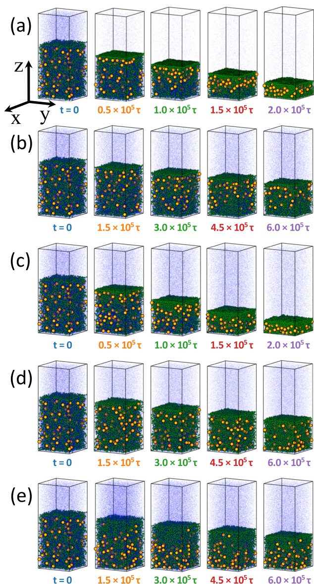
Figure 2. Snapshots during solvent evaporation for (a) T_{1.0\zeta_{30}}^1 , (b) T_{1.0\zeta_5}^1 , (c) T_{1.0\zeta_{30}}^1 , (d) T_{1.0\zeta_5}^1 , and (e) T_{1.0}^1 T_{1.2\zeta_5}^v . The elapsed time since the initiation of evaporation at t = 0 is listed under each snapshot. Temperature and density profiles of the five systems are shown in Figure 3. Color code: SNPs (green), LNPs (orange), and solvent (blue). Only 5% of the solvent beads are visualized to improve clarity.
