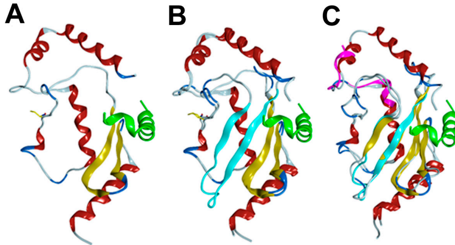
Figure 4. Homology models of RAD6B \Delta exon4 and RAD6Bintron5ins. (A) Model of RAD6B \Delta exon4. The catalytic cysteine residue is shown as a yellow line. RAD18 is shown in green. (B) Overlay of RAD6B \Delta exon4 and wild-type RAD6B from PDB file 2YBF. Beta sheets 3 and 4 of the wild-type RAD6B are shown in light blue. RAD18 is shown in green. (C) Overlay of RAD6Bintron5ins with wild-type RAD6B from PDB file 2YBF. The insertion is shown in magenta.
