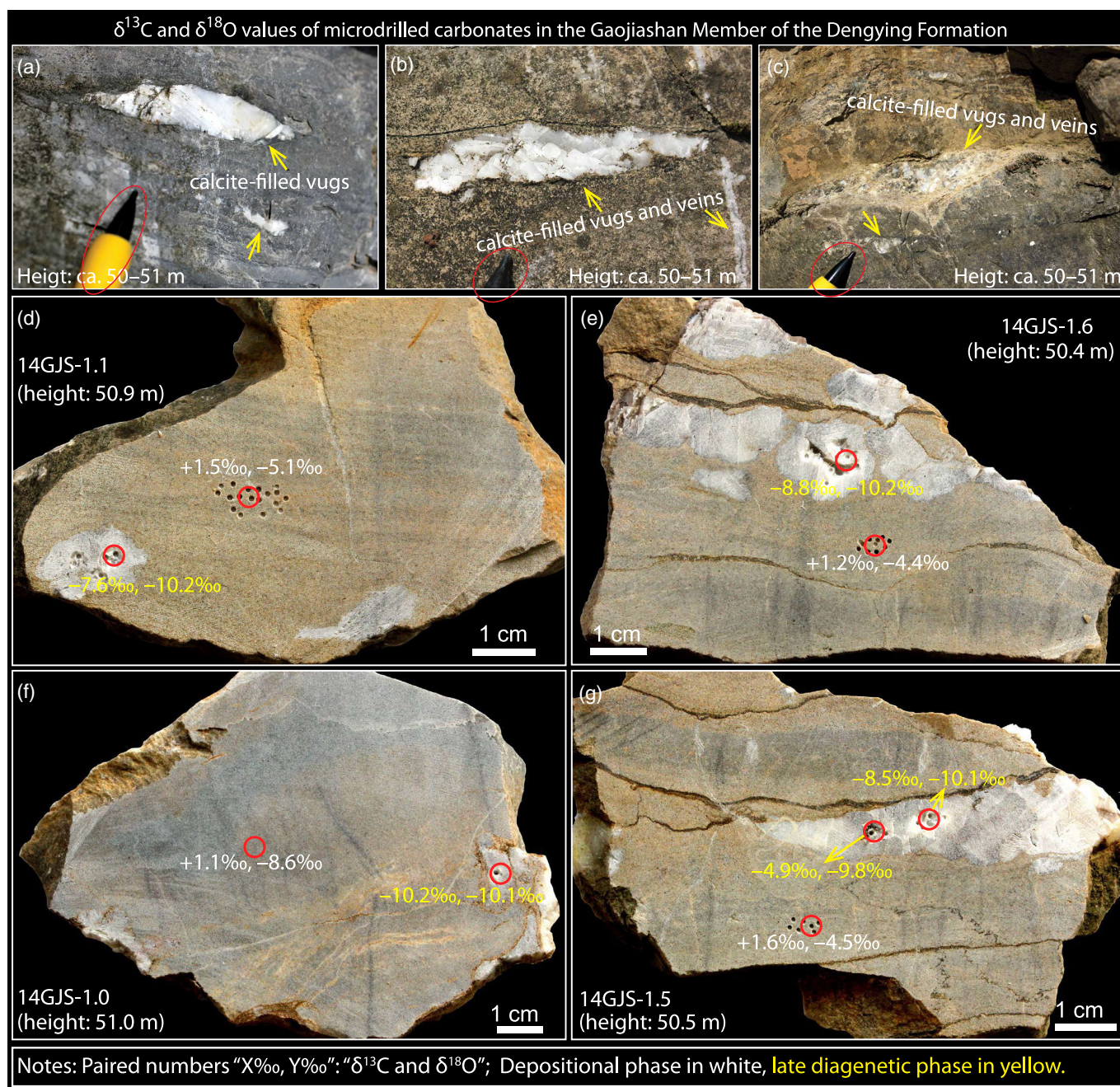
Fig. 11. (Colour online) Carbonate \delta^{13}\text{C} (left) and \delta^{18}\text{O} (right) values of micro-drilled samples from the Gaojiashan Member, Dengying Formation, at the Gaojiashan section. (a–c) Calcite-filled vugs and veins (arrows) at c. 50–51 m in Figure 13. Pencil for scale. (d–g) Carbonate \delta^{13}\text{C} (left) and \delta^{18}\text{O} (right) values of micro-drilled samples from the Gaojiashan Member. Note that the \delta^{13}\text{C} and \delta^{18}\text{O} values (in yellow) of the vug-filling calcite are consistently lower than those (in white) measured from the host carbonate rocks. Numbers in sample IDs represent distance (in metres) below the conglomerate/sandstone interval of the upper Gaojiashan Member. The stratigraphic height values in (d–g) represent the distance above the Gaojiashan/Algal Dolomite boundary.
