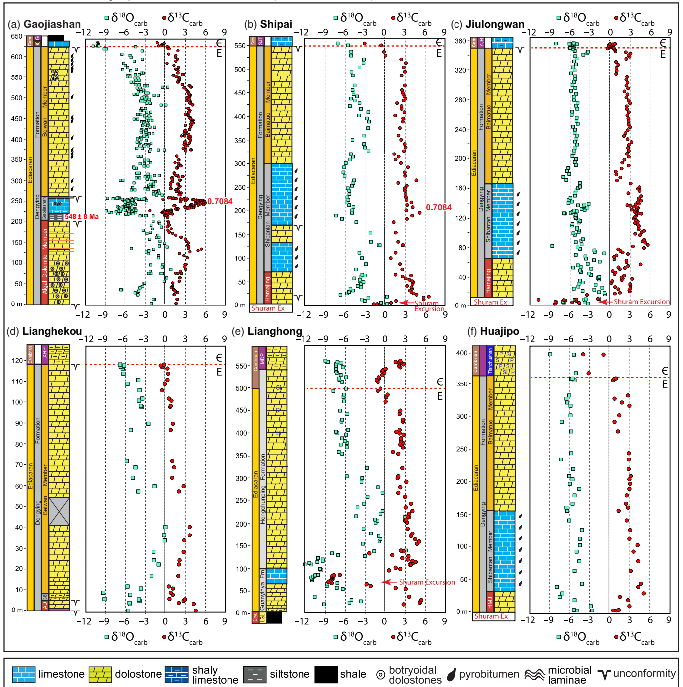
Fig. 14. (Colour online) Chemostratigraphic \delta^{13}\text{C}_{\text{carb}} (‰, VPDB) and \delta^{18}\text{O}_{\text{carb}} (‰, VPDB) profiles of multiple terminal Ediacaran sections in South China. Data sources: (a) Gaojiashan section (this study); (b) Shipai section (Jiang et al. 2007); (c) Jiulongwan section (Wang et al. 2014b); (d) Lianghekou section (Chen et al. 2015); (e) Lianghong section (Wang et al. 2012); (f) Huajipo section (Zhang et al. 2004). Source of the lowest ^{87}\text{Sr}/^{86}\text{Sr} values (0.7084): Gaojiashan section (this study) and Shipai section (Jiang et al. 2007). Abbreviations: AD – Algal Dolomite Member; Cam – Cambrian; \epsilon – Crogenian Period; E – Ediacaran; G – Guojiaba Formation; GJS – Gaojiashan Member; HMJ – Hamajing Member; K – Kuanchuanpu Formation; LGL – Lieguli Formation; MDP – Maidiping Formation; SJT – Shuijingtuo Formation; Shuram Ex – Shuram Excursion; XHP – Xihaoing Member; YJH – Yanjiahe Formation.
