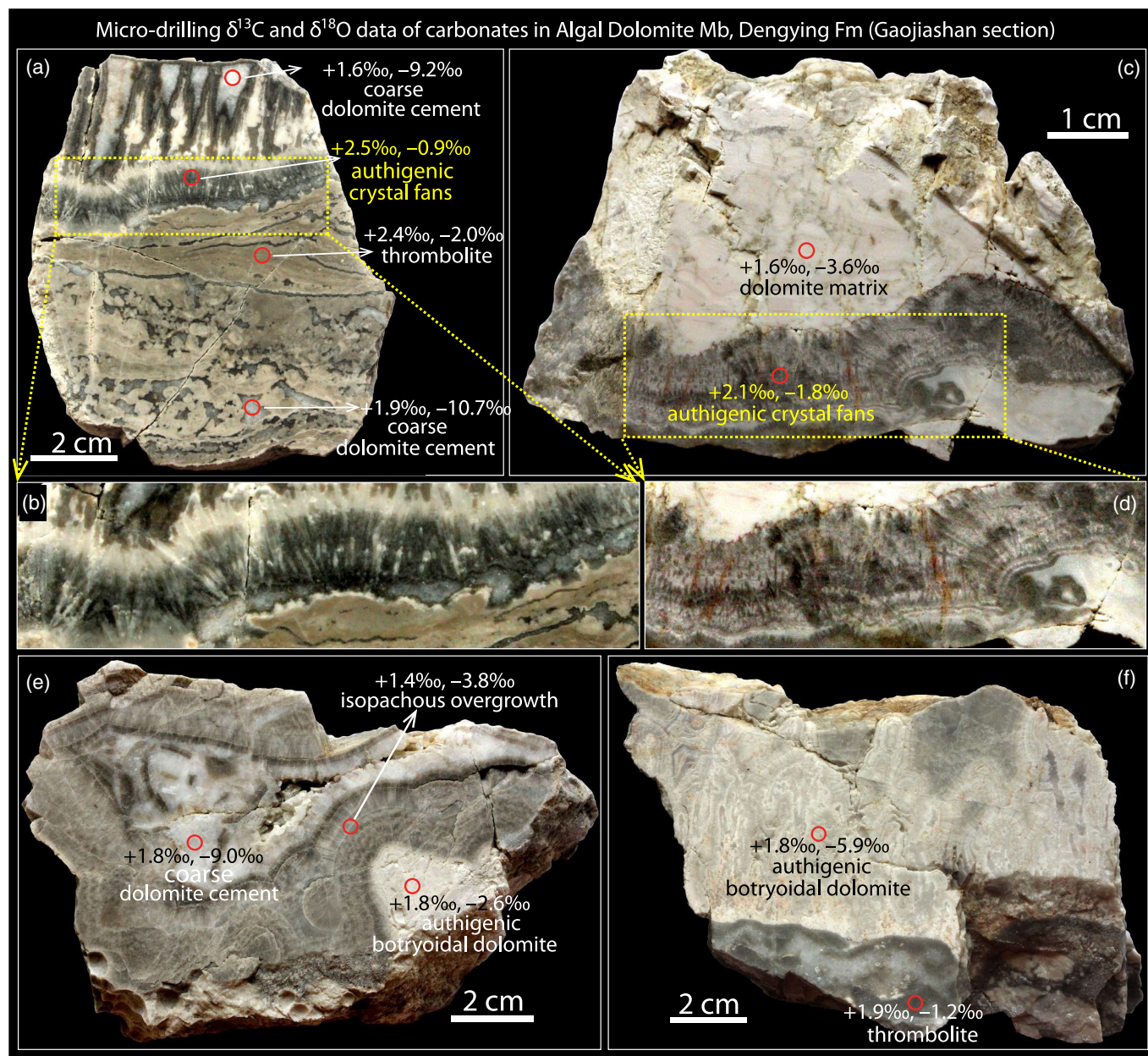
Fig. 10. (Colour online) Carbonate \delta^{13}\text{C} (left) and \delta^{18}\text{O} (right) values of micro-drilled samples from the Algal Dolomite Member, Dengying Formation, at the Gaojiashan section. (a–d) Freshly cut dolostone slabs showing authigenic crystal fans. (a) and (b) also illustrated in Figure 4a–f; (c) and (d) also illustrated in Figure 4g–i. Although all samples have been dolomitized, relic fabrics of aragonite are retained. (e, f) Freshly cut dolostone slabs showing thrombolite matrix, botryoidal dolomite, isopachous cements and late-stage dolomite cements. Note the relatively high \delta^{18}\text{O}_{\text{carb}} values in the aragonite crystal fans (-0.9‰ in (a) and -1.8‰ in (c)) and the relatively low \delta^{18}\text{O}_{\text{carb}} values in the late-stage coarse dolomite cements (-9.2‰ in (a) and -9.0‰ in (e)).
