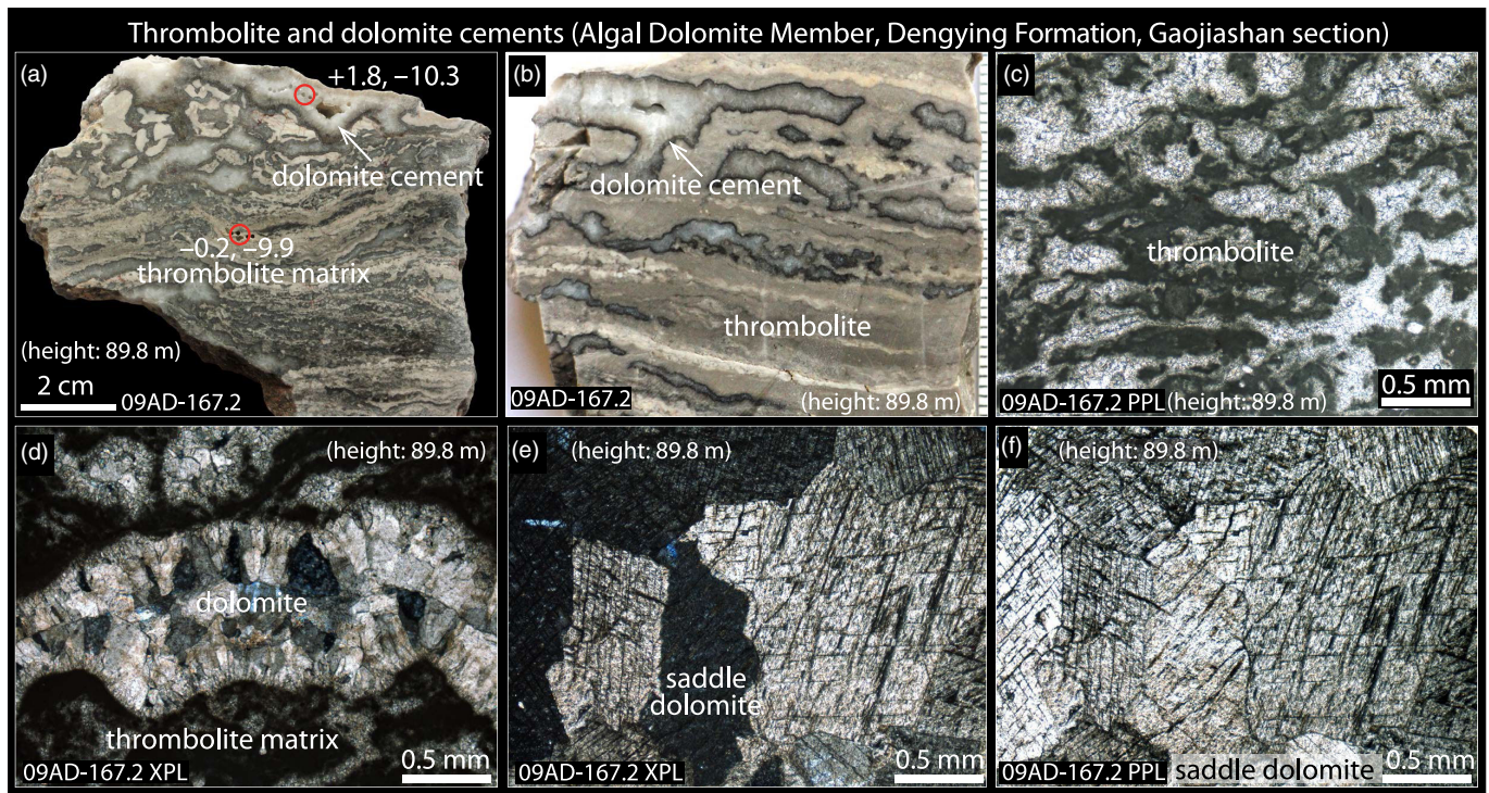
Fig. 5. (Colour online) Thrombolitic dolostone and void-filling hydrothermal dolomite cements in the Algal Dolomite Member, Dengying Formation, at the Gaojiashan section. Sample 09AD-167.2 from a stratigraphic height of 89.8 m in Figure 12. (a, b) Dolostone slabs showing thrombolitic dolomite matrix with vug-filling dolomite cements. Fabric-specific \delta^{13}\text{C} (left) and \delta^{18}\text{O} (right) data are provided in (a). Scale in (b) in millimetres. (c) A magnified view of the thrombolitic dolomite matrix under plane-polarized light. (d) A magnified view of coarse dolomite cements in the thrombolitic dolomite matrix under cross-polarized light. (e, f) Magnified views of hydrothermal saddle dolomites with two distinct sets of cleavages and sweeping extinction. PPL – plane polarized light; XPL – cross-polarized light.
