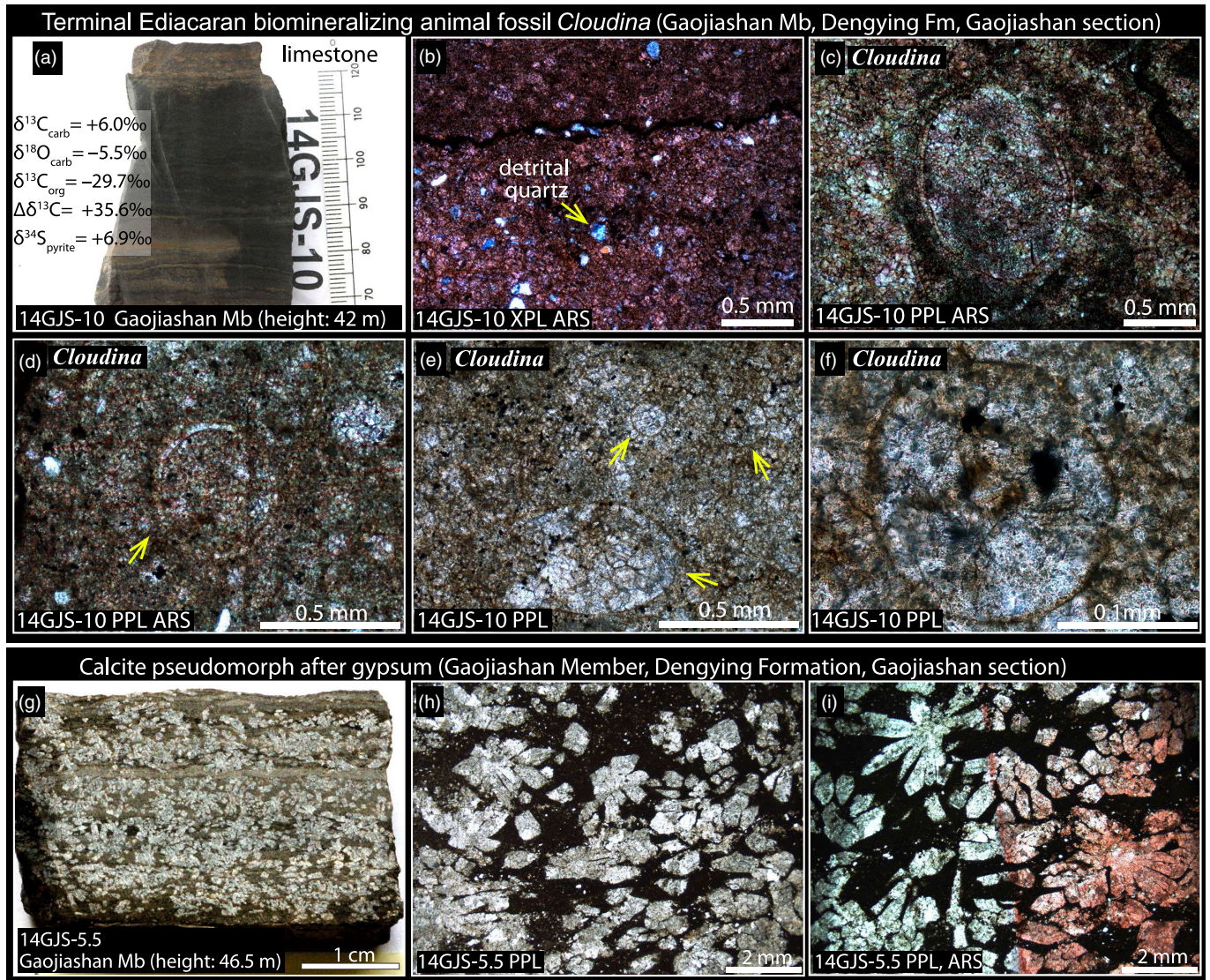
Fig. 7. (Colour online) Fossils and gypsum pseudomorphs in the Gaojiashan Member, Dengying Formation, at the Gaojiashan section. (a) Limestone slab 14GJS-10 (collected at 42 m in Fig. 13) with the terminal Ediacaran fossil Cloudina . (b) Thin-section of 14GJS-10 stained by Alizarin Red S, confirming its limestone lithology. Note abundant detrital quartz in this sample (arrow). (c–f) Transverse cross-sections of Cloudina (arrows) in thin-sections of the sample 14GJS-10. (g) Rock slab of sample 14GJS-5.5 (collected at 46.5 m in Fig. 13), showing calcite pseudomorphs after gypsum in the Gaojiashan Member. (h, i) Magnified views of the calcite pseudomorphs after gypsum rosettes. The right half of image (i) shows a red colour after being stained by Alizarin Red S, confirming the calcite composition of the pseudomorphs. PPL – plane polarized light; XPL – cross-polarized light; ARS – stained by Alizarin Red S.
