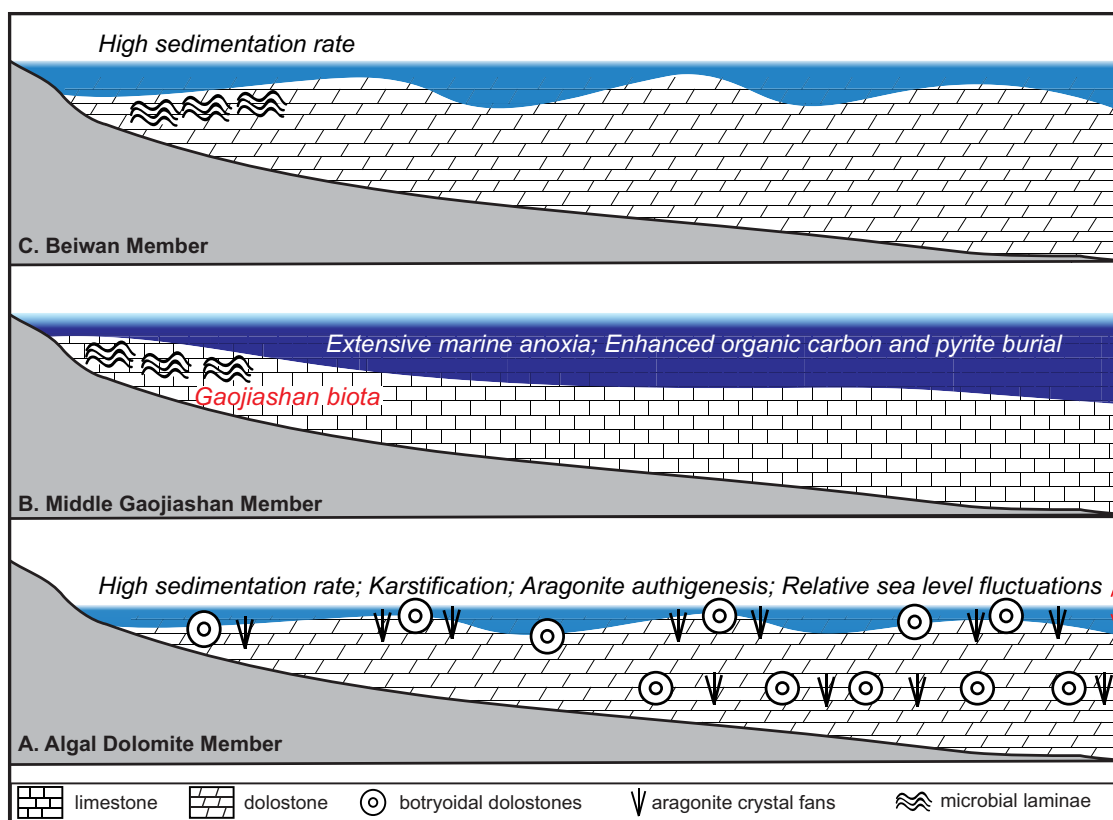
Fig. 9. (Colour online) A depositional model of the terminal Ediacaran Dengying Formation based on studies of the Gaojiashan section. See main text for a detailed discussion.
