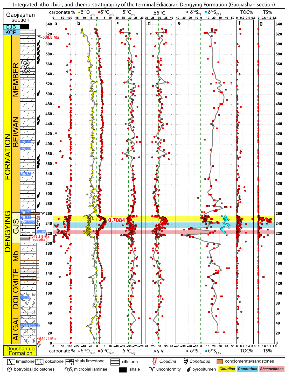
Fig. 12. (Colour online) Integrated litho-, bio- and chemostratigraphy of the terminal Ediacaran Dengying Formation at the Gaojiashan section. Geochemical profiles show (a) carbonate contents, (b) carbonate carbon isotopes ( \delta^{13}\text{C}_{\text{carb}} , ‰ VPDB), carbonate oxygen isotopes ( \delta^{18}\text{O}_{\text{carb}} , ‰ VPDB), (c) organic carbon isotopes ( \delta^{13}\text{C}_{\text{org}} , ‰ VPDB), (d) carbon isotope fractionations ( \Delta\delta^{13}\text{C}_{\text{carb-org}} ), (e) pyrite sulfur isotopes ( \delta^{34}\text{S}_{\text{TS}} , ‰ VCDT), carbonate-associated sulfate (CAS) sulfur isotopes ( \delta^{34}\text{S}_{\text{CAS}} , ‰ VCDT), (f) total organic carbon content (TOC) and (g) total sulfur content (TS, dominated by pyrite with trace amount of organic S) of acidified residues. The grey lines represent the five-point running average of the chemostratigraphic data. The lowest ^{87}\text{Sr}/^{86}\text{Sr} value (0.7084) measured from a limestone sample in the Gaojiashan Member is also marked in the \delta^{13}\text{C}_{\text{carb}} profile (at 246 m in stratigraphic height). The stratigraphic positions of some figures have been marked on the lithology column. Note that \delta^{13}\text{C}_{\text{carb}} and \delta^{18}\text{O}_{\text{carb}} data plotted here and in Figures 13, 14 only include micro-drilled samples of the least-altered micritic carbonate matrix, whereas \delta^{13}\text{C}_{\text{org}} and \delta^{34}\text{S}_{\text{TS}} data were measured from bulk samples after a complete acidification of carbonates. TS and TOC data are generally low owing to significant carbonate dilutions. Source of the detrital zircon age: Cui et al. (2016b). Abbreviations: GJS – Gaojiashan Member; KCP – Kuanchuanpu Formation; GJB – Guojiaba Formation. See online Supplementary Material Table S1 for complete data.
