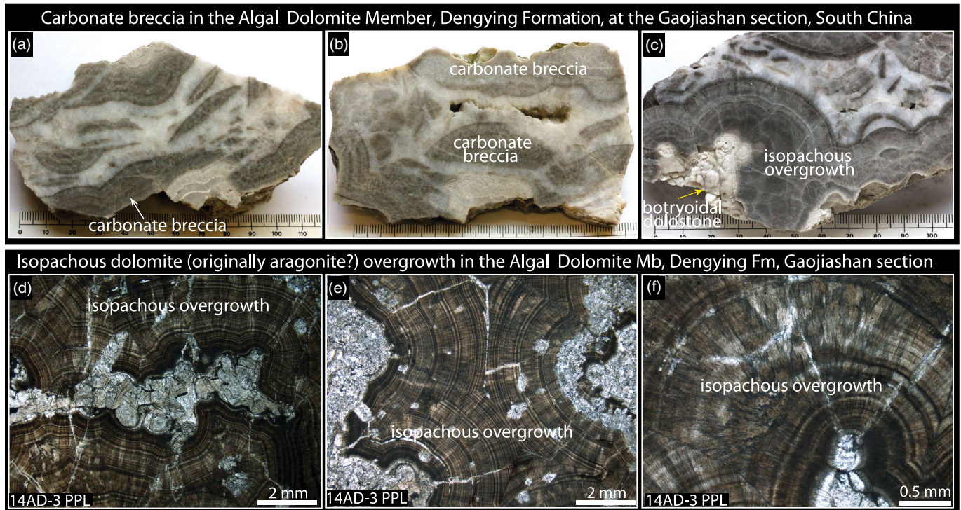
Fig. 3. (Colour online) Field samples and microscopic views of the carbonate breccia and isopachous overgrowth that are typical in the lower half of the Algal Dolomite Member of the Dengying Formation at the Gaojiashan section. (a–c) Karst breccia cemented by carbonates in the vugs between breccias. Scale in millimetres. (d–f) Petrographic images of sample 14AD-3, showing isopachous void-filling carbonate cements with concentric textures (brown colour) surrounding coarse dolomite sediments (white colour). PPL – plane polarized light.
