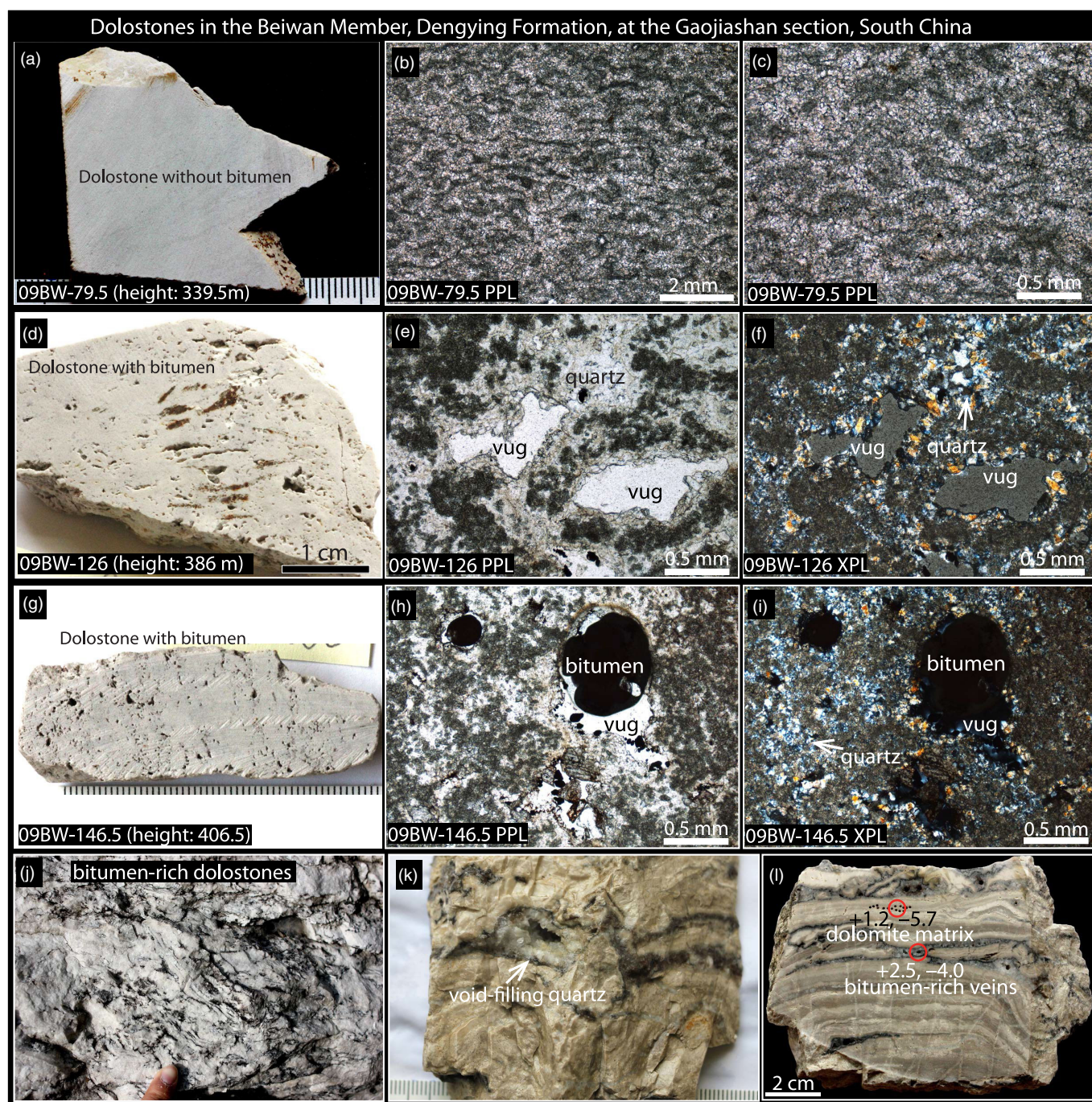
Fig. 8. (Colour online) Petrographic observations of dolostones in the Beiwai Member, Dengying Formation, at the Gaojiashan section. (a–c) Slab and petrographic photographs of sample 09BW-79.5 (collected at 339.5 m in Fig. 12) showing dolomitic texture with abundant algal fabrics (?). (d–f) Slab and petrographic photographs of sample 09BW-126 (collected at 386 m in Fig. 12) showing dolostone with vugs and quartz cements. (g–i) Slab and petrographic photographs of sample 09BW-146.5 (collected at 406.5 m in Fig. 12). Note the vugs with bitumen in (h) and (i), and the quartz cements (arrows) in (f) and (i) under cross-polarized light. (j) Outcrop photograph showing dolostones (white) with abundant bitumen (black). (k, l) Photographs of hand samples showing bitumen in dissolution vugs. Note the void-filling quartz (arrow) in (k). Micro-drilling geochemical \delta^{13}\text{C} (left) and \delta^{18}\text{O} (right) data are provided in (l). PPL – plane polarized light; XPL – cross-polarized light.
