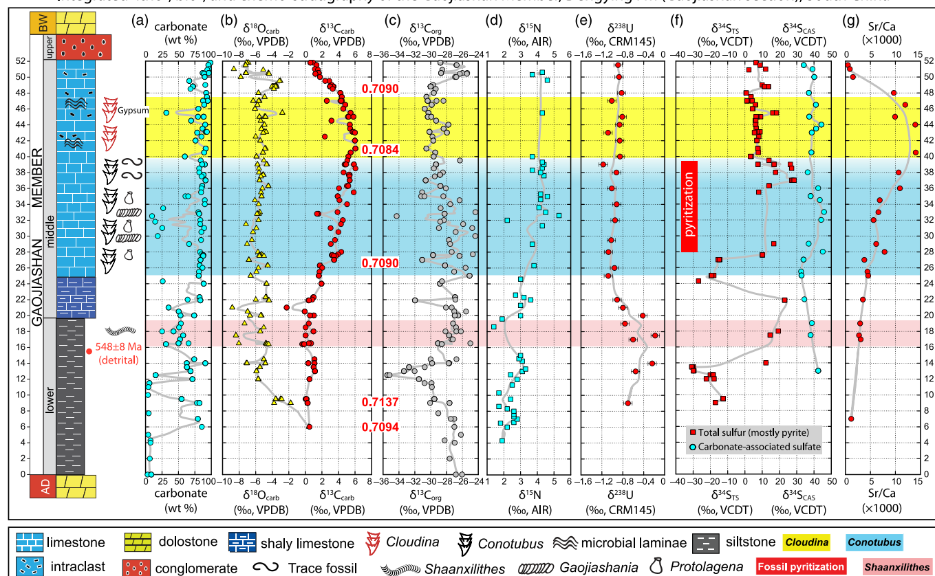
Fig. 13. (Colour online) Integrated litho-, bio- and chemostratigraphy of the Gaojiashan Member of the middle Dengying Formation at the Gaojiashan section. Geochemical profiles show (a) carbonate contents (wt %), (b) carbonate carbon isotopes ( \delta^{13}\text{C}_{\text{carb}} , ‰ VPDB), carbonate oxygen isotopes ( \delta^{18}\text{O}_{\text{carb}} , ‰ VPDB), (c) organic carbon isotopes ( \delta^{13}\text{C}_{\text{org}} , ‰ VPDB), (d) nitrogen isotopes ( \delta^{15}\text{N} , ‰ AIR), (e) uranium isotopes ( \delta^{238}\text{U} , ‰ CRM145), (f) sulfur isotopes ( \delta^{34}\text{S}_{\text{TS}} , ‰ VCDT) of total sulfur (TS, dominated by pyrite with trace amount of organic S) after a complete acidification of carbonates, carbonate-associated sulfate (CAS) sulfur isotopes ( \delta^{34}\text{S}_{\text{CAS}} , ‰ VCDT), and (g) Sr and Ca concentration (in ppm) ratios (Sr/Ca). Grey lines represent the three-point running average of the chemostratigraphic data. ^{87}\text{Sr}/^{86}\text{Sr} values measured from limestone beds or limestone nodules in the Gaojiashan Member are also marked along the \delta^{13}\text{C}_{\text{carb}} profile. Data sources: \delta^{13}\text{C} , \delta^{18}\text{O} , \delta^{34}\text{S} , Sr/Ca data (H. Cui, unpub. Ph.D. thesis, Univ. Maryland, 2015; Cui et al. 2016b), ^{87}\text{Sr}/^{86}\text{Sr} values (this study), \delta^{15}\text{N} data (A. Gampner, unpub. Ph.D. dissertation, Freie Universität Berlin, 2014), \delta^{238}\text{U} data (Zhang et al. 2018). Modified from Cui et al. (2016b). AD – Algal Dolomite Member; BW – Beiwan Member.
