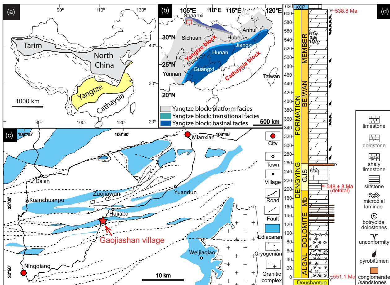
Fig. 1. (Colour online) Simplified tectonic map, geological map, litho- and chemostratigraphy of the terminal Ediacaran Dengying Formation at the Gaojiashan section, South China. (a) Tectonic framework of China, with the Yangtze Craton highlighted in yellow. (b) Ediacaran depositional environments on the Yangtze Craton (Jiang et al. 2007). Rectangle showing the location of the Ningqiang area in the northwestern margin of the Yangtze Platform. (c) Geological map of the Gaojiashan area in southern Shaanxi Province, modified after Cai et al. (2014). Red star indicates the studied section at Gaojiashan village, Niqiang county, Hanzhong city, southern Shaanxi Province. (d) Simplified stratigraphy of the Dengying Formation at Gaojiashan (Cui et al. 2016b). Sources of age data: Condon et al. (2005); Cui et al. (2016b); Linnemann et al. (2019). Abbreviations: GJS – Gaojiashan Member; KCP – Kuanchuanpu Formation.
