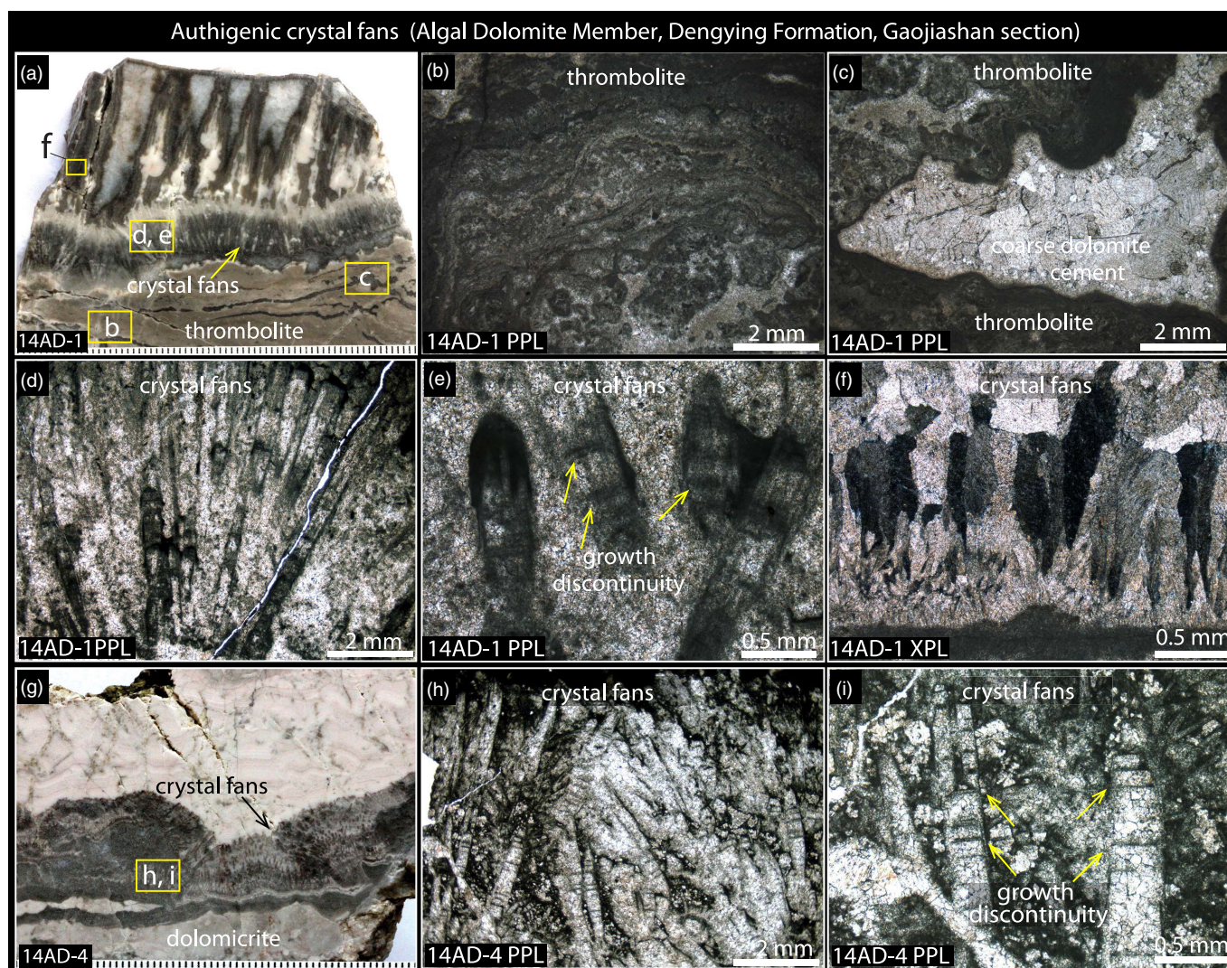
Fig. 4. (Colour online) Hand samples and microscopic views of the thrombolite and authigenic aragonite (now dolomite) crystal fans that are typical in the lower half of the Algal Dolomite Member of the Dengying Formation at the Gaojiashan section. (a) Sample slab 14AD-1, showing thrombolite sediments in the lower part and two generations of crystal fans in the middle and upper parts, respectively. Scale in millimetres. (b, c) Magnified views of thrombolitic texture in labelled rectangles in (a). Note the coarse dolomite cements within a large void in the thrombolitic dolomite matrix. (d, e) Authigenic crystal fans in labelled rectangles in (a). Note the crystals with growth discontinuities (arrows). Although the entire rocks have been dolomitized, the relic fabrics of the original aragonite crystals are retained. (f) Divergent fabrics of dolomite crystals with sweeping extinction under cross-polarized light in labelled rectangles in (a). (g) Dolostone slab 14AD-4 with crystal fans growing above dolomitic sediments. Scale in millimetres. (h, i) Magnified views of crystal fans in labelled rectangles in (g), showing growth discontinuities (arrows in (i)) within the aragonite crystals. PPL – plane polarized light; XPL – cross-polarized light.
