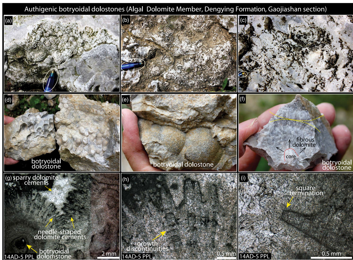
Fig. 2. (Colour online) Field and microscopic views of the authigenic botryoidal dolostones that are typical in the lower half of the Algal Dolomite Member of the Dengying Formation at the Gaojiashan section. (a–c) Outcrops showing distinct botryoidal textures with concentric lamina. Pen for scale. (d, e) Hand samples showing the distinct botryoidal texture. Note the part and counterpart in (d). (f) Fresh fracture surface showing radial fabrics diverging from the core. (g) Microscopic images of the authigenic botryoidal dolomite showing needle-shaped crystals with growth discontinuities and square terminations. Note the needle-shaped crystals as the first-stage cements and the sparry dolomite as the second-stage cements. (h, i) Magnified views of the needle-shaped crystals with discontinuities and square terminations, indicating original aragonite mineralogy. PPL – plane polarized light.
