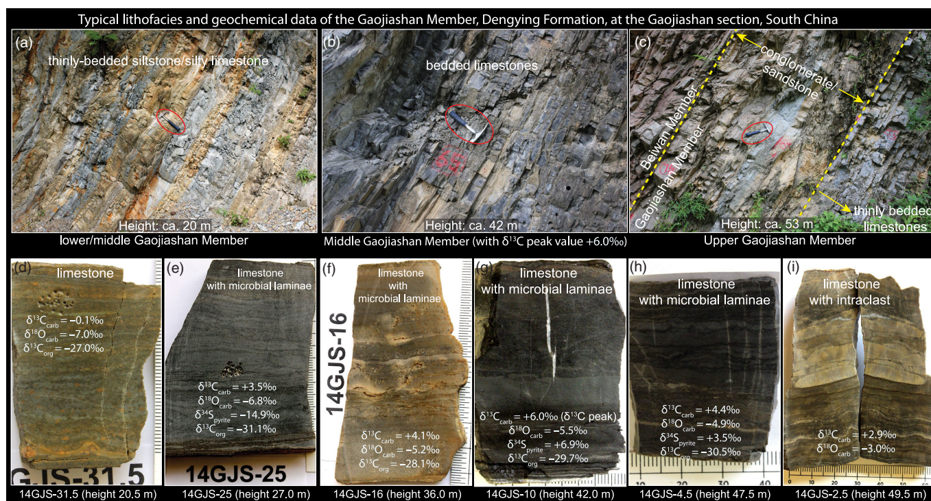
Fig. 6. (Colour online) Typical lithofacies and geochemical data of the Gaojiashan Member, Dengying Formation, at the Gaojiashan section, South China. Stratigraphic height numbers represent the distance above the Algal Dolomite/Gaojiashan boundary. (a) Thinly bedded siltstones and silty limestones in the lower/middle transition of the Gaojiashan Member. (b) Dark-coloured thin-bedded limestones in the middle Gaojiashan Member that records a \delta^{13}\text{C}_{\text{carb}} positive excursion of up to +6 ‰ (Cui et al. 2016b). (c) A conglomerate/sandstone interval in the upper Gaojiashan Member. Hammer for scale is 33 cm long. (d–i) Photographs of freshly cut slabs of samples from the Gaojiashan Member with microbial laminae and intraclasts. These slabs represent (d) greenish grey dolostone, (e–h) limestones with microbial laminae, and (i) intraclastic limestone. The numbers in the sample IDs represent distance (in metres) below the conglomerate interval in the upper Gaojiashan Member; for example, sample 14GJS-10 is 10 m below the conglomerate interval in the Gaojiashan Member. The \delta^{13}\text{C}_{\text{carb}} and \delta^{18}\text{O}_{\text{carb}} values of micro-drilled carbonate powders are marked on the slab. The \delta^{34}\text{S}_{\text{pyrite}} and \delta^{13}\text{C}_{\text{org}} values of each slab were analysed from bulk acidified residues.
