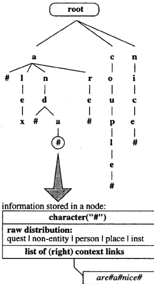
Figure 5: Cucerzan’s example of a prefix trie for “Alex and Anda are a nice couple” [13]
