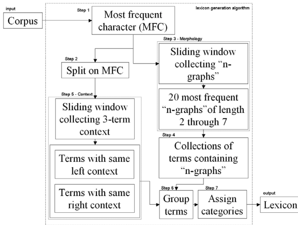
Figure 10: Lexicon Generation Algorithm
