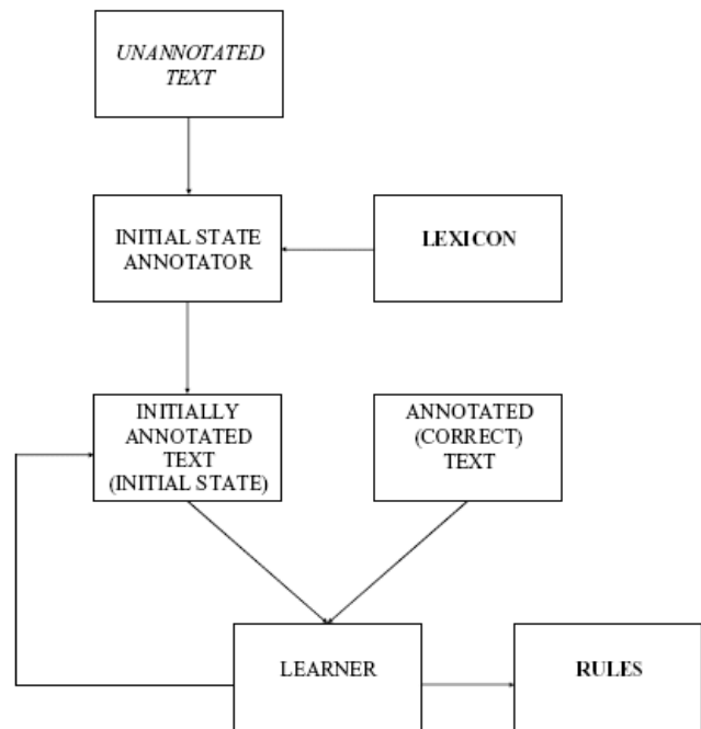
Figure 4: Brill's description of transformation-based rule learning [8].
