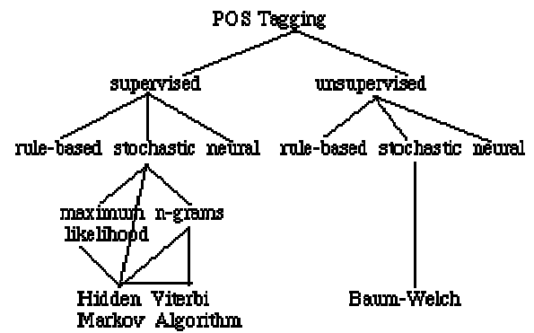
Figure 2: Approaches for POS Tagging [34]
