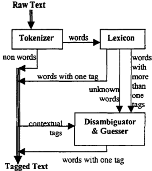
Figure 3: Traditional POS-Tagger Architecture [25]
