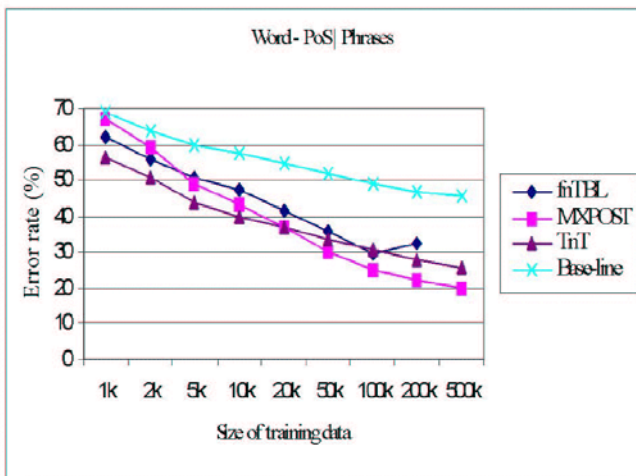
Figure 8: Comparing POS taggers using word-only to predict parts-of-speech [21]
