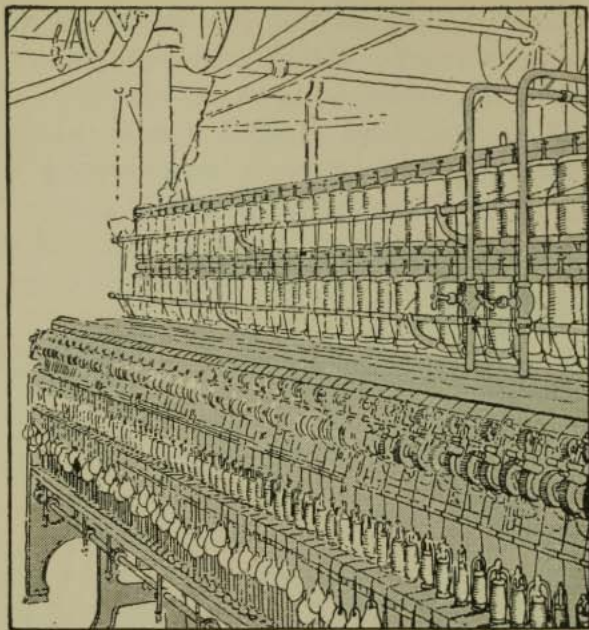
FIG. 179. — Flax spinning.
