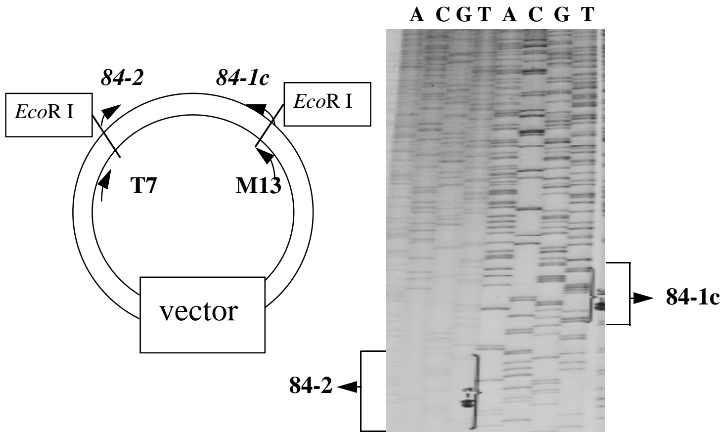
Figure 13. DNA sequencing of the PCR fragment for the DdRPA1 gene. 84-2 (sense) and 84-1c (antisense) were the degenerate primers for the touchdown PCR reaction. T7 and M13 reverse primers were the sequencing primers.
