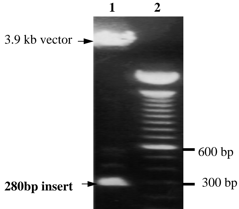
Figure 53. Restriction enzyme digestion of the cloned DdRPA2 PCR fragment. Lane 1: EcoR I digestion of cloned 35 kDa PCR fragment; lane 2: 100 bp DNA ladder standard.
