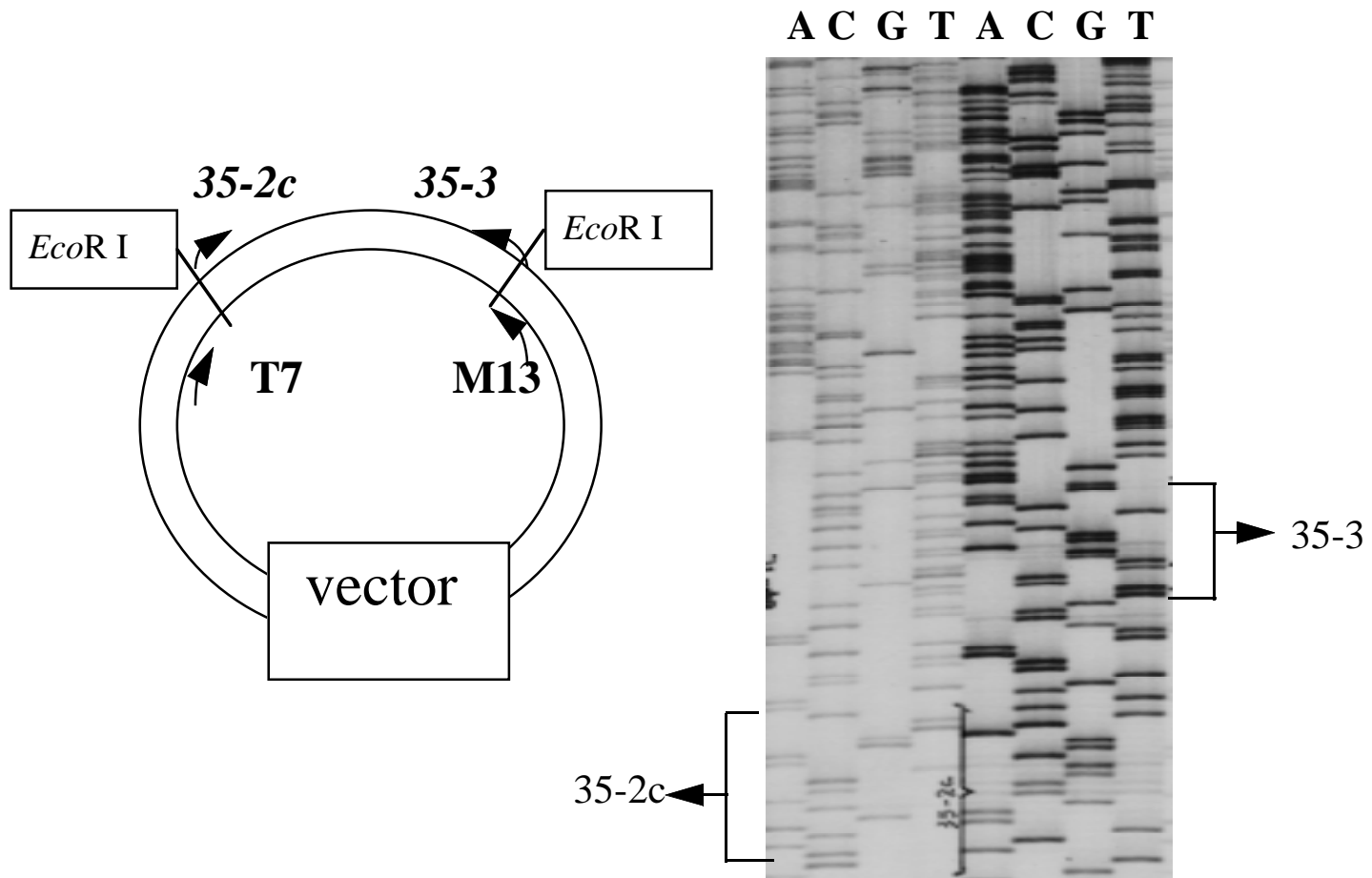
Figure 54. DNA sequencing of a PCR fragment for the DdRPA2 gene. 35-3 (sense) and 35-2c (antisense) were the degenerate primers for the PCR reaction. T7 and M13 reverse primer were the sequencing primers.
