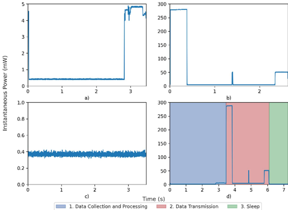
Figure 6. Instantaneous power dissipation a) for data collection and processing b) for data transmission c) during sleep d) total power dissipation of the WSN.
