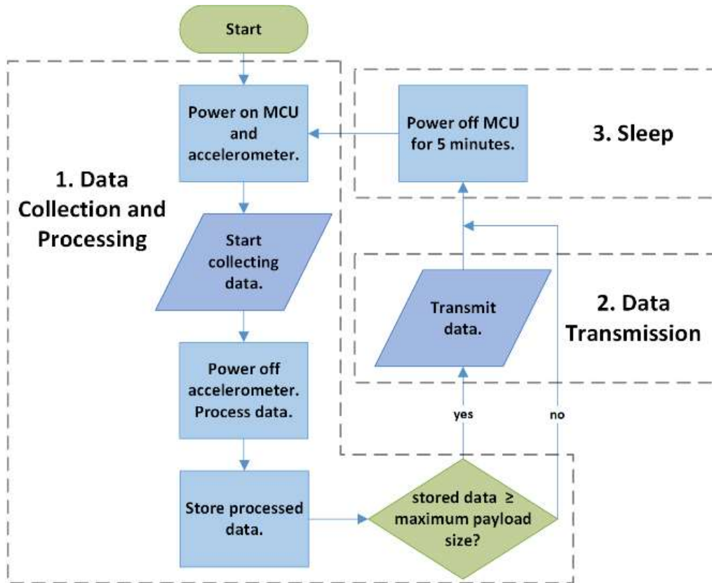
Figure 3. Flowchart of the WSN's operation.
