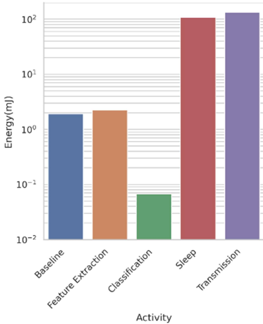
Figure 7. Energy consumed by the WSN performing various activities.
