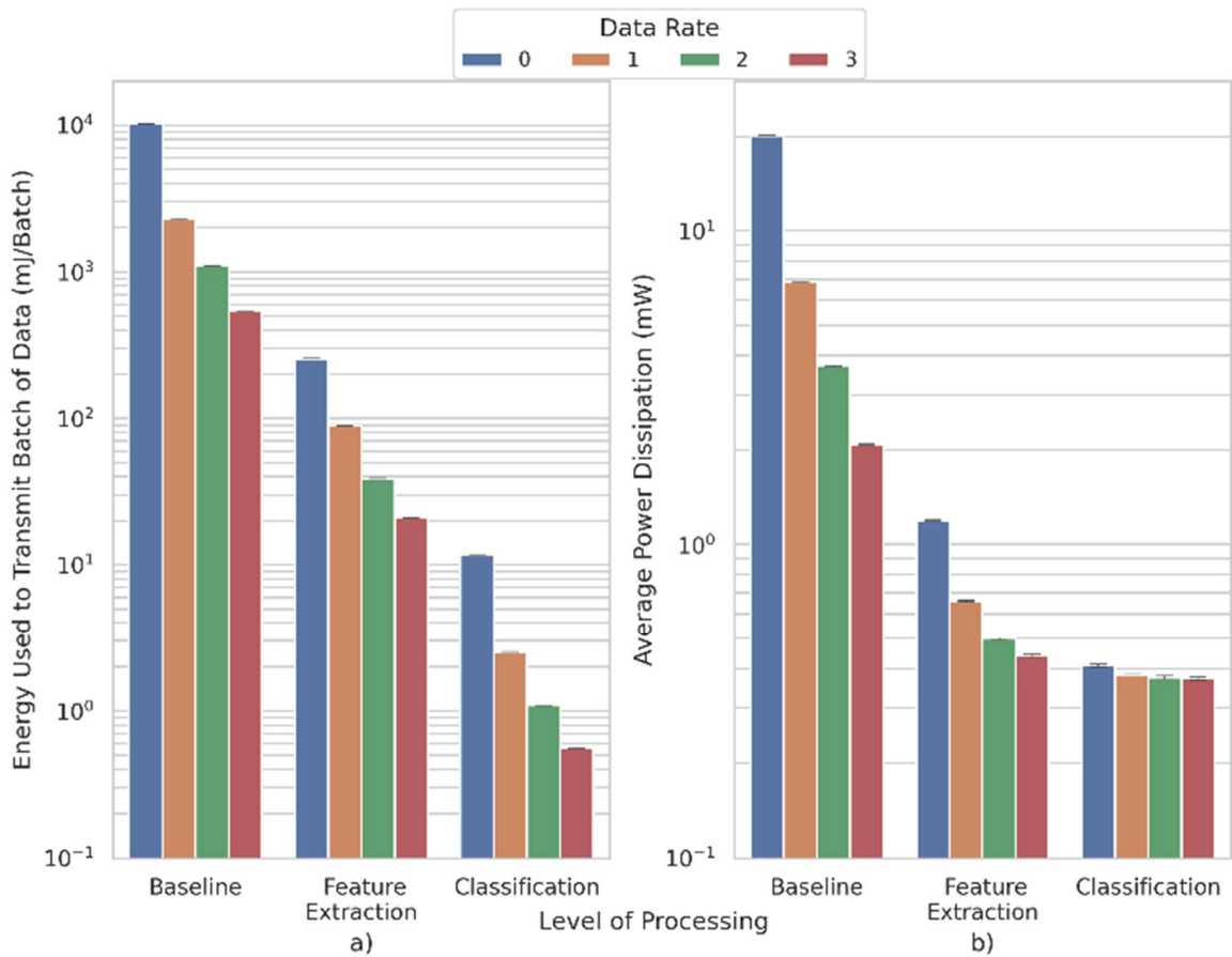
Figure 8. a) Energy used to transmit a batch of data processed to varying degrees. b) average power dissipation of the WSN.
