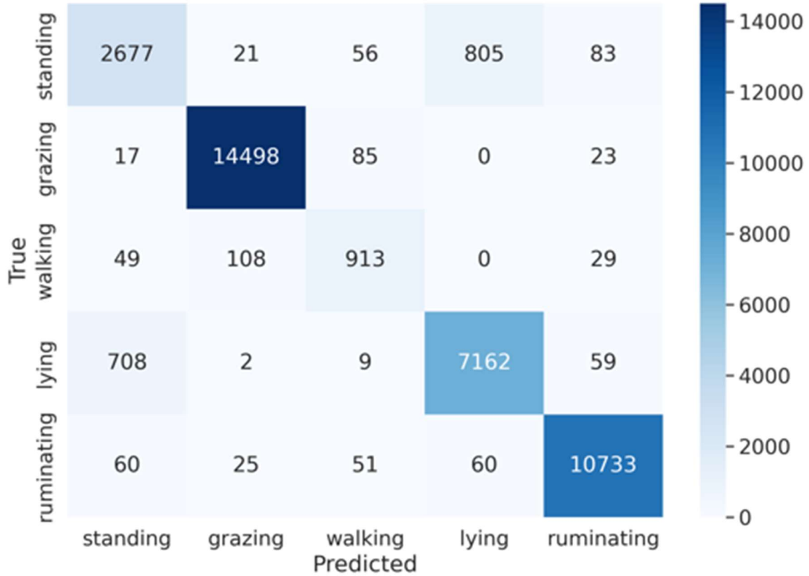
Figure 5. Confusion matrix of the decision tree model.
