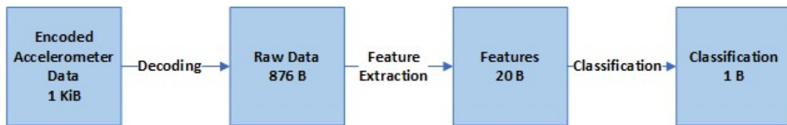
Figure 4. Pipeline to process the accelerometer data.
