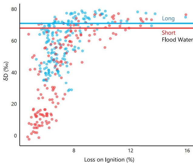
Figure 7. Concentration of deuterium in soil water from peds subjected to short- and long-duration artificial flooding by water spiked with deuterium to the indicated concentrations, as a function of organic matter estimated by mass loss on ignition (likely 4%–6% overestimated).
