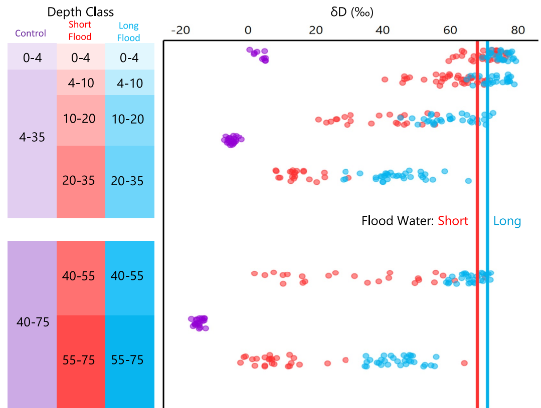
Figure 5. Concentration of deuterium in soil water from peds subjected to short- and long-duration artificial flooding by water spiked with deuterium to the indicated concentrations. Data were collected in depth classes and are presented with randomly jittered vertical positions for visibility.
