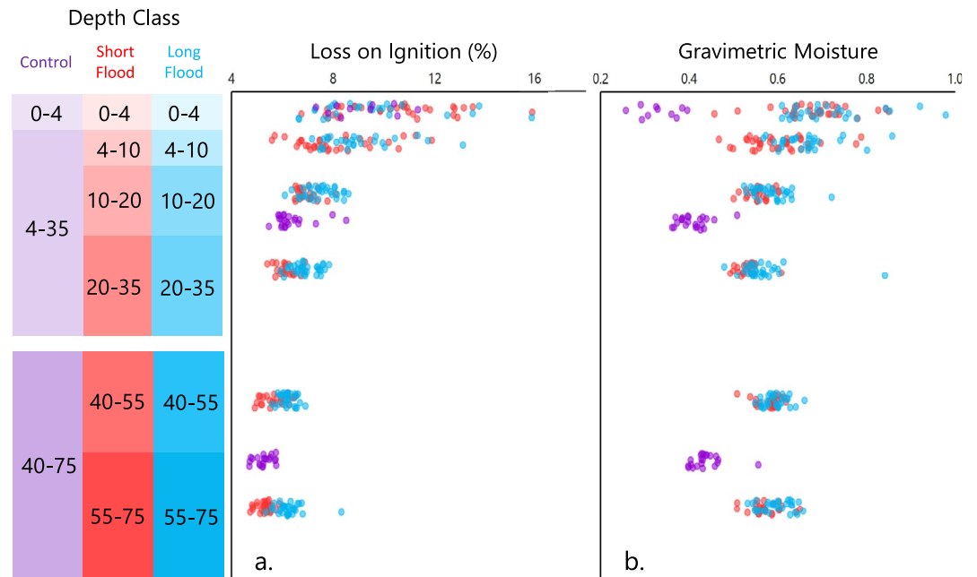
Figure 3. (a) Organic matter estimated by mass loss on ignition (likely 4%–6% overestimated) and (b) gravimetric moisture of control and artificially flooded soil pedes. Data were collected in depth classes and are presented with randomly jittered vertical positions for visibility. Differences in organic matter between short-flood and long-flood samples are coincidental.
