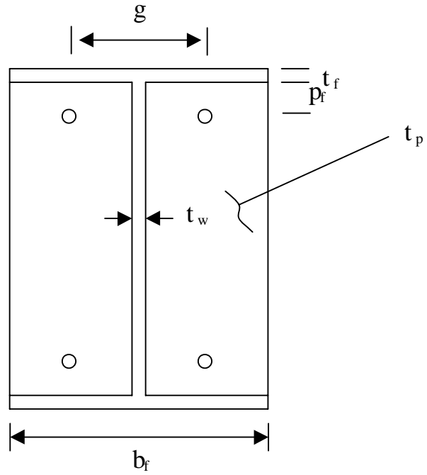
FIGURE 3-1. Flush validation specimen.
