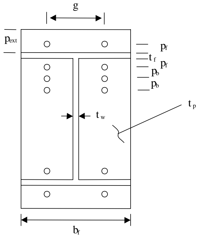
FIGURE 3-2. Multi-row-extended validation specimen.
