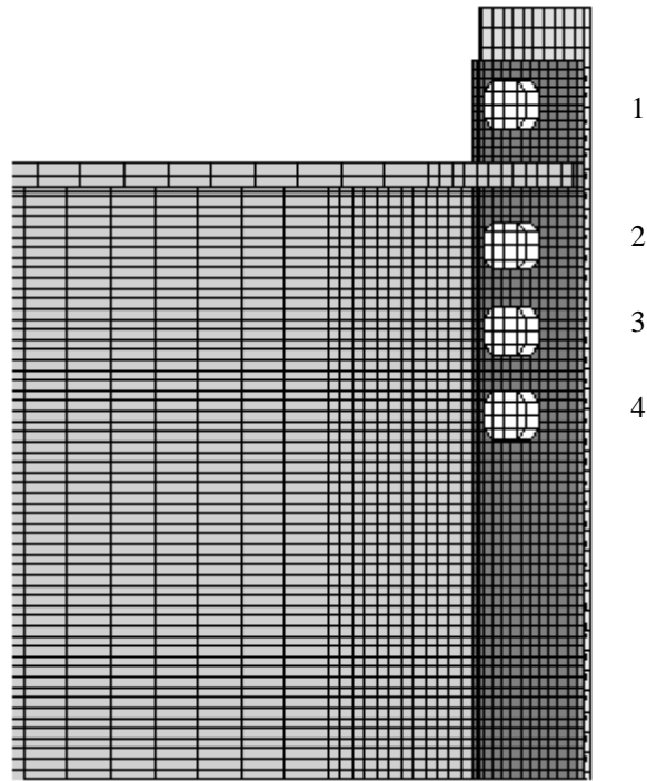
FIGURE 3-9. Finite element mesh and tension bolt numbering scheme for MRE-1/3-1 1/4-5/8-62 (deep beam to rigid column flange).
