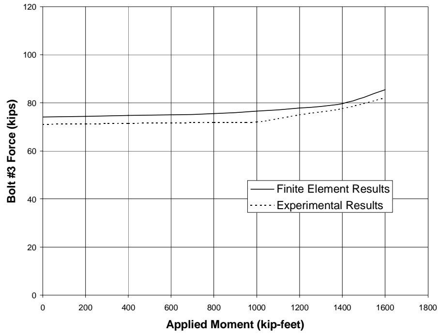
FIGURE 3-13. Bolt #3 force vs. applied moment for deep beam.
