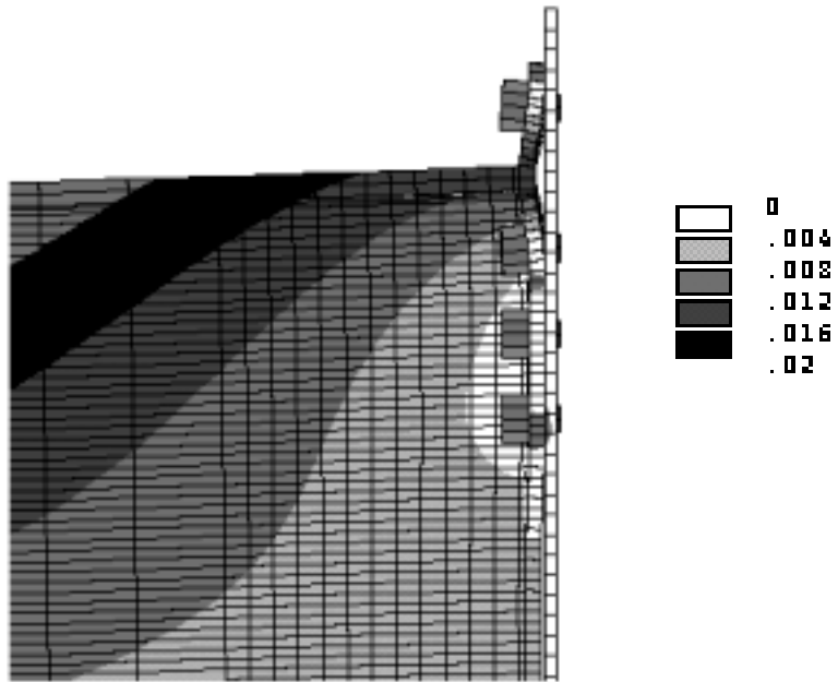
FIGURE 3-11. End-plate separation (inches) at ultimate applied moment for deep beam.
