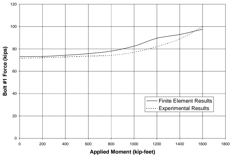
FIGURE 3-12. Bolt #1 force vs. applied moment for deep beam.
