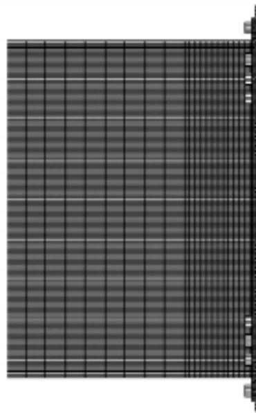
FIGURE 3-10. Finite element mesh for MRE-1/3-1 1/4-5/8-62 (deep beam to rigid column flange).
