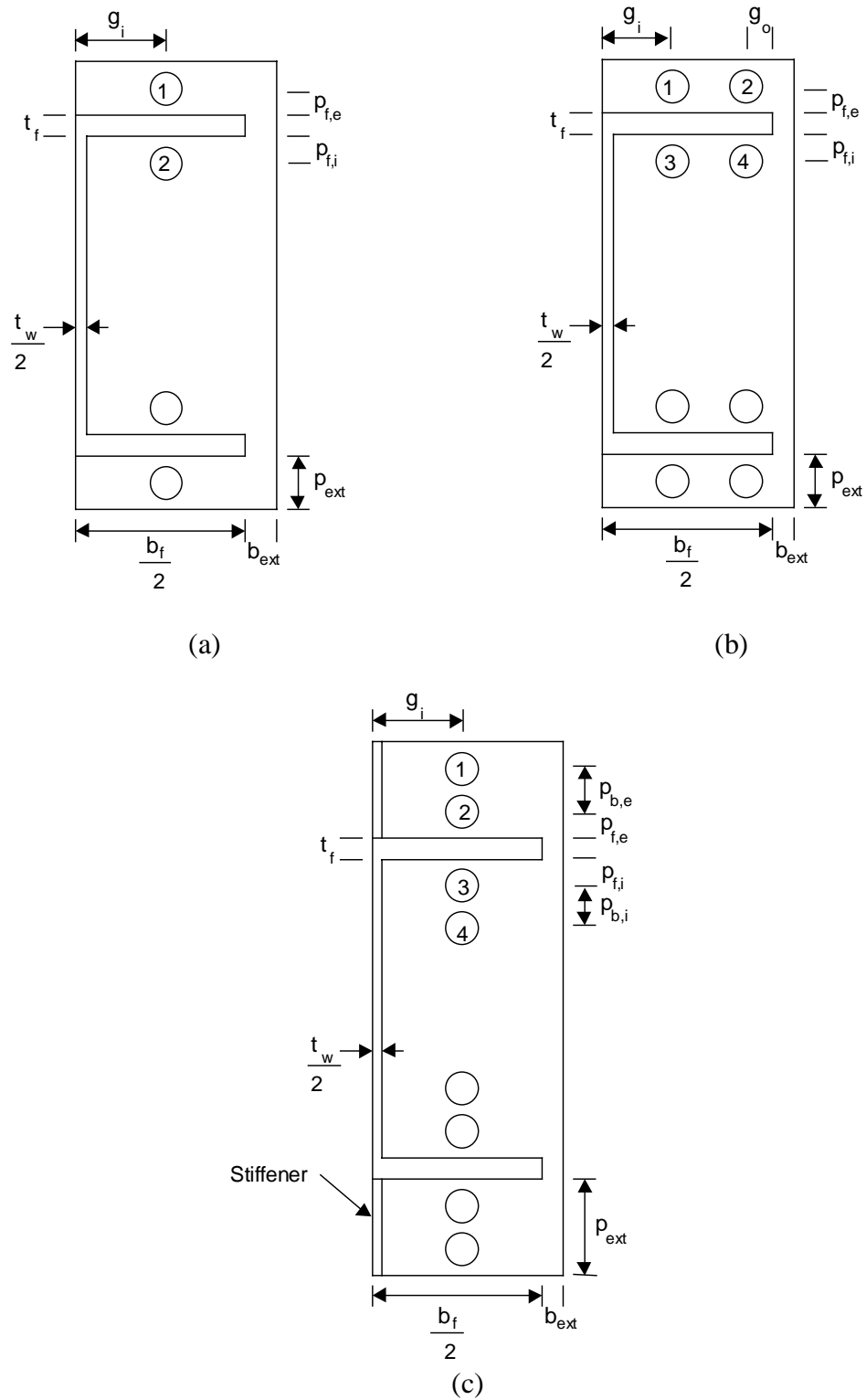
FIGURE 4-1. (a) Four-bolt extended unstiffened, (b) four-bolt wide, and (c) eight-bolt extended stiffened moment end-plate configurations.
