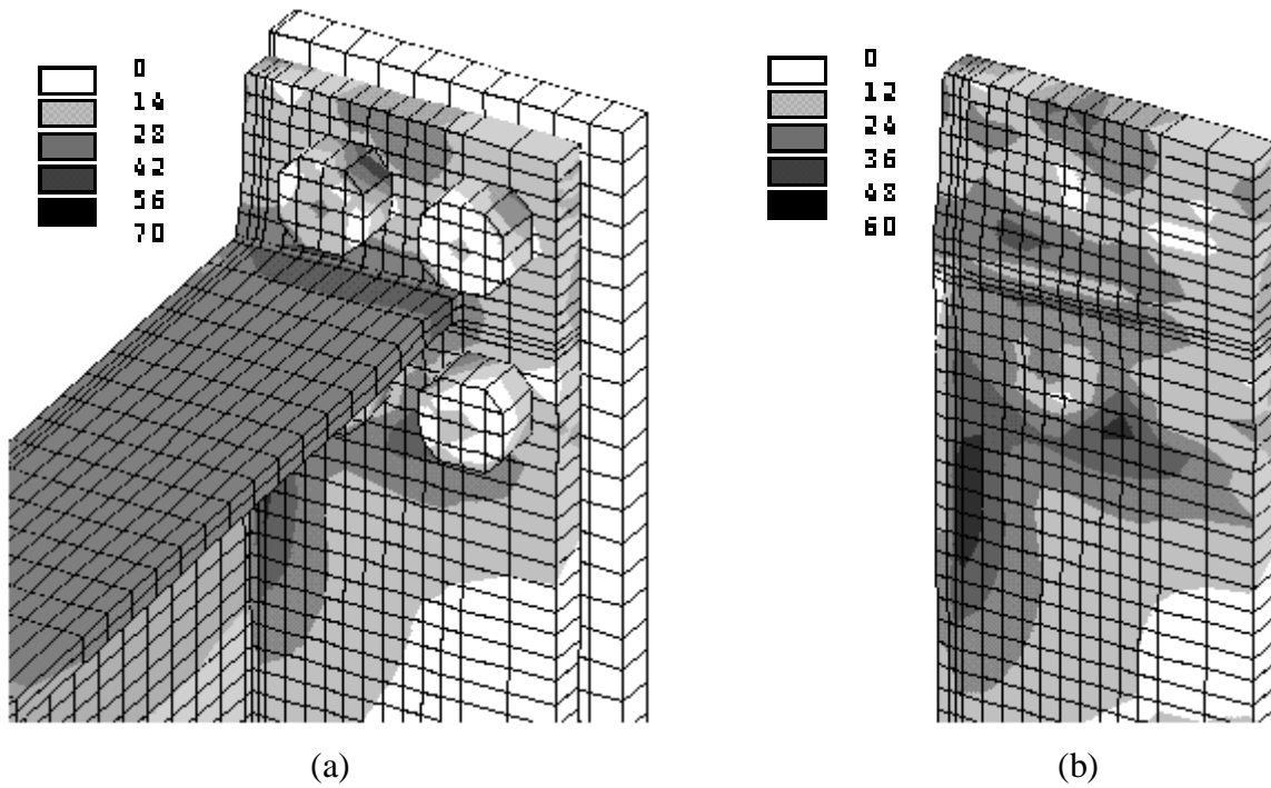
FIGURE 4-4. Von Mises stress (ksi) distribution across tension region of four-bolt wide (a) beam-to-column flange connection and (b) isolated end-plate.
