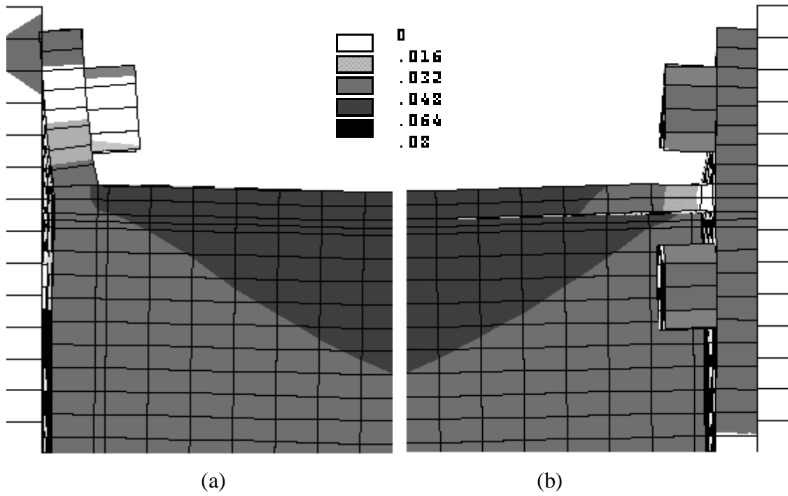
FIGURE 4-5. Plate separation (in.) at tension flange region of four-bolt wide beam-to-column flange connection shown as (a) back view and (b) front view.
