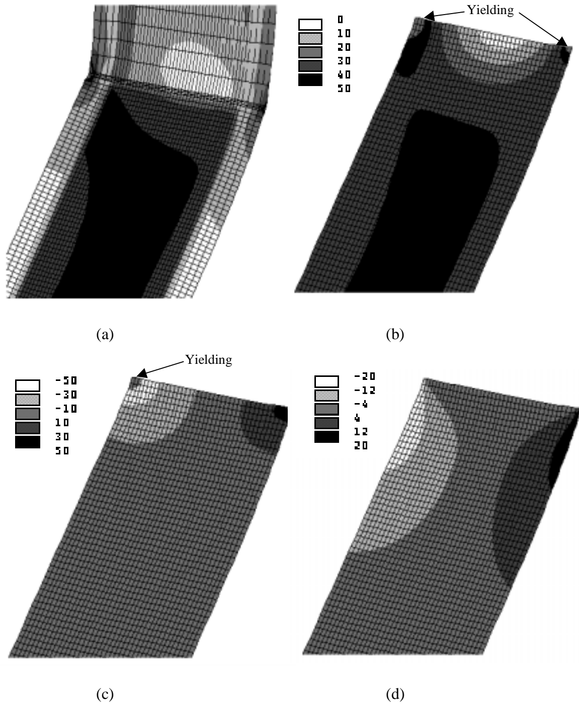
FIGURE 7-5. Elastic stress (ksi) distribution for case IB: (a) column panel zone (von Mises); (b) doubler plate (von Mises); (c) doubler plate (horizontal shear stress); (d) doubler plate (vertical shear stress).
