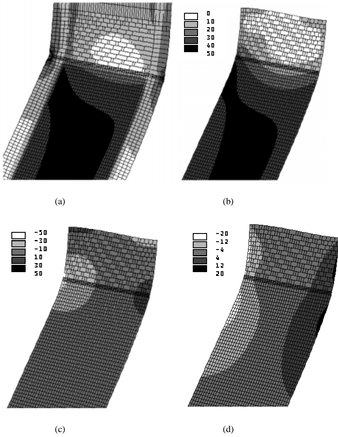
FIGURE 7-7. Elastic stress (ksi) distribution for case IIB: (a) column panel zone (von Mises); (b) doubler plate (von Mises); (c) doubler plate (horizontal shear stress); (d) doubler plate (vertical shear stress).
