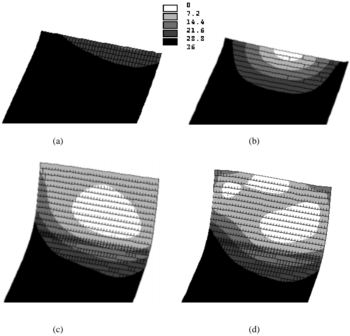
FIGURE 7-8. Von Mises stress (ksi) distribution at doubler plate for case: (a) IA-PL; (b) IB-PL; (c) IIA-PL; (d) IIB-PL.
