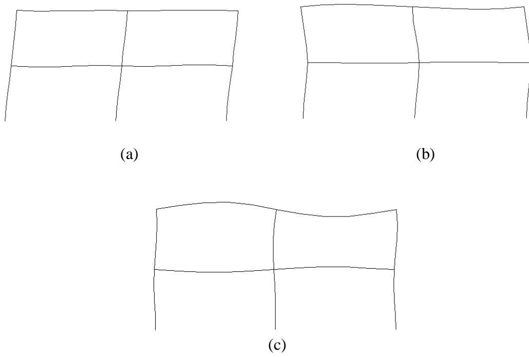
FIGURE 8-26. First three mode shapes for 8ES frame.
