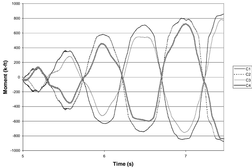
FIGURE 8-30. Moment occurring at each connection vs. time for the 4E (partially restrained/thin plate) frame.
