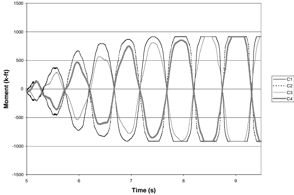
FIGURE 8-29. Moment occurring at each connection vs. time for the 4E (partially restrained/thick plate) frame.
