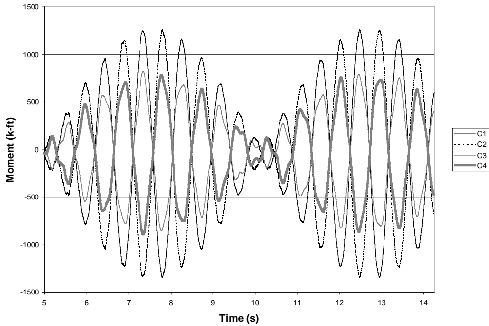
FIGURE 8-28. Moment occurring at each connection vs. time for the 4E (fully restrained/elastic connection) frame.
