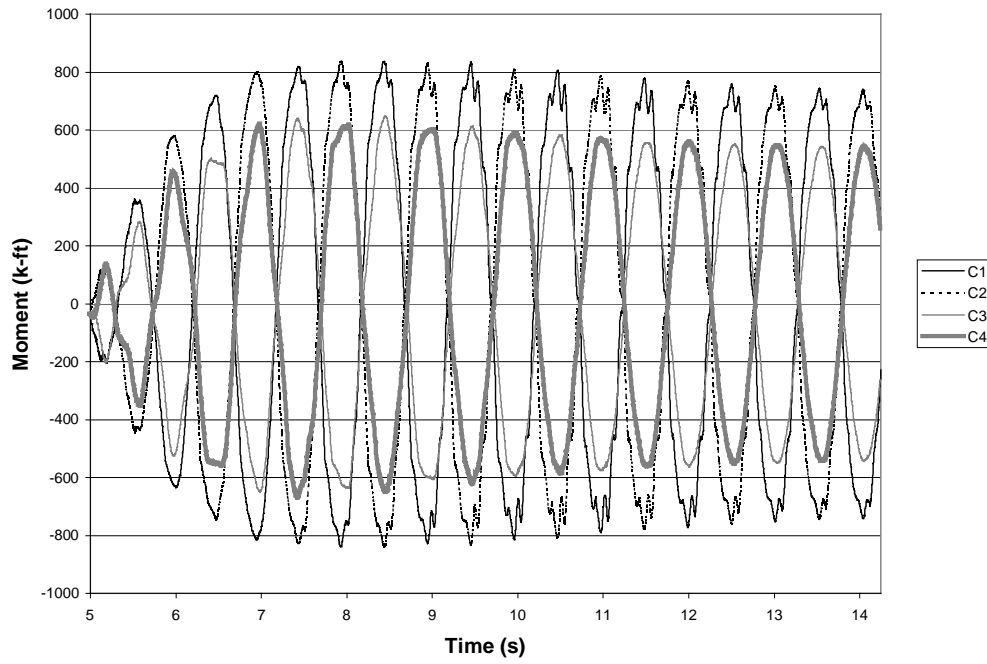
FIGURE 8-32. Moment occurring at each connection vs. time for the 4E (hysteretic behavior/thin plate) frame.
