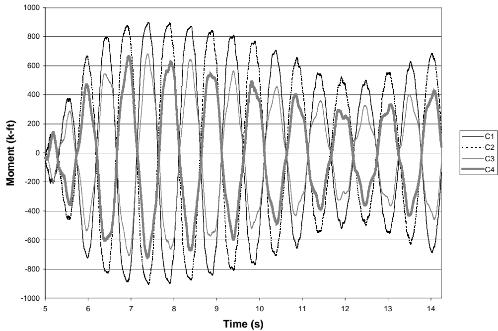
FIGURE 8-31. Moment occurring at each connection vs. time for the 4E (hysteretic behavior/thick plate) frame.
