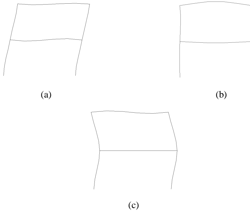
FIGURE 8-25. First three mode shapes for 4E frame.
