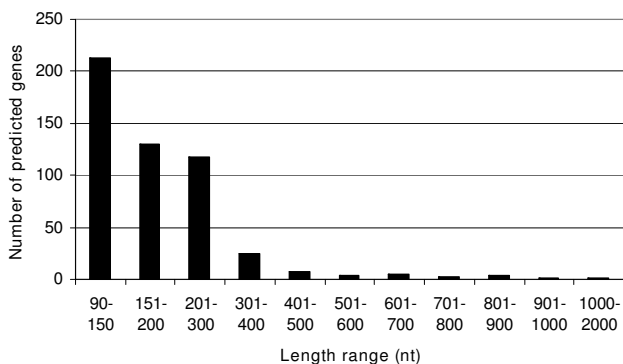
Figure 1 Length distribution of predicted gene candidates.
