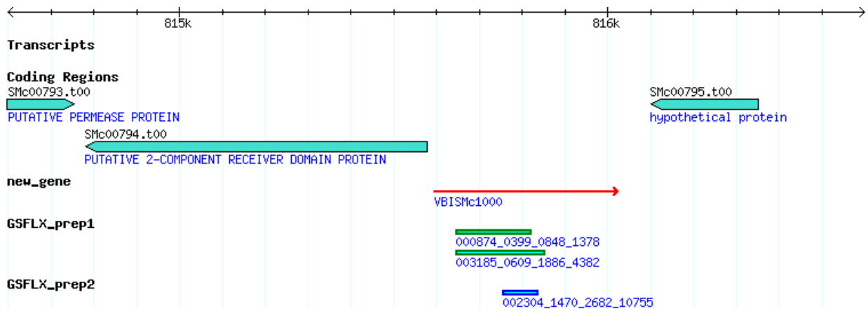
Figure 3 Genome view of a new gene (in red). GLX sequences (in green from prep 1 and in blue from prep 2) are aligned to VBISM1000.
