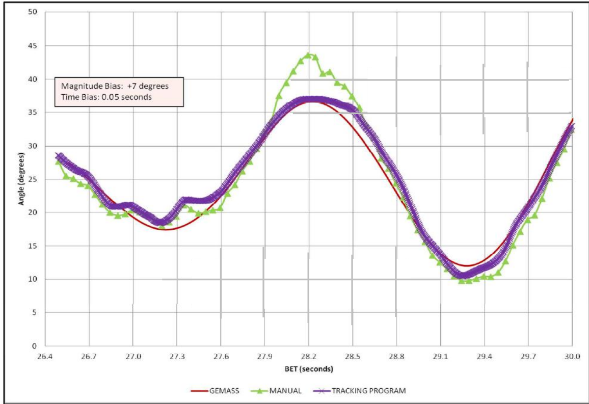
Figure 1-10: Apollo model comparison to Pad Abort-1 drogue parachute pitch angle with bias and time shift [9].
