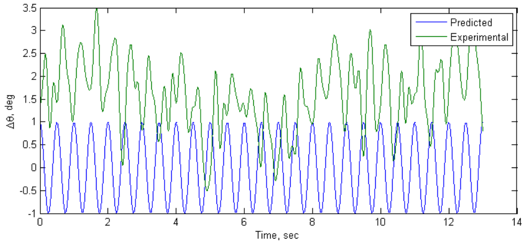
Figure 4-5: Predicted versus experimental drogue chute \Delta\theta time history
