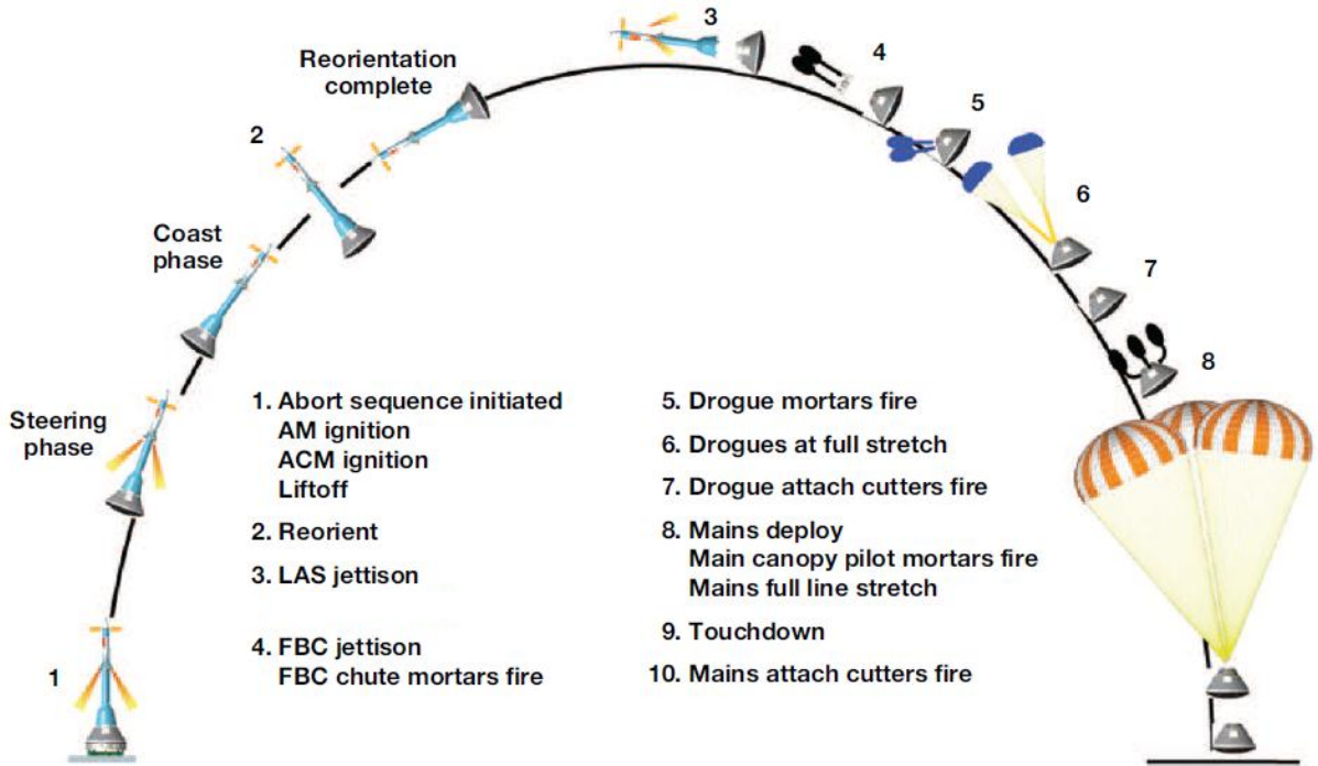
Figure 1-4: Launch Abort System PA-1 flight profile [8].
