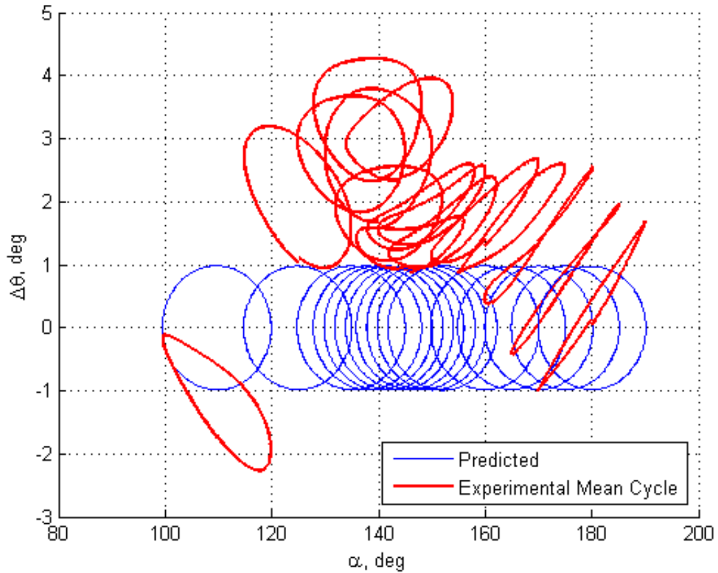
Figure 4-7: Predicted versus experimental \Delta\theta mean cycles ( k = 0.123 , \hat{q}_{max} = 0.021 ).
