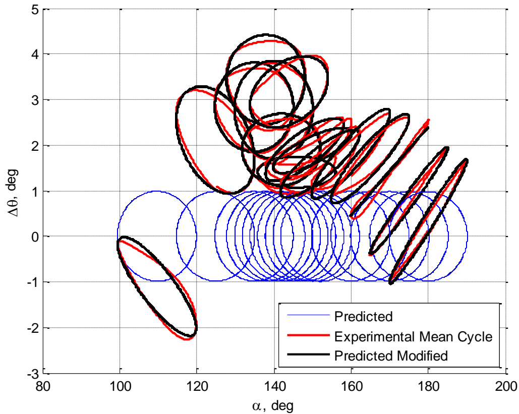
Figure 4-10: Time shift, bias, and scale factor in predicted \Delta\theta to replicate experimental \Delta\theta ( k = 0.123 , \hat{q}_{max} = 0.021 ).
