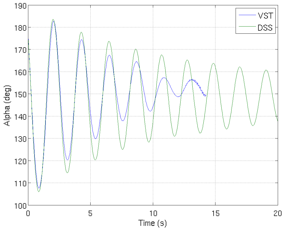
Figure 1-6: Angle of attack time history: DSS analytical simulation versus VST subscale free-flight test [9].
