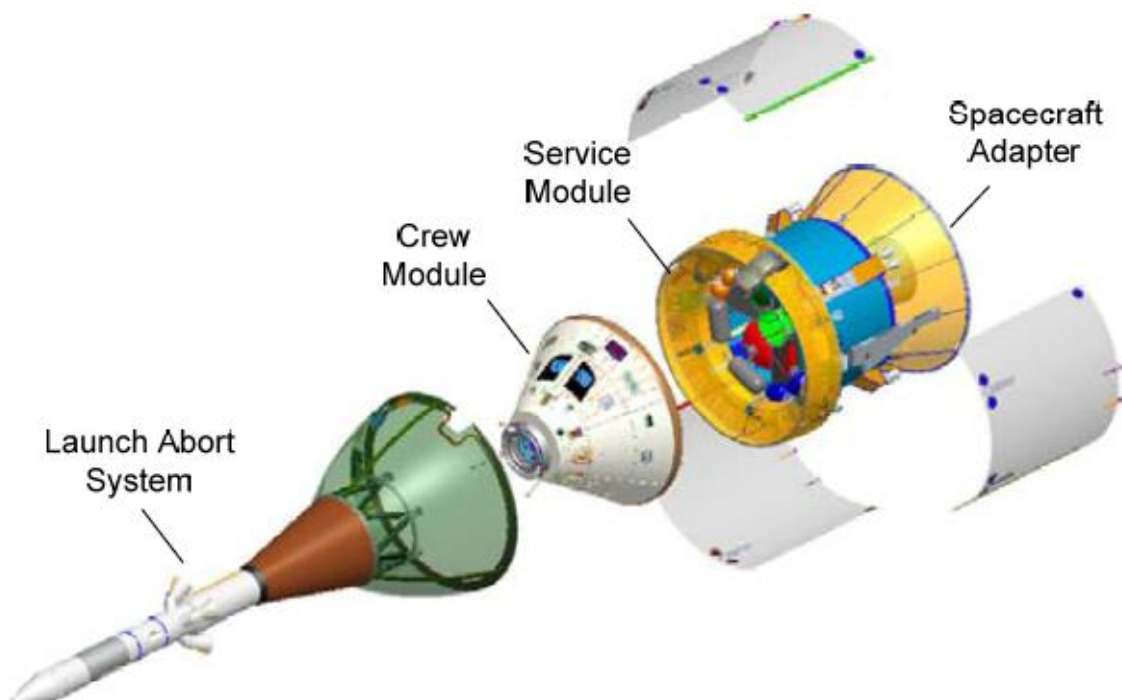
Figure 1-1: Orion Multi-Purpose Crew Vehicle (MPCV) (Image credit: NASA).
