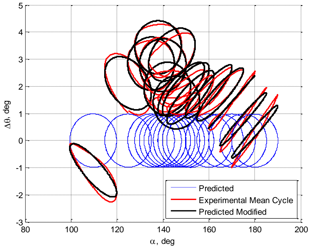
Figure 4-9: Time shift and bias in predicted \Delta\theta to replicate experimental \Delta\theta ( k = 0.123, \hat{q}_{max} = 0.021 ).
