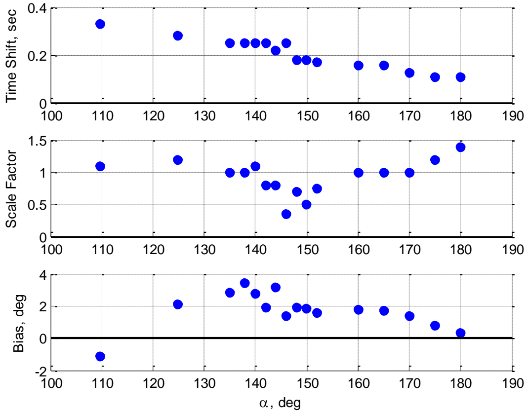
Figure 4-11: Time shift, bias, and scale factor parameters versus angle of attack ( k = 0.123 , \hat{q}_{max} = 0.021 ).
