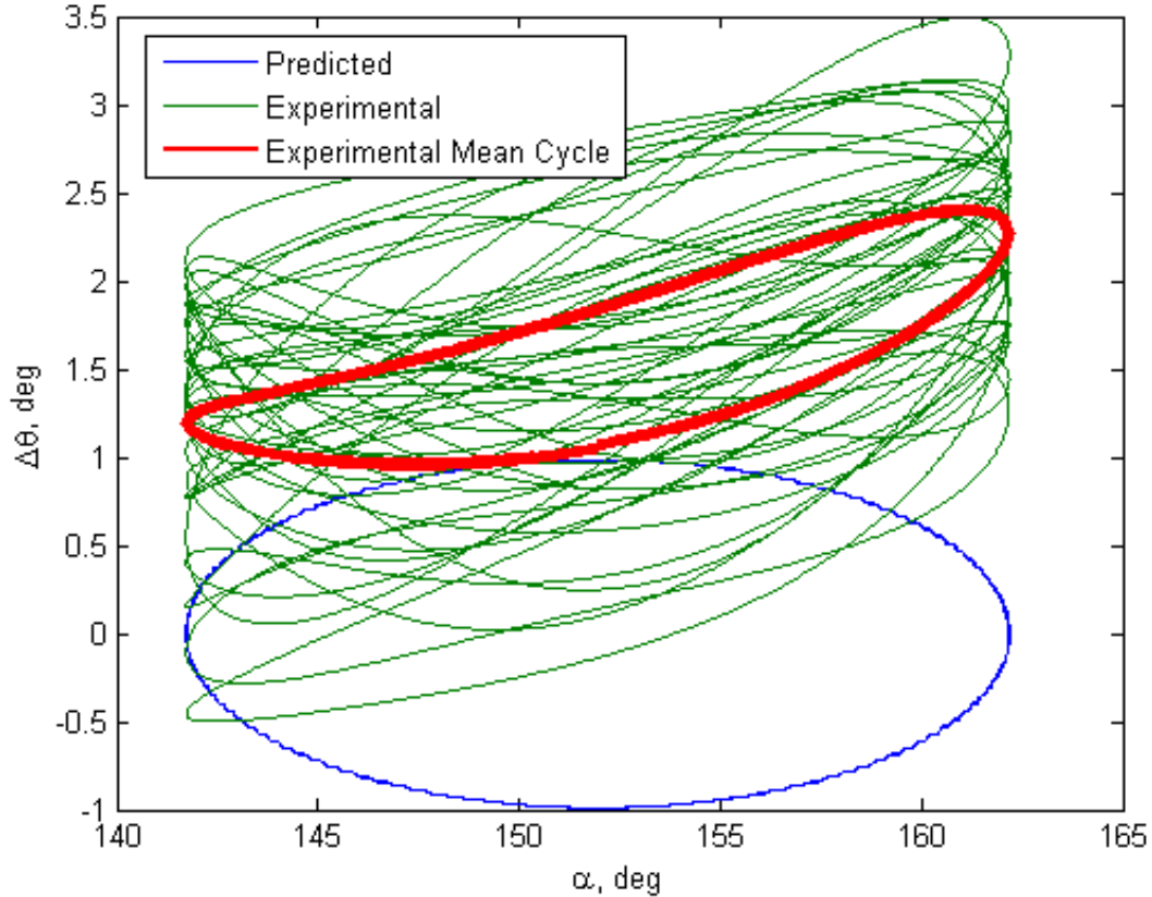
Figure 4-6: \Delta\theta versus CM angle of attack ( k = 0.123 , \hat{q}_{max} = 0.021 , \alpha = 152^\circ ).
