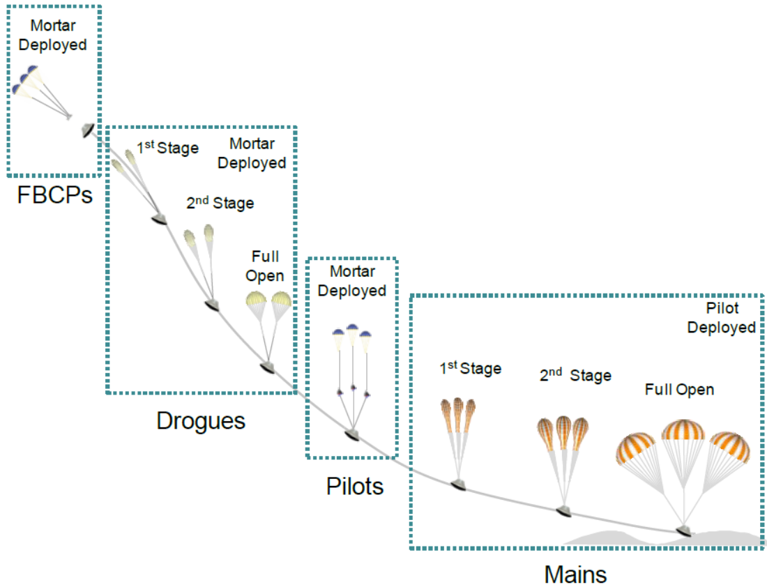
Figure 1-3: Parachute sequence for Crew Module [3].
