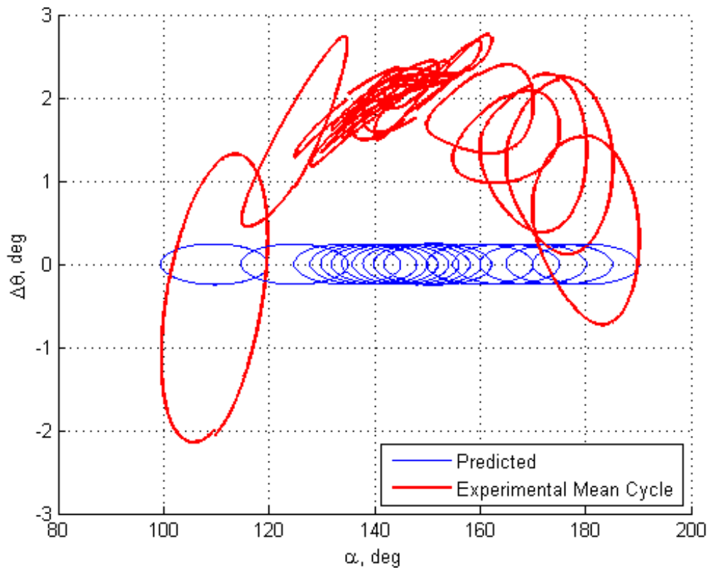
Figure 4-14: Predicted versus experimental \Delta\theta mean cycles for k = 0.042 , \hat{q}_{max} = 0.007 .
