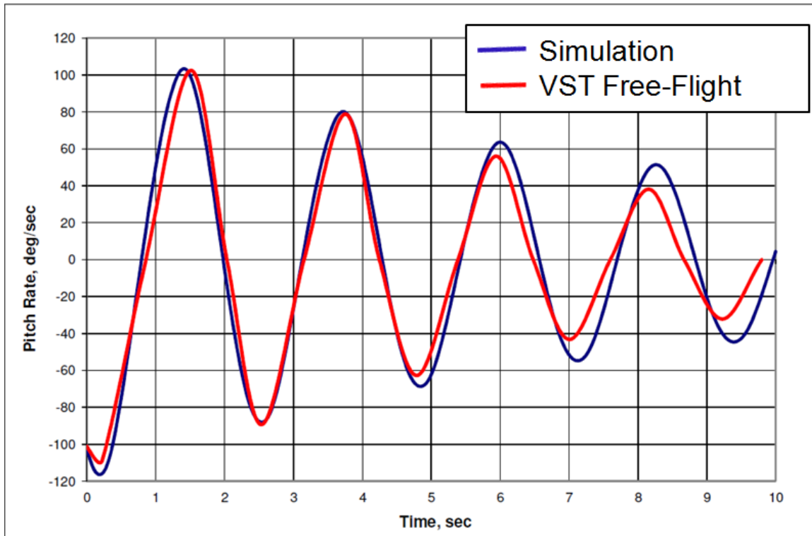
Figure 1-11: CM pitch rate time history comparison between Apollo drogue model and VST free-flight CM pitch rate [9].
