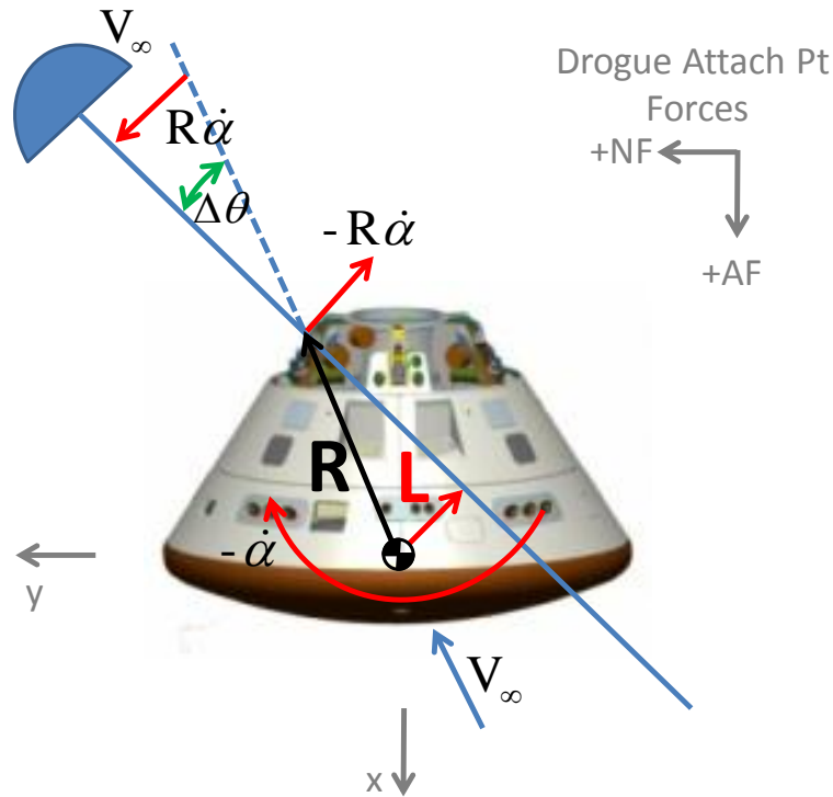
Figure 4-4: Diagram of CM-drogue system with coordinate system and drogue force coordinate system.
