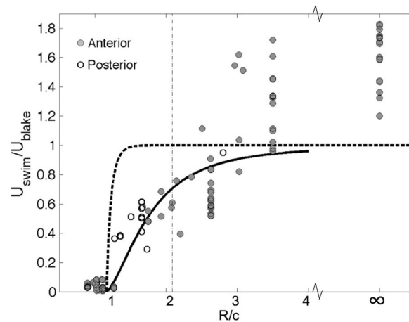
FIG. 6. Plot of normalized swimming velocity vs. the non-dimensional radius of the tube. Two different cases are compared, one with the dotted line shows the model of an infinite ciliate swimming in capillary tube. The solid line shows the velocity variation of the finite sized Paramecium inside confined geometries. Dots represent the experimental result and compares well with the finite pressure gradient model in the restrictive environment.
