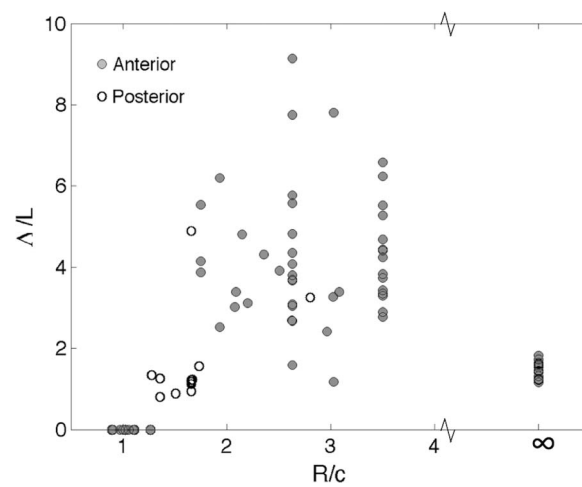
FIG. 7. Plot of the non-dimensional wavelength vs. non-dimensional radius of the tube. No apparent trend is seen for larger radius of the tube. In contrast while swimming in the semi-infinite domain the Paramecium has well defined wavelengths of the helical path.
