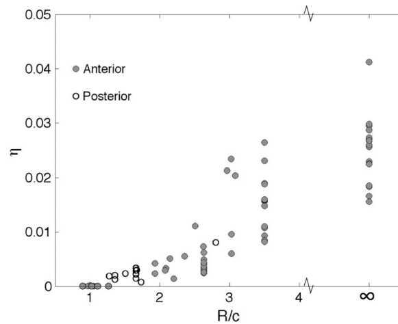
FIG. 8. Plot of the efficiency of the various trajectories inside the tube as well as semi-infinite domain from experiments as compared to a Paramecium swimming in semi-infinite fluid domain.
