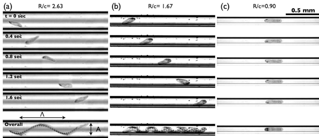
FIG. 3. Swimming of Paramecium in tubes of different diameters. \Lambda denotes the wavelength and A the amplitude of the helical trajectory traced by the organism in tubes of different diameter. (a) shows swimming in large tube ( R/c = 2.63 ) where the trajectory of the motion is helical. In swimming inside tubes of intermediate diameters ( R/c = 1.67 ) small wavelength helices are seen. In very small tubes ( R/c = 0.9 ) as shown in (c) Paramecium swims in a straight line.
