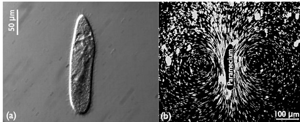
FIG. 1. (a) A Paramecium swimming in a thin layer of fluid. (b) Pathlines of particles in flows generated by the cilia.
