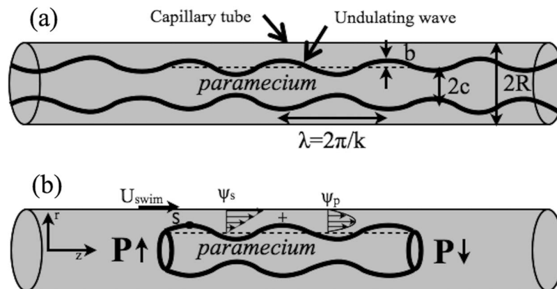
FIG. 4. Schematic of a wavy (a) infinite cylinder or (b) finite cylinder swimming inside the cylindrical tube. It is assumed that the organism is swimming in the negative z direction with a velocity U_{swim} . By transforming the coordinate system to one, where the organism is swimming with velocity U_{swim} we get the current schematic with the descriptions of the velocities on the walls of capillary.
