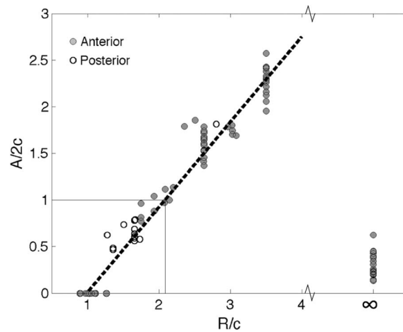
FIG. 5. Plot of the non-dimensional amplitude of the helical path vs. the non-dimensional radius of the tube. The plot shows a linear variation which increases with the radius of the tube.
