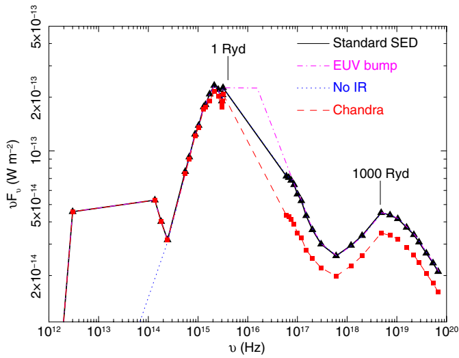
Fig. 3. SED used of Mrk 509 for the time-averaged XMM-Newton and Chandra observations. Data points from Table 2 are indicated with triangles and squares.
