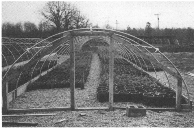
Plastic greenhouse for winter protection. Note simple construction with pipe or 10' sections of electrical conduit can be used. (Glenwood Nursery and Garden Center, Richmond, VA)
