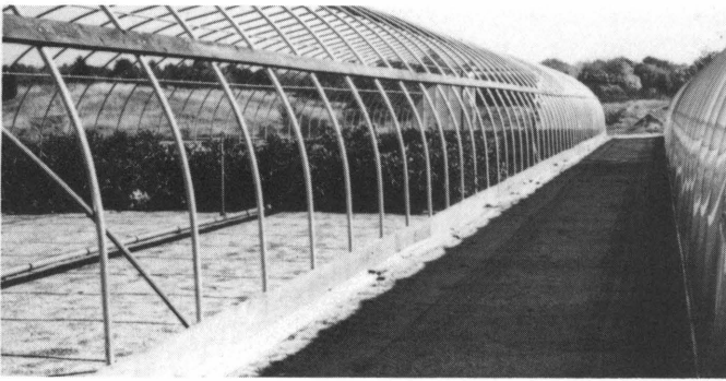
Pipe frame greenhouse for winter protection. Space between houses for spacing plants for summer growing and for moving into and out of greenhouses. This grower-constructed house is 196' long, 30' wide, and 14' high. (Roadview Farm Nursery, Gloucester, VA)
