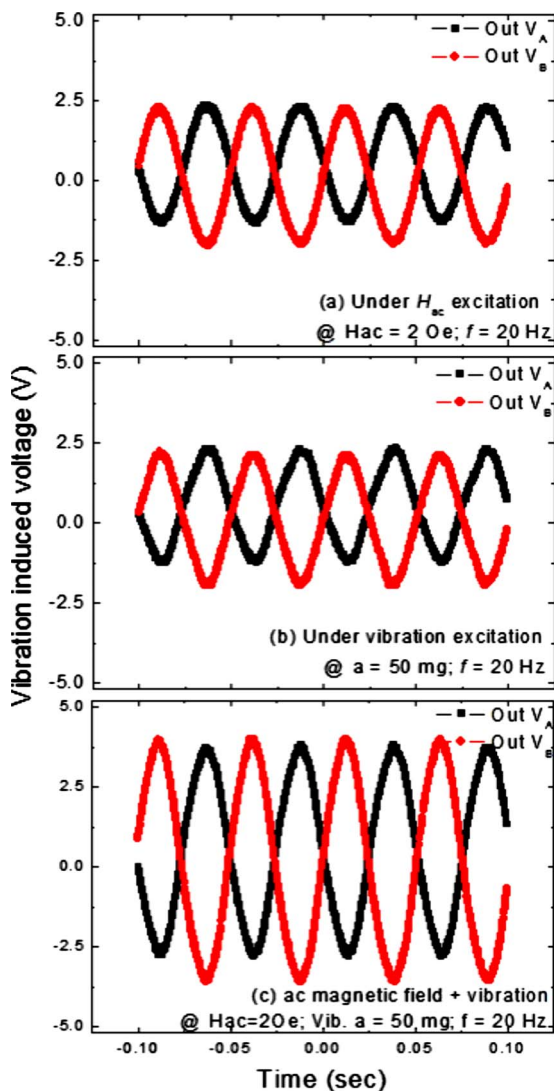
FIG. 4. (Color online) Experimental confirmation of the bimechanism for magnetic field and mechanical vibration EH: (a) under only a stray magnetic excitation of H_{ac}=2 Oe ( f=20 Hz), (b) under only a stray vibrational excitation of a=50 mg ( f=20 Hz), and (c) under both stray magnetic and vibrational excitations.
