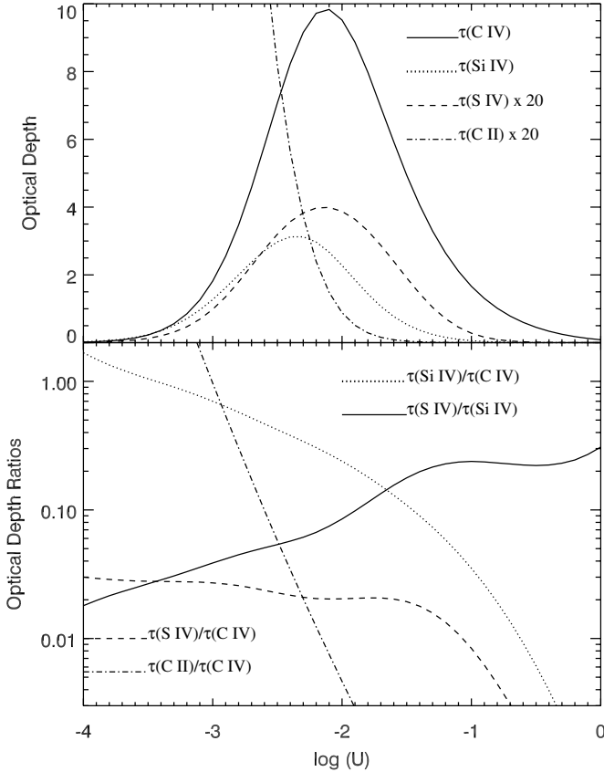
Figure 3. Expected optical depth for C IV, Si IV, S IV, and C II lines, from Equation (2), assuming solar abundances (Lodders et al. 2003) and normalizing to \tau_{\text{max}}(\text{C IV}) = 10 . We used an oscillator strength of 0.05 for S IV \lambda 1063 (Hibbert et al. 2002), 0.19 for C IV \lambda 1548 , 0.52 for S IV \lambda 1393 , and 0.13 for C II \lambda 1334 (Kurucz & Bell 1995). Ionization fractions were calculated with the photoionization code CLOUDY using a Mathews & Ferland (1987) SED.
