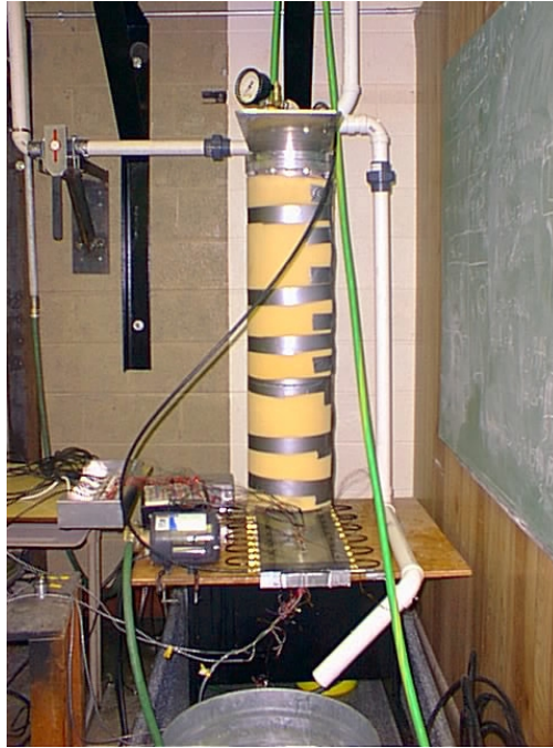
Figure 119. Photograph of calibration rig.
