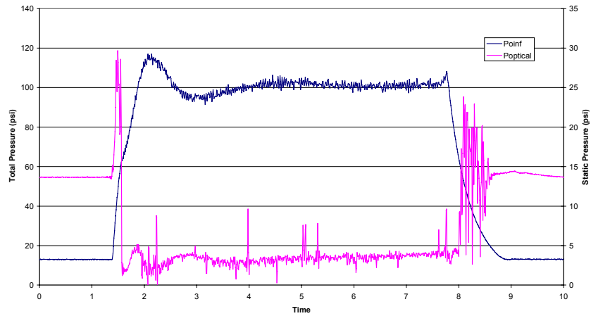
Pressure - Run 9
