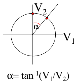
Figure 35. Idealized Lissajous figure of dual-wavelength output.
