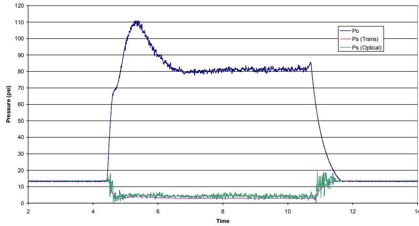
Pressure - Run 25
