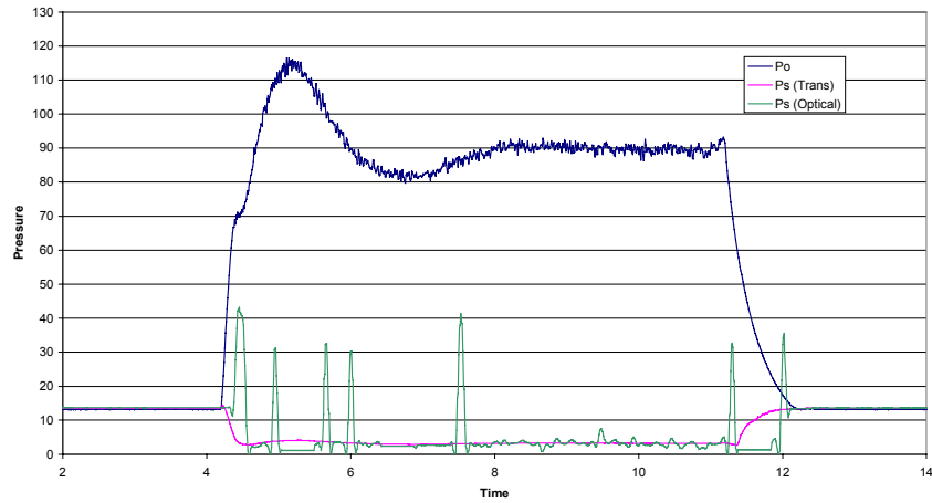
Pressure - Run 24
