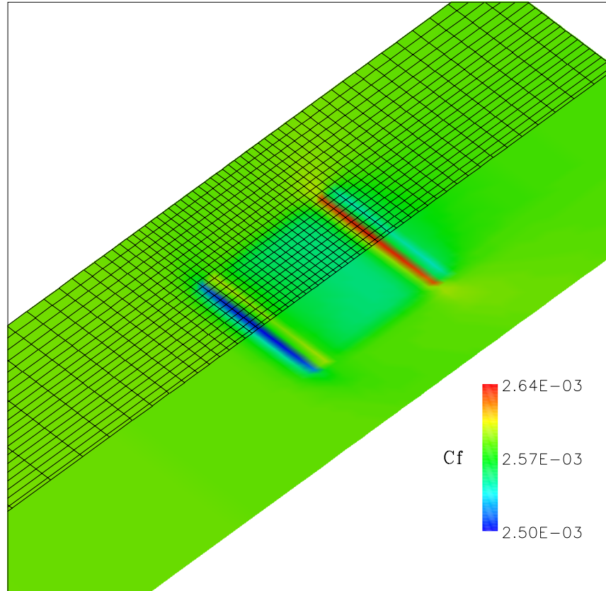
Figure 51. Computational skin friction results for a Mach 3 flow and 60 °C temperature difference. Note that the flow direction is from left-to-right. 81
