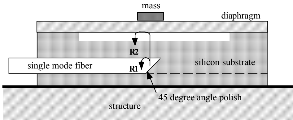
Figure 152. Sketch of the fiber optic accelerometer. 97
