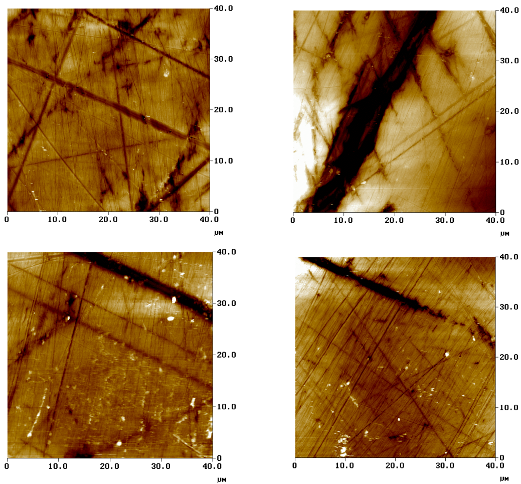
Figure 168. AFM of portions of typical skin friction sensor reflector (darkening of shade indicates a deeper surface).
