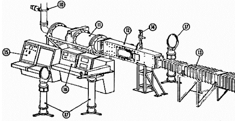
Figure 85. Virginia Tech supersonic wind tunnel.
