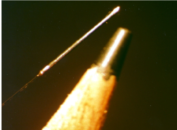
Figure 81. Photograph of fiber optic temperature sensor using metal wire.
