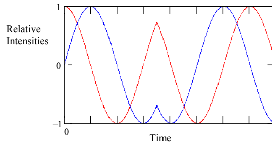
Figure 34. Two-λ system theoretical output showing the phase lead/lag relationship at a direction change.
