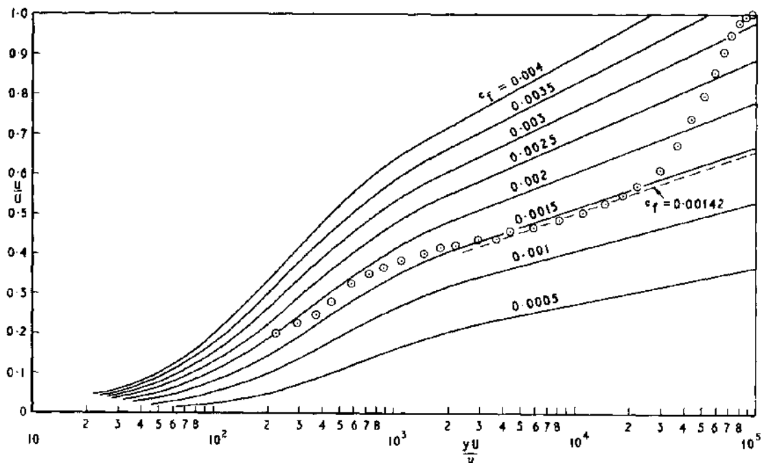
Figure 4. Clauser chart. (from Winter 10 )
