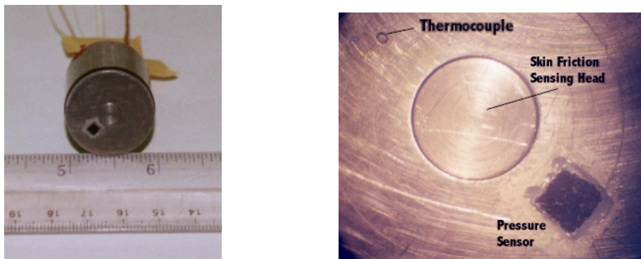
Figure 107. Photographs of the Version 3 skin friction sensor.
