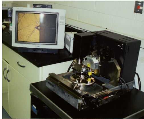
Figure 166. Photograph of the AFM setup.
