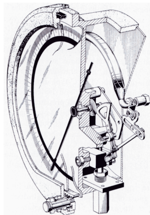
Figure 16. Bourdon tube. 26
