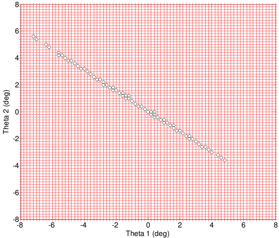
Figure 5.15: Global view of the basin of stability based on the outcomes of trajectories. Circles show initial locations where trajectories remained in the neighborhood of the origin. Crosses represent initial locations that resulted in unstable trajectories.
