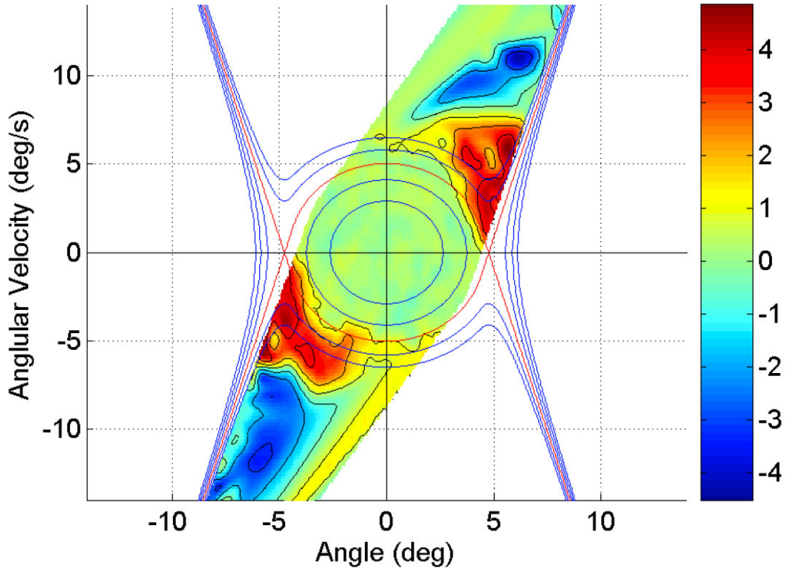
Figure 4.19: At an evolution time of T = 0.6 seconds the LCS is observable near the ejection points in state space.
