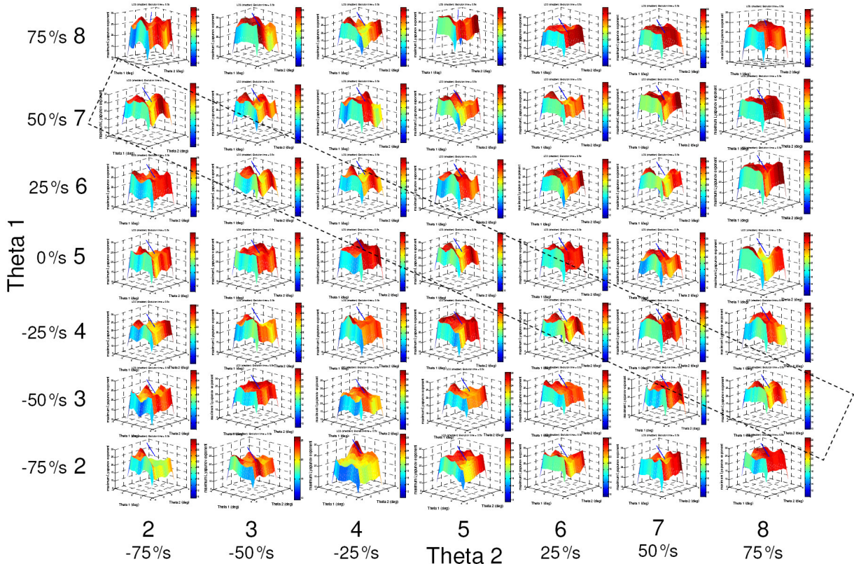
Figure 5.30: The 2-dimensional figures are arranged into a two dimensional grid. By comparing the figures at different grid locations, the full four dimensional basin of stability can be visualized (see associated document, “4D Basin of Stability”)
