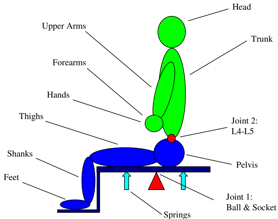
Figure 5.2: Model of the person sitting on the wobble chair. Blue components contribute to segment one. Green components make up segment 2. The joints are shown in red and the springs in aqua.
