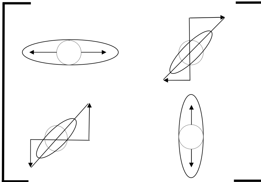
Figure 5.23: Graphical representation of the terms that make up the state transition matrix.
