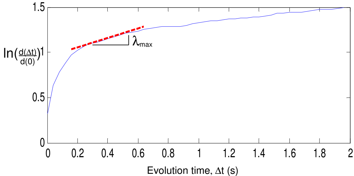
Figure 2.4: The maximum Lyapunov exponent was determined by calculating the slope of the mean expansion as a function of the evolution time.
