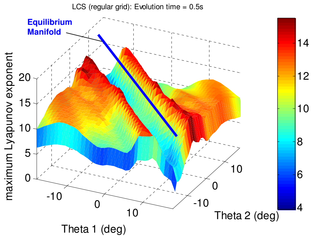
Figure 5.10: LCS are visible in both the (a) top view and (b) 3D view of the FTLE field for the Acrobot.
