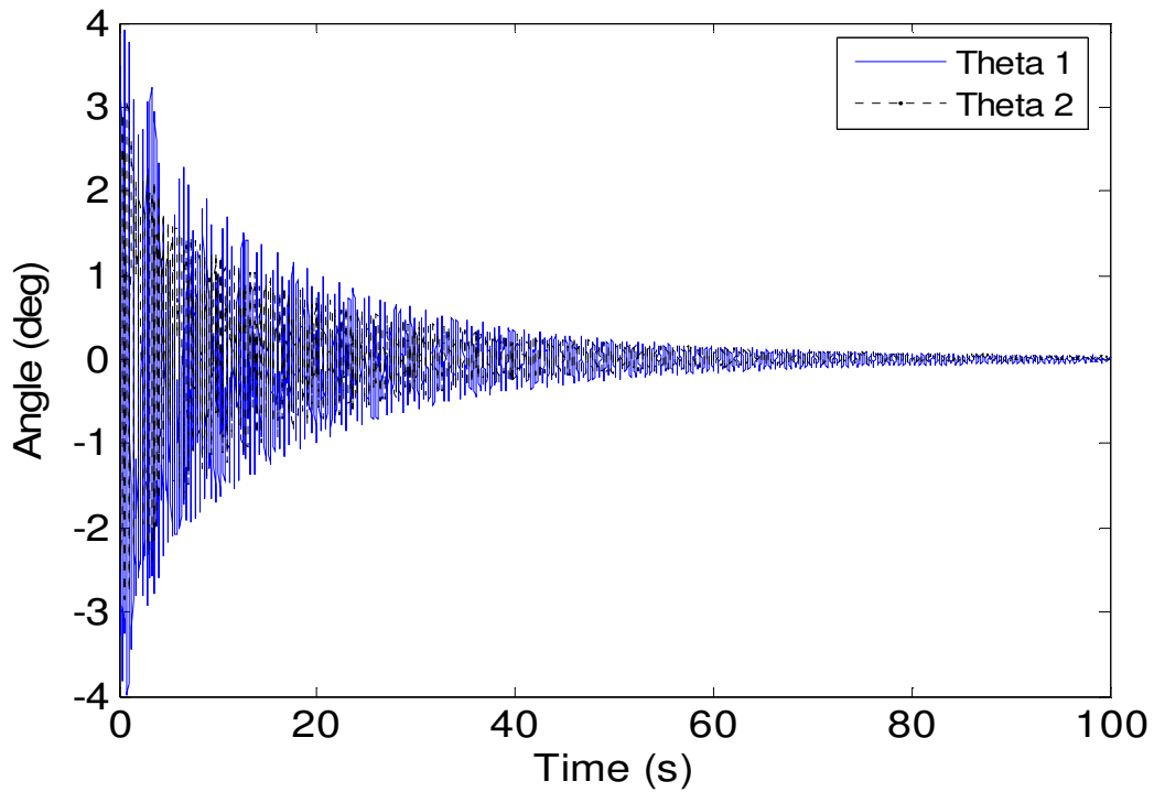
Figure 5.13: Time plot for the upper and lower segments of the wobble chair.
