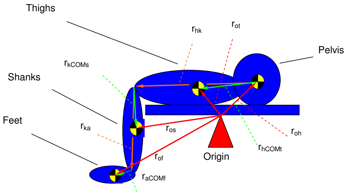
Figure 5.3: Vectors were used to find the locations of the center of mass of each body segment.
