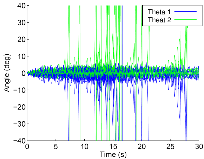
Figure 5.20: Time plot for the upper and lower segments of the wobble chair. Both stable and unstable dynamics are visible.
