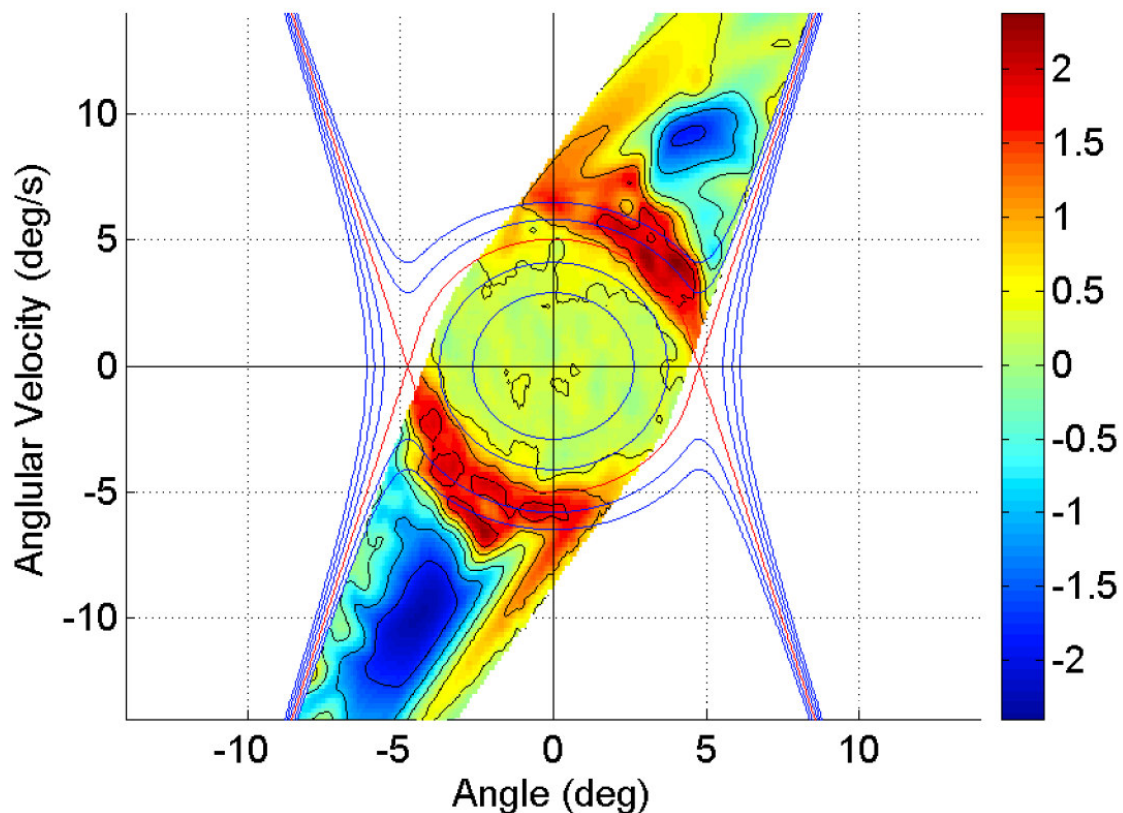
Figure 4.20: By T = 1.2 seconds the LCS is clearly observable spanning more of the boundary.
