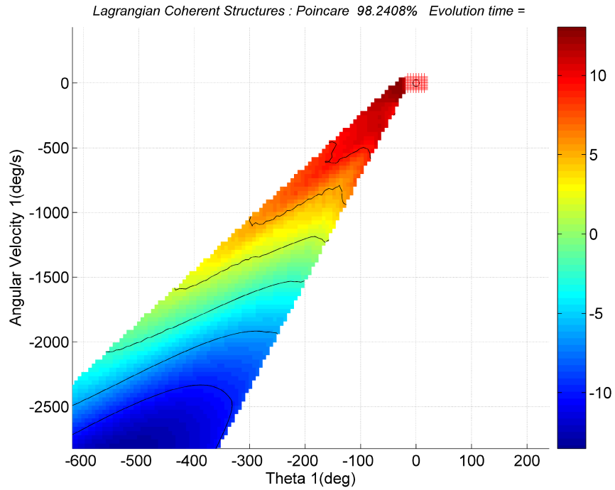
Figure 5.25: FTLE field for the wobble chair generated using the Euclidean distance method. This two dimensional plot shows the (\theta_1, \dot{\theta}_1) slice of state space. The position and velocity of \theta_2 is reduced to a 10% band around (\theta_2 = 0, \dot{\theta}_2 = 0) .
