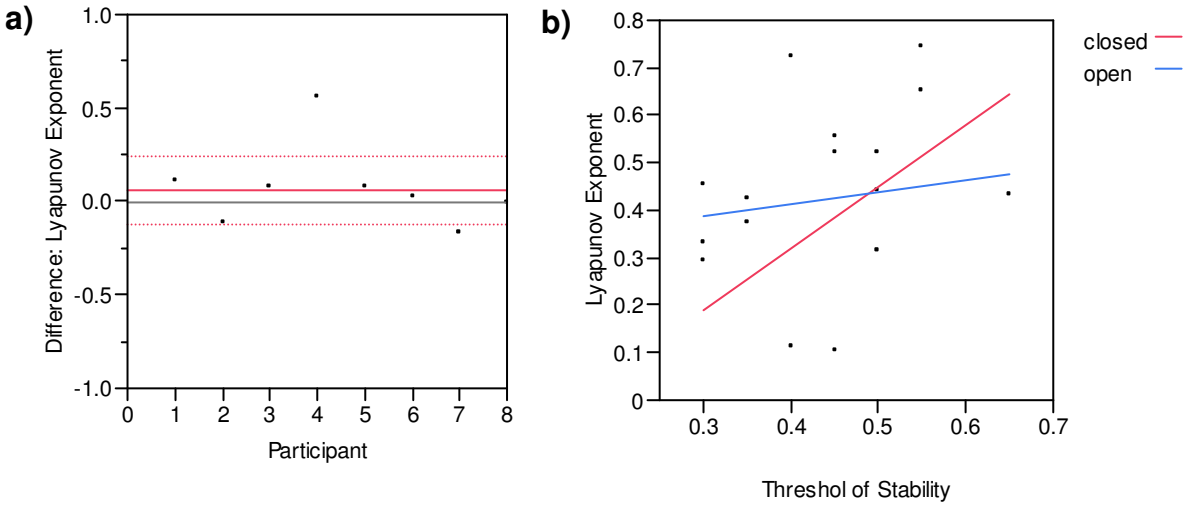
Figure 3.7: a) Difference in the maximum Lyapunov exponent was insignificant. b) Covariant analysis also showed no significant difference.
