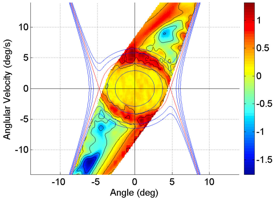
Figure 4.21: By T = 1.2 seconds the LCS is clearly observable spanning more of the boundary.
