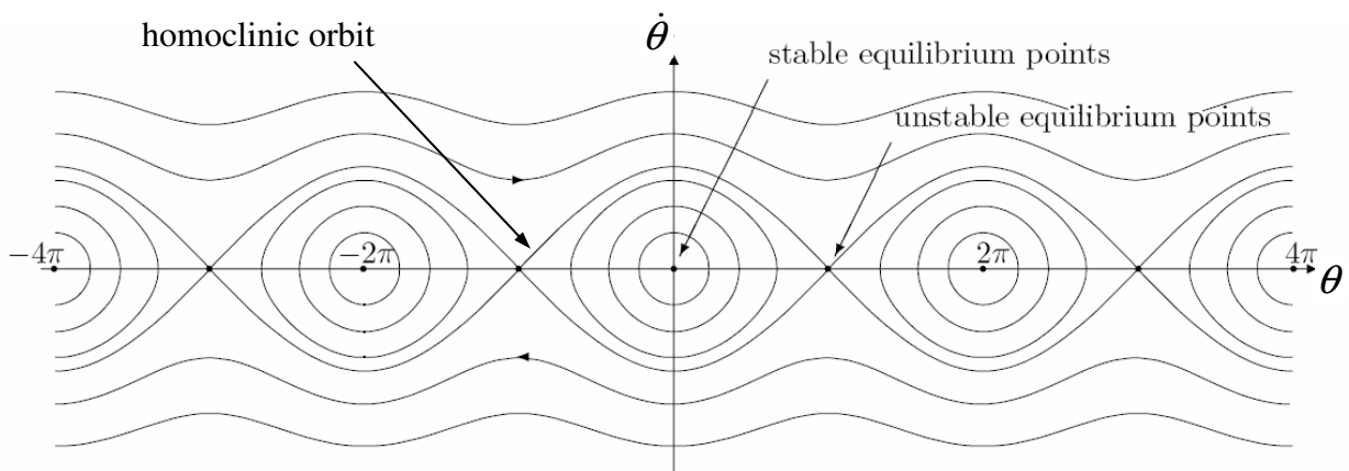
Figure 1.3: Phase plot of a single planar pendulum. Nearly circular trajectories around the stable equilibrium points represent oscillating motion. Larger almost elliptical trajectories indicate higher amplitude oscillations. The undulating lines on the top and bottom represent circular orbits in a single direction.
