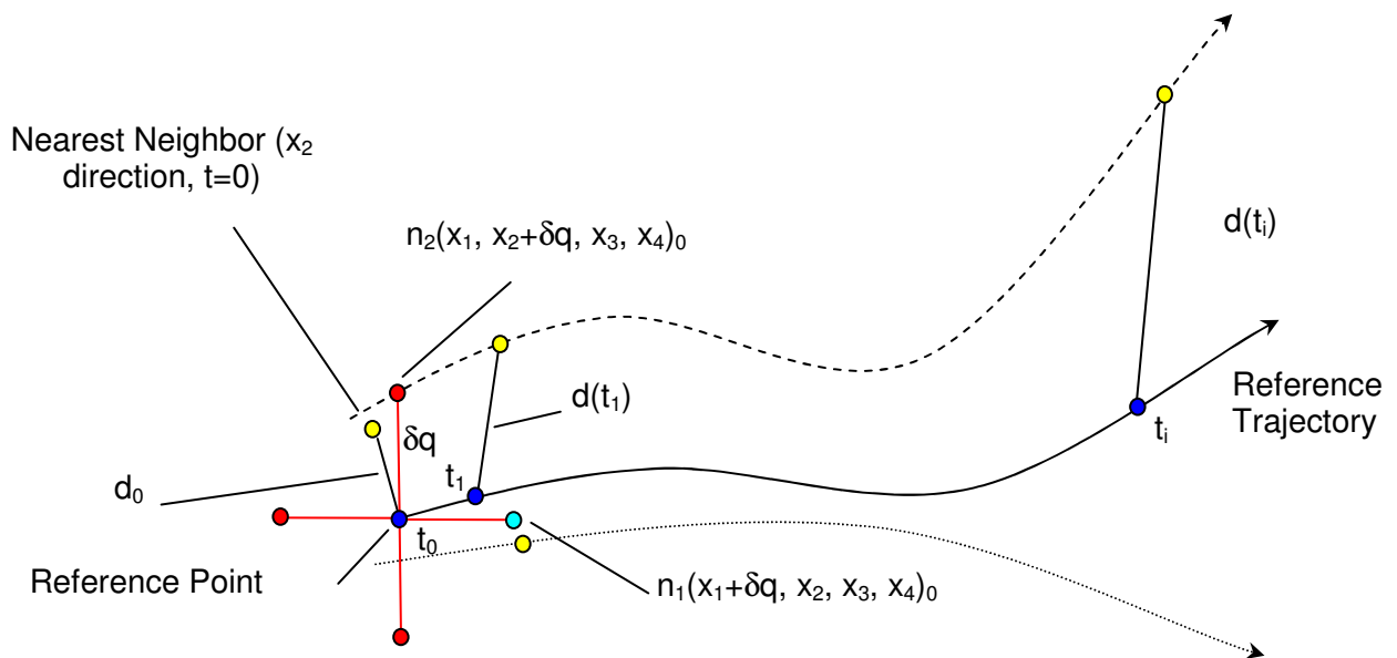
Figure 4.17: The maximum FTLE is found by calculating the growth of perturbation vectors in multiple state space directions. The assumption is made that the maximum FTLE dominates the evolution of the perturbation vectors.
