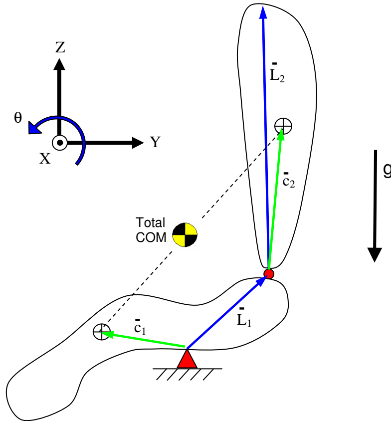
Figure 5.4: Simplified model of the person sitting on the wobble chair. Position vectors, \bar{L}_1 and \bar{L}_2 , show the connectivity of the model. Vectors \bar{c}_1 and \bar{c}_2 are from the joint to the center of mass of each segment. In the initial balanced configuration shown, the segment angles \theta_1 and \theta_2 are set to zero.
