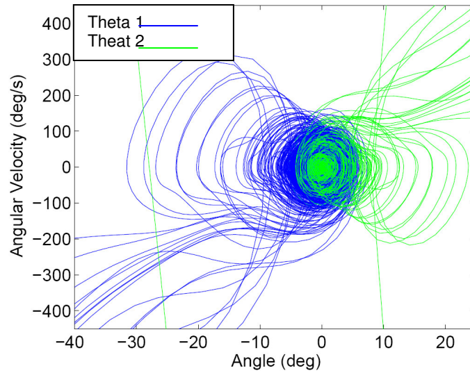
Figure 5.21: Phase plot for the upper and lower segments of the wobble chair. Both stable and unstable dynamics are visible. Stable behavior occurs within \sim 4 degrees of the origin (see 5.24).
