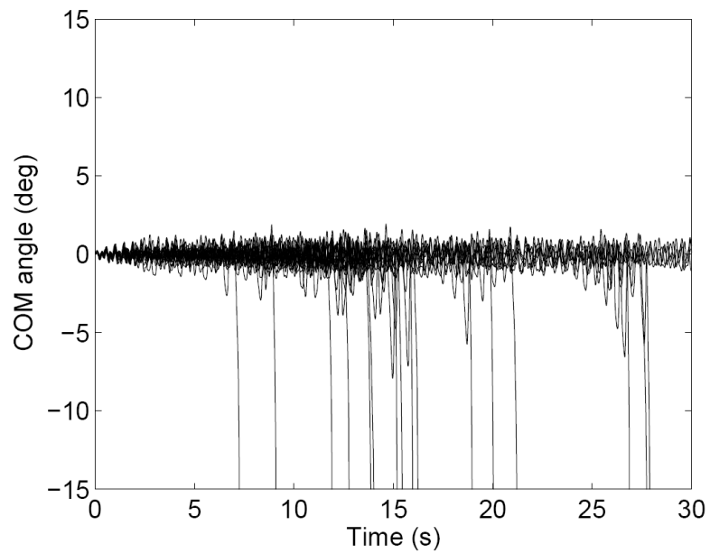
Figure 5.19: Simulation results showing the location of the center of mass over 50 trials. The PD controller drove the system towards the equilibrium manifold.
