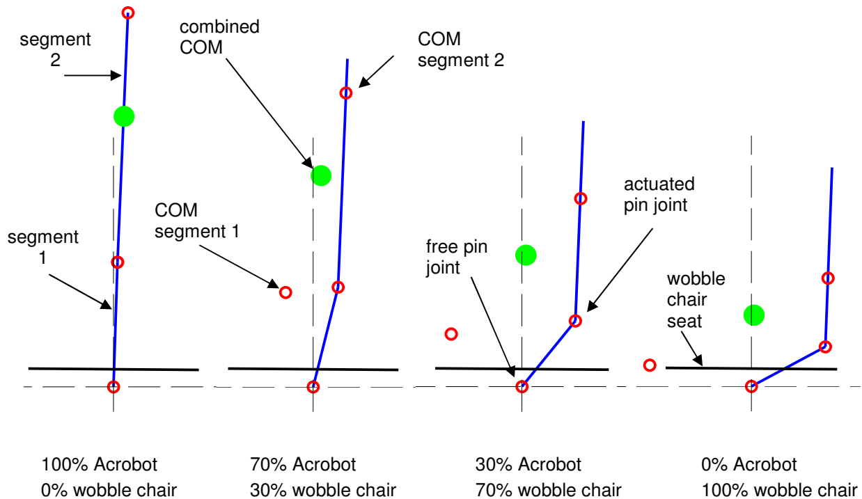
Figure 5.1: Center of mass and segment vectors for the Acrobat were slowly changed to those of the wobble chair. This effectively morphed one model into the other.
