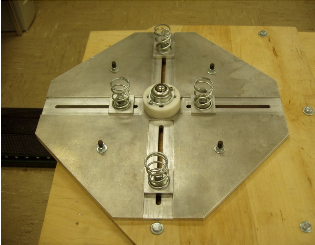
Figure 3.2: The wobble chair has four stabilizing springs that can be set to different distances to control the amount of restorative torque applied to the participant (photo by M. Tanaka).
