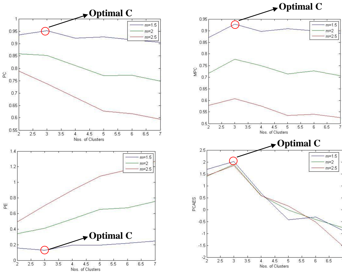
Figure 7.3. Input = x_1 , 0 \leq x_j \leq 3 , m = (1.5, 2, 2.5) , FCM Iterations = 40 (PC, MPC, PE, and PCAES validity test)
