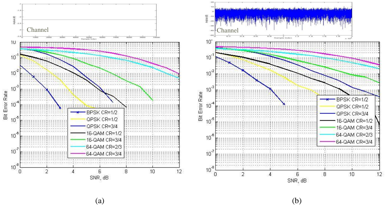
Figure 6.2 The Seven WiMAX Combinations for a (a) Flat Slow-Fading Channel and (b) Frequency-Selective Fast-Fading Channel. (The number of samples used were 10000 and MRC paths = 3.)
