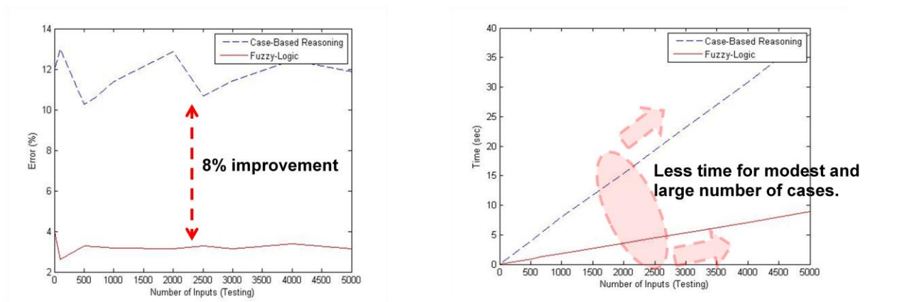
Figure 5.7 Comparison between CBR Engine and a Fuzzy logic Engine in Terms of the Error (%) and Time (sec), 1000 Cases Were Used for Training.
