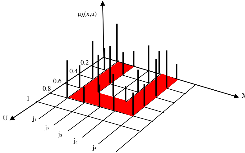
Figure 3.11 Foot Print Uncertainty (FOU) for Different Values of x Showing the set of Possible u Values ( j_x ), for Example for x=3 j_x=[0.6, 0.8] . J_x is Called the Primary Membership of x and is the Domain of the Secondary Membership Function. The Amplitude of the ‘Sticks’ is called a Secondary Grade
