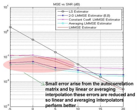
Number of Subcarriers=124, Rayleigh Channel (4 paths), AWGN, Doppler Frequency= 50Hz, D_t=8 , D_f=8 , T_S=1/10000 , SNR=-5 to 20 dB.
