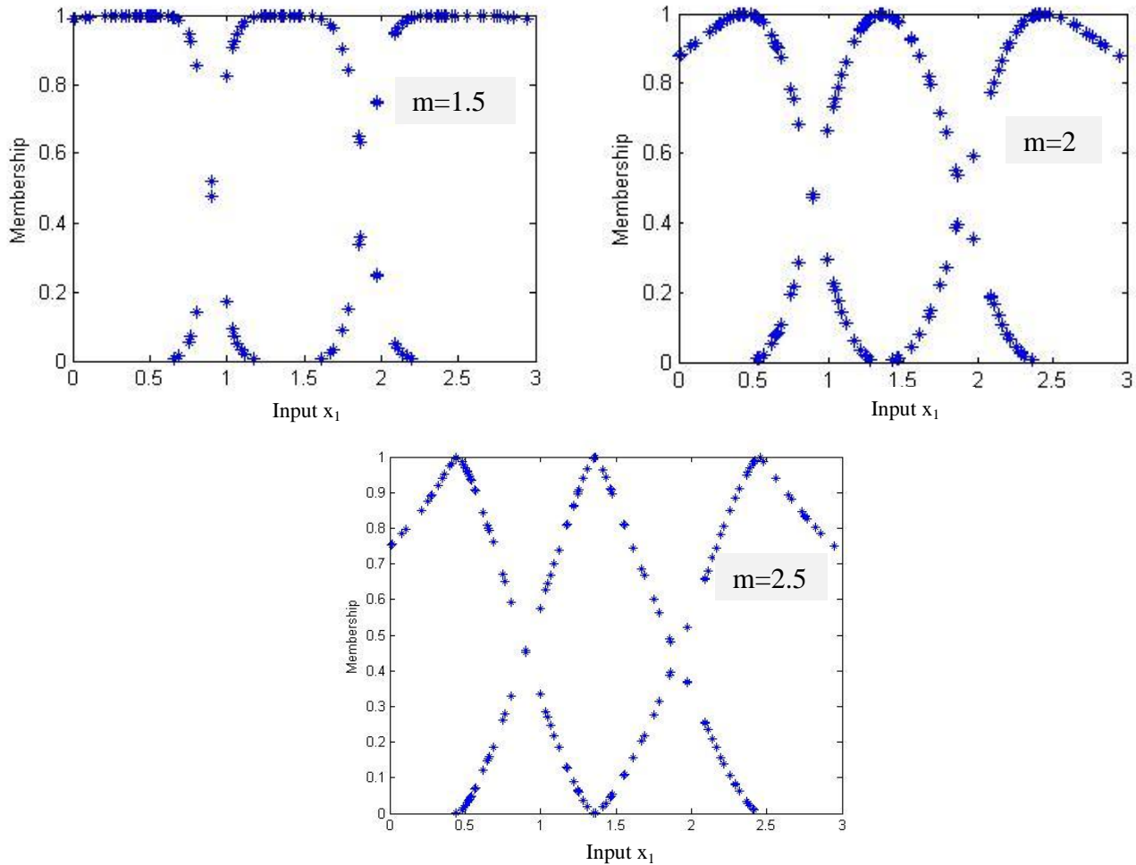
Figure 7.4. Membership Functions of x_1 , 0 \leq x_1 \leq 3 , m = (1.5, 2, 2.5) , c = 3 , FCM Iterations = 40
