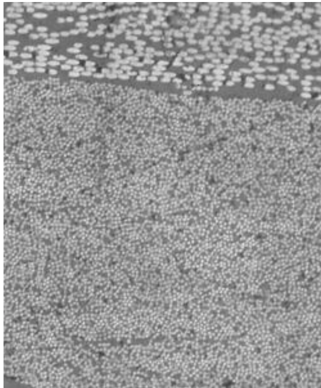
Figure 5.12 Optical Micrograph of 4-Tube Surface-Lock Braided Panel with SC-36 Resin
