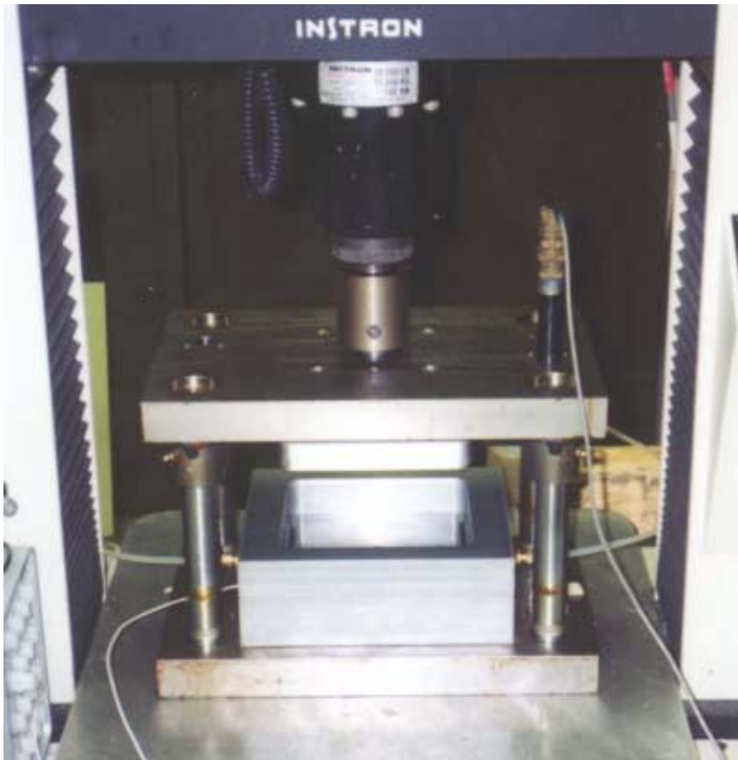
Figure 3.1 RTM In-Plane Fixture for Steady-State and Advancing Front Permeability
