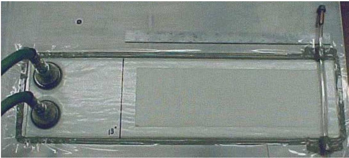
Figure 5.1 Experimental VARTM Processing Set-Up for a 10-ply, 1523 E-glass Composite Panel
