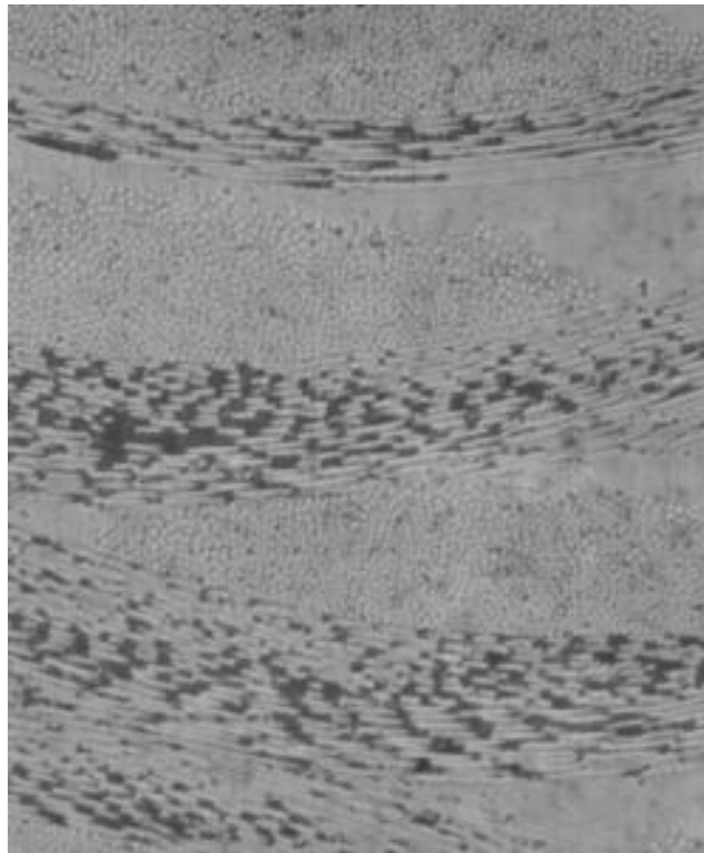
Figure 5.9 Optical Micrograph of 1523 E-glass/510A-40 Composite Panel
