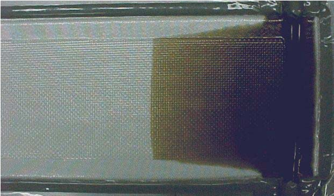
Figure 5.2 Resin enters high-permeable distribution medium.
