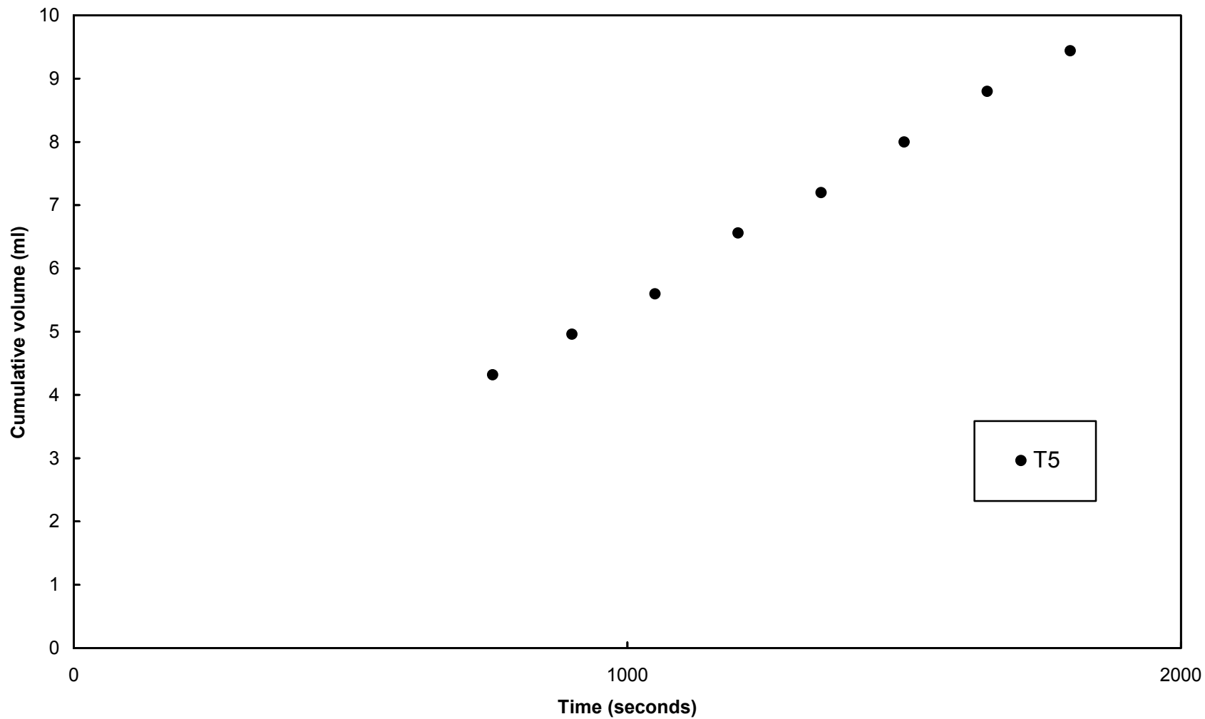
Figure A-15. Constant head piezometer test results, L3D2, W1
