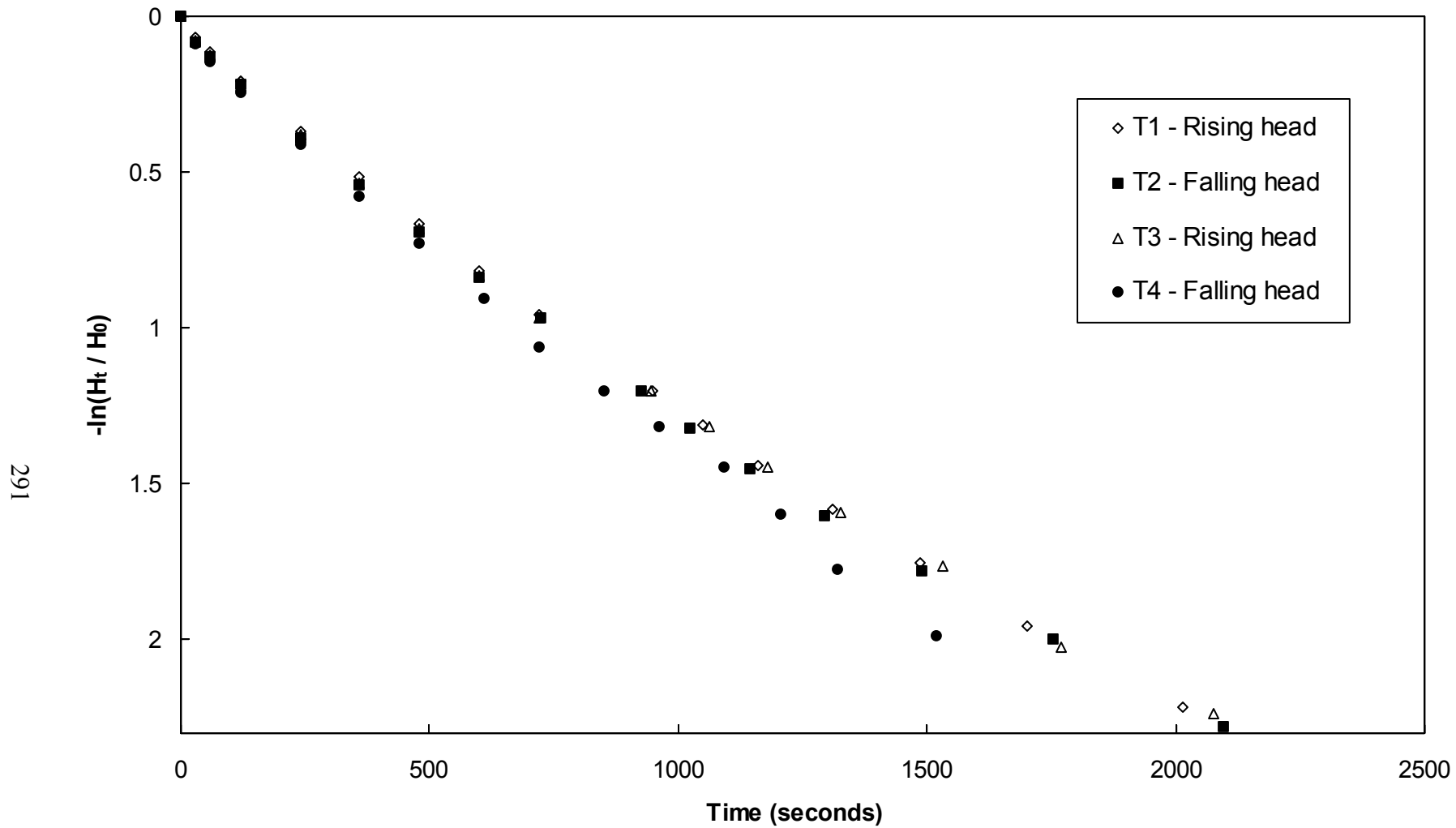
Figure A-20. Variable head piezometer test results, L1D2, W2
