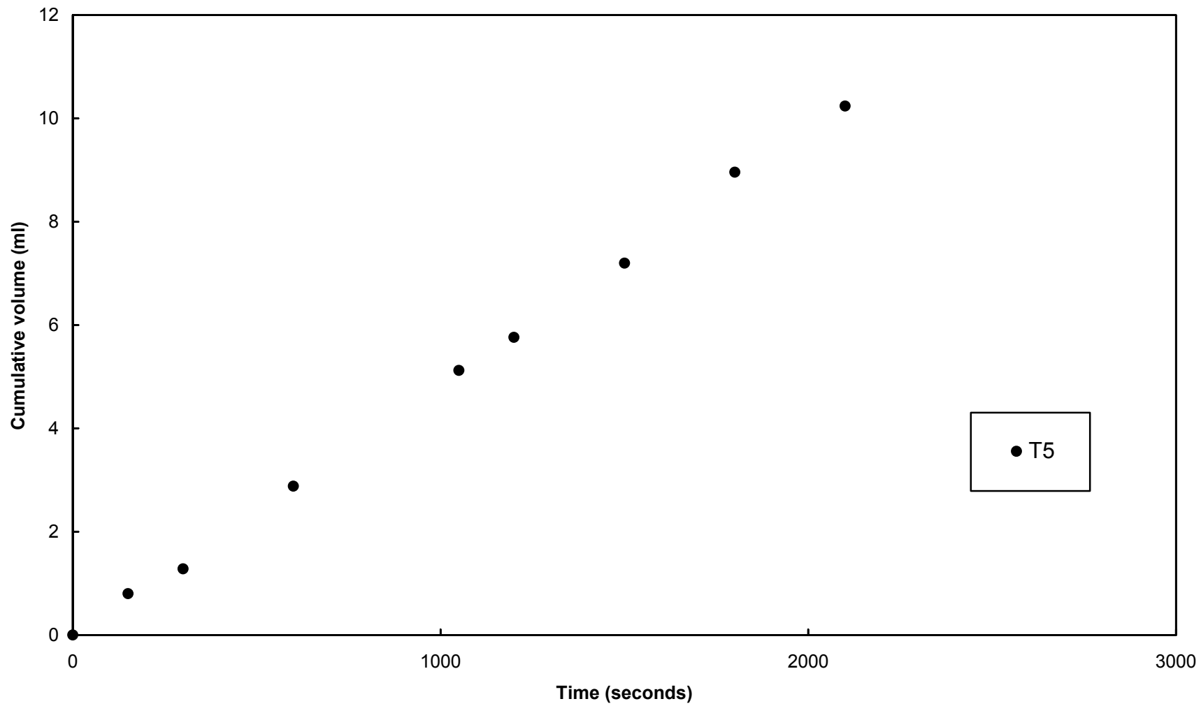
Figure A-17. Constant head piezometer test results, L3D3, W1
