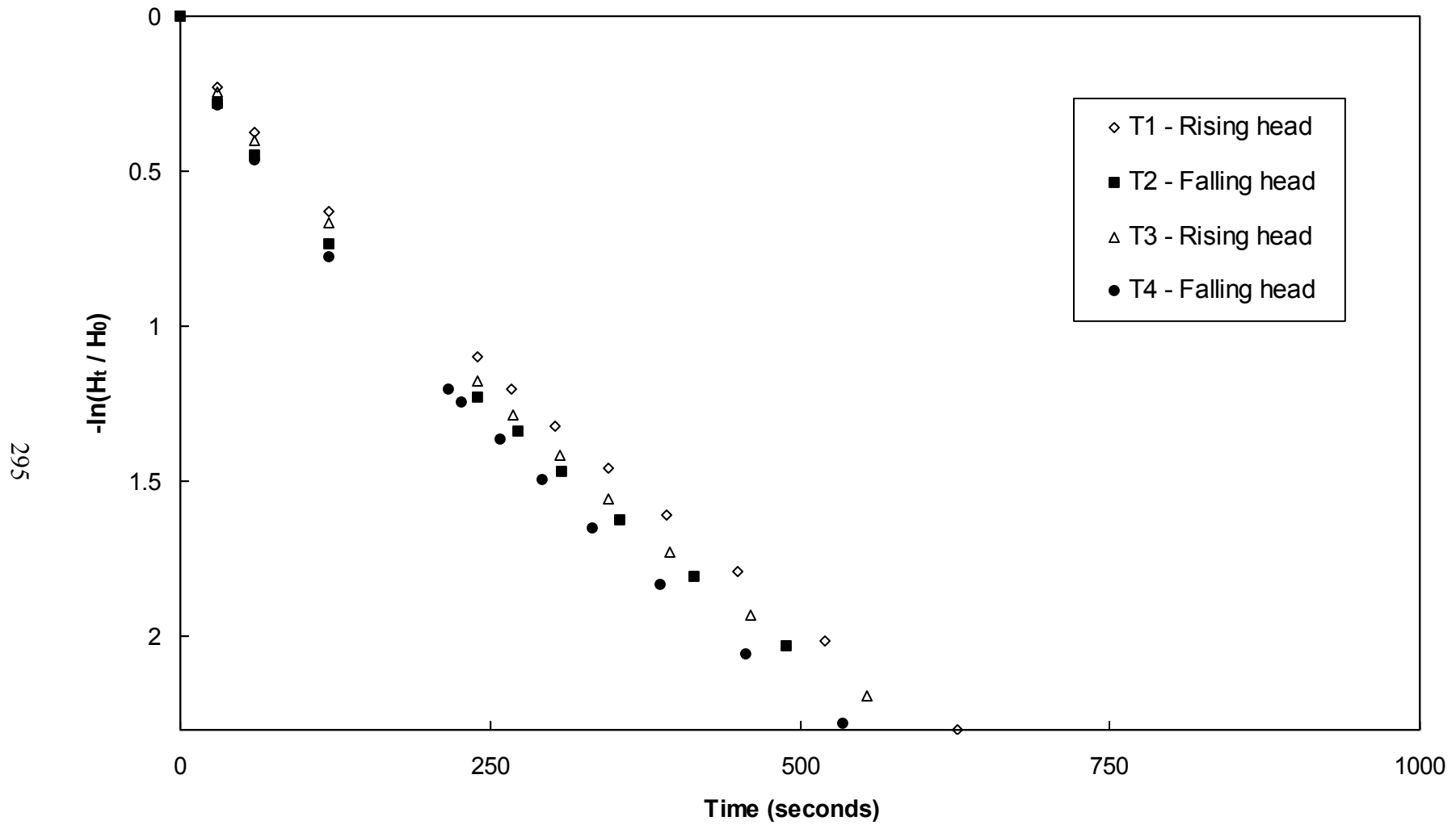
Figure A-24. Variable head piezometer test results, L2D3, W2
