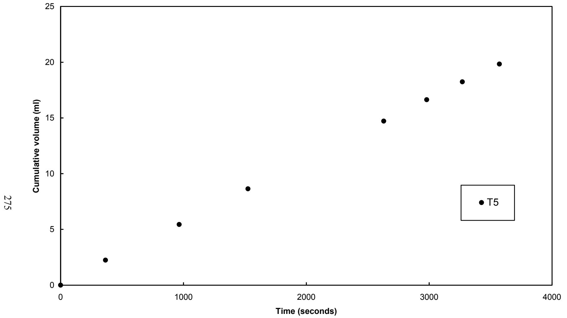
Figure A-4. Constant head piezometer test results, L1D2, W1
