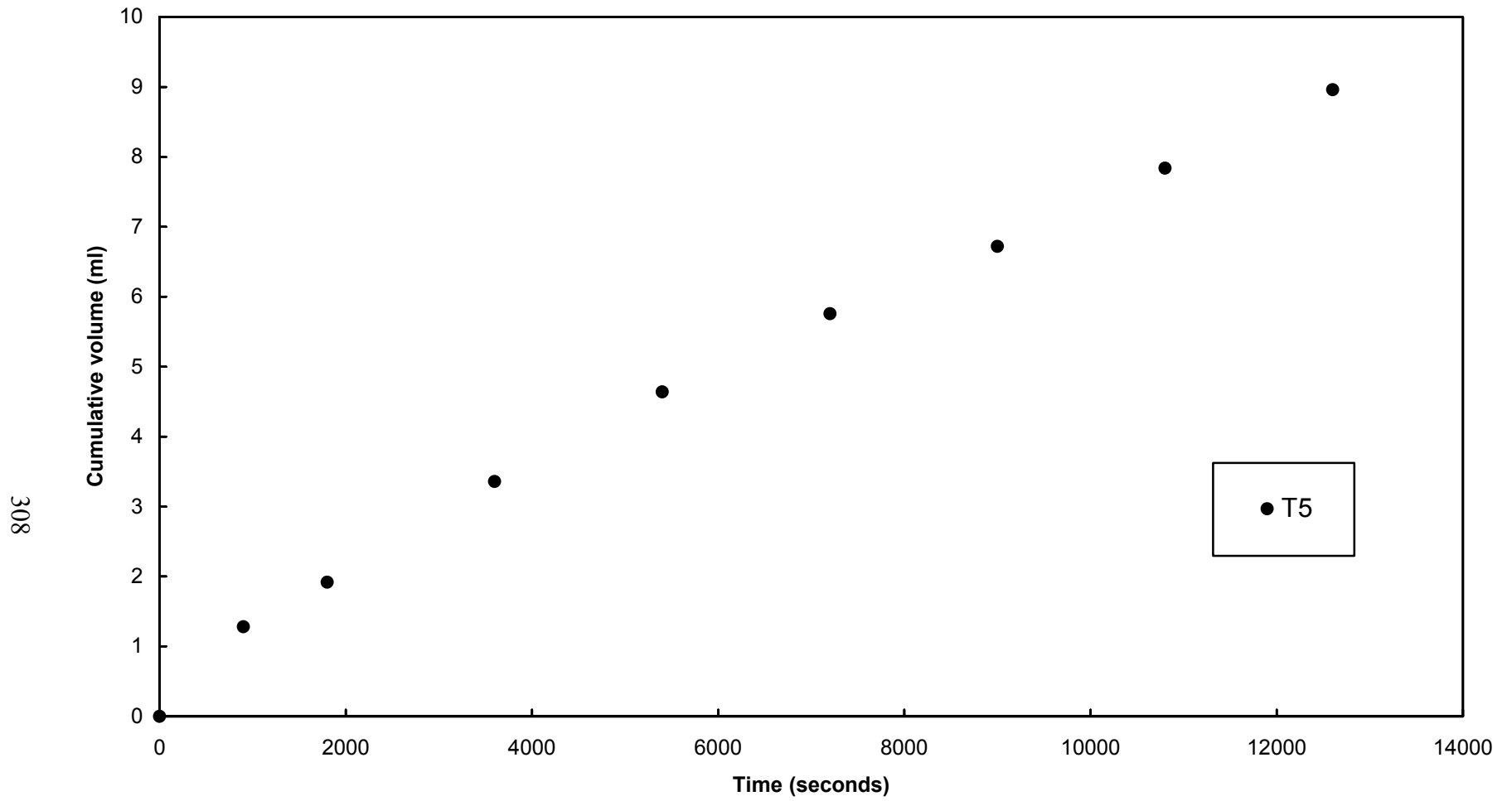
Figure A-37. Constant head piezometer test results, L2D2, W3
