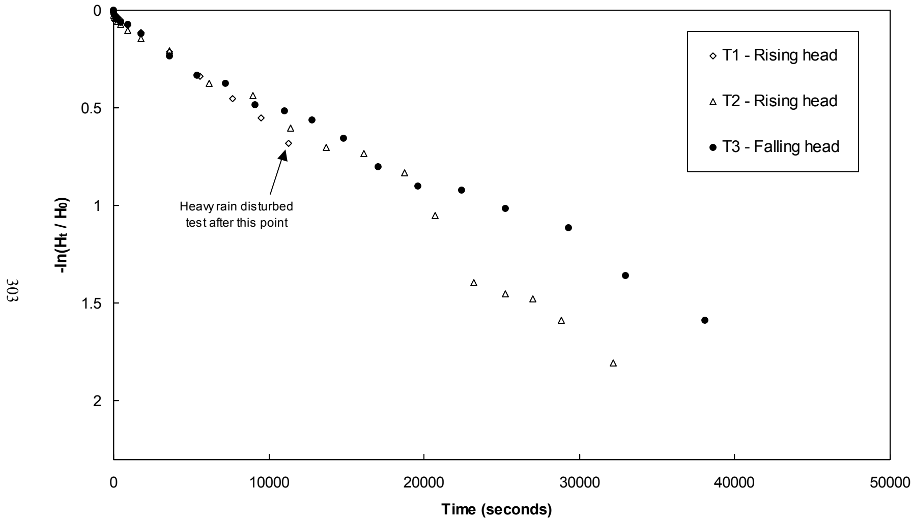
Figure A-32. Variable head piezometer test results, L1D2, W3
