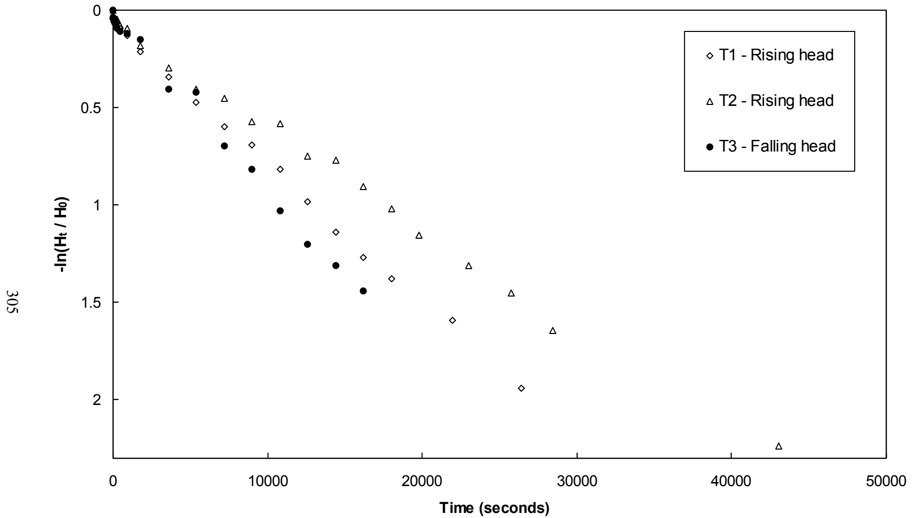
Figure A-34. Variable head piezometer test results, L2D1, W3
