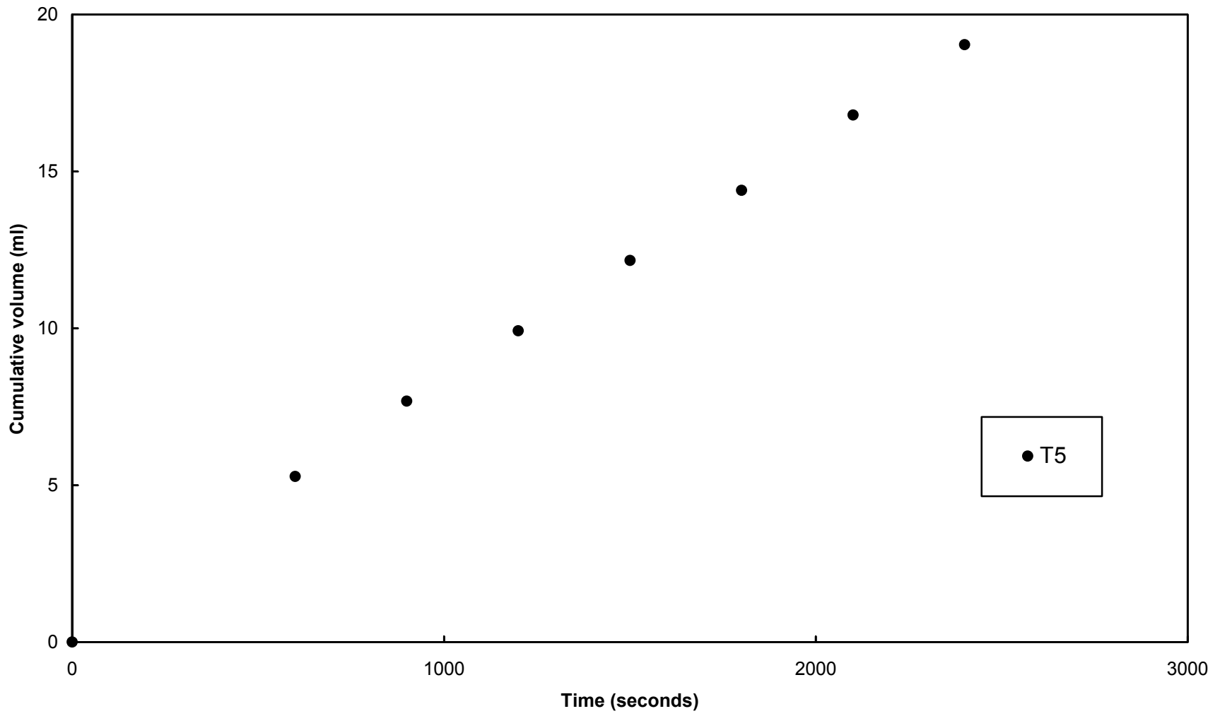
Figure A-21. Constant head piezometer test results, L1D2, W2
