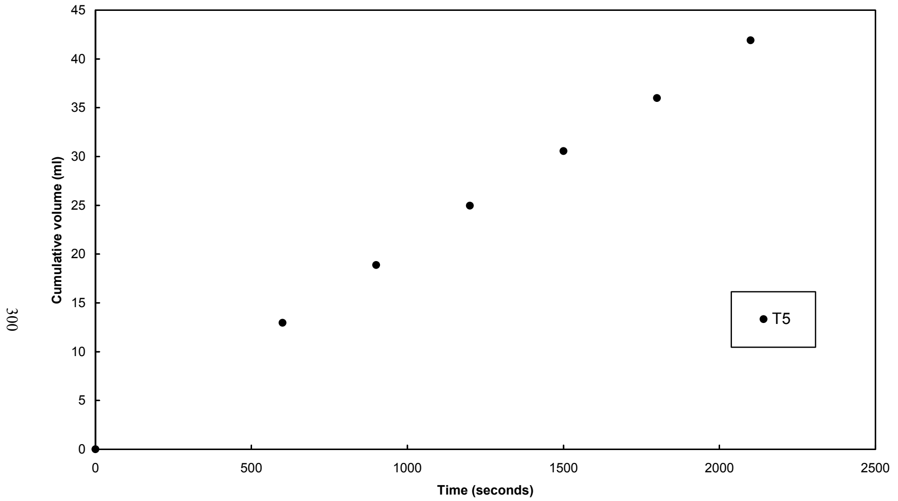
Figure A-29. Constant head piezometer test results, L3D2, W2
