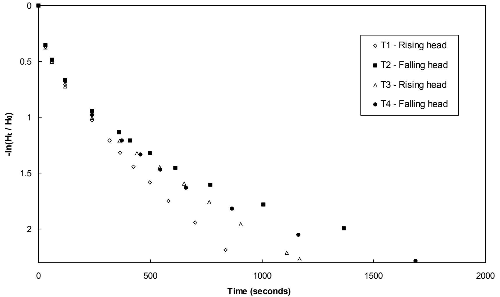
Figure A-26. Variable head piezometer test results, L3D1, W2
