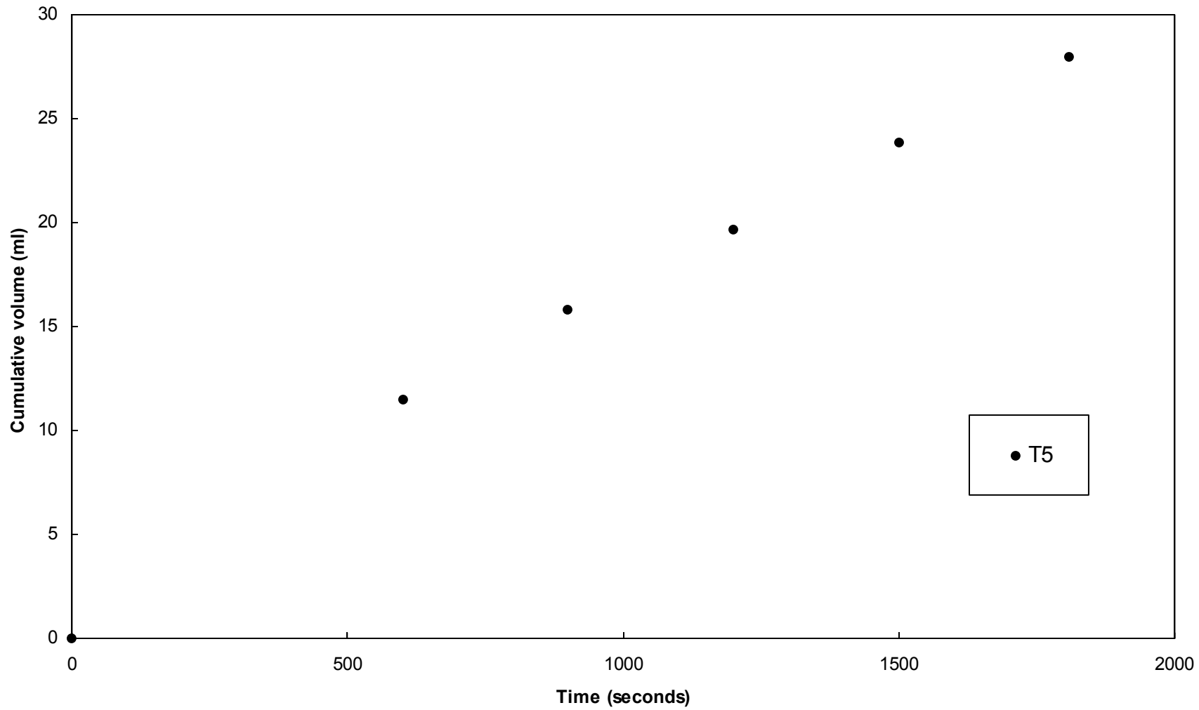
Figure A-27. Constant head piezometer test results, L3D1, W2
