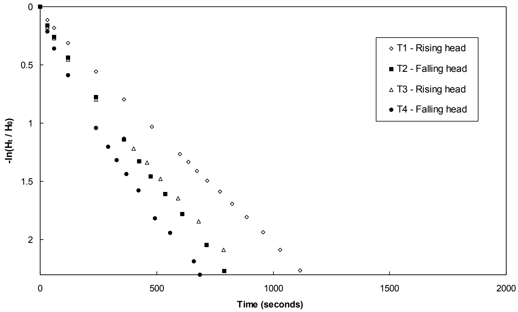
Figure A-22. Variable head piezometer test results, L1D3, W2
