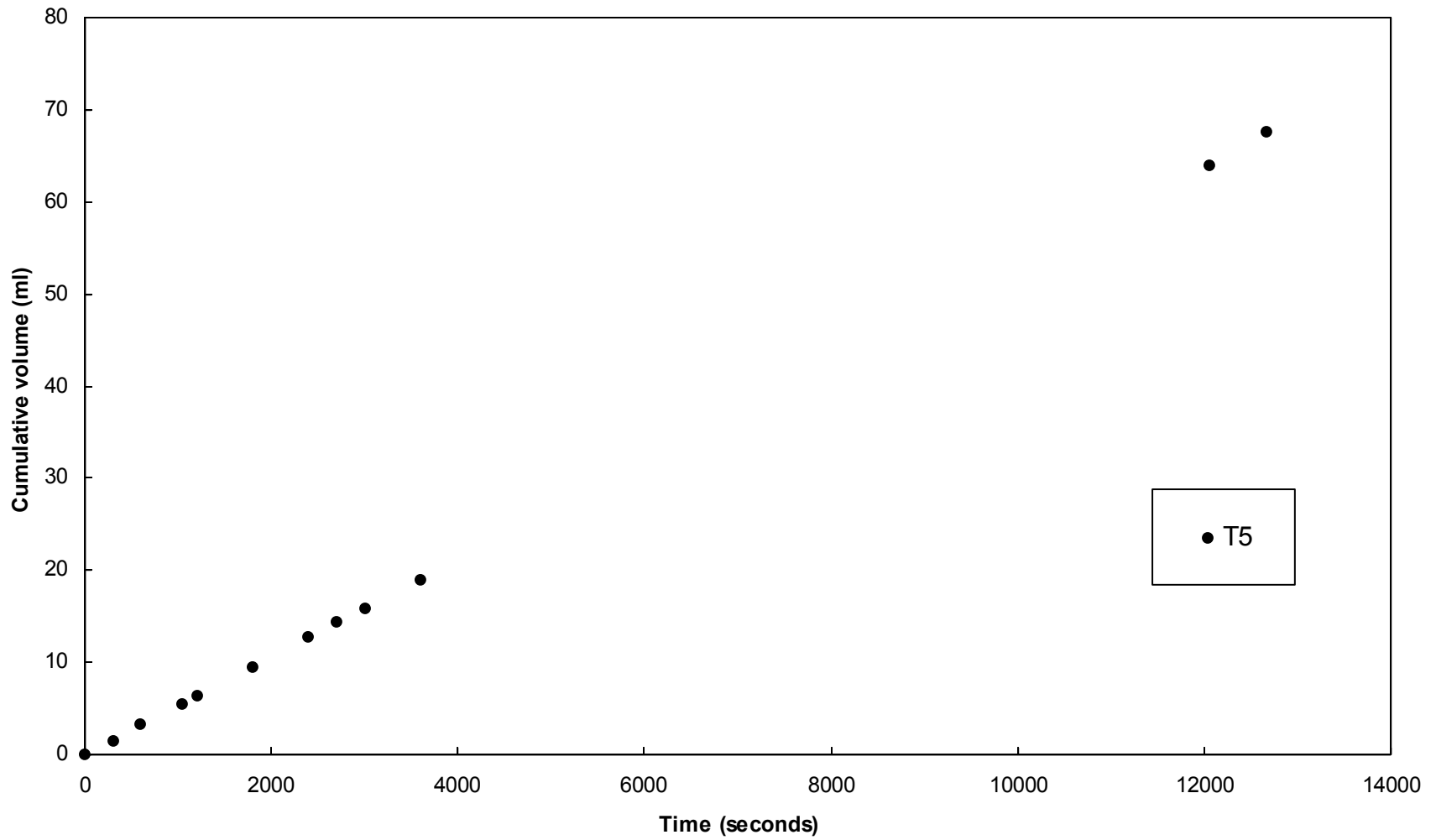
Figure A-2. Constant head piezometer test results, L1D1, W1
