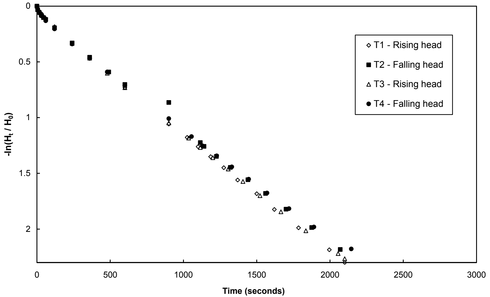
Figure A-3. Variable head piezometer test results, L1D2, W1
