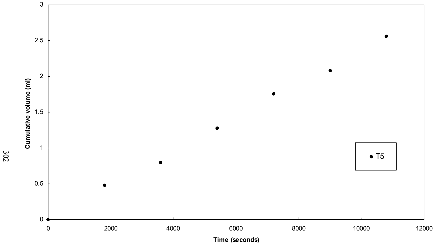
Figure A-31. Constant head piezometer test results, L1D1, W3
