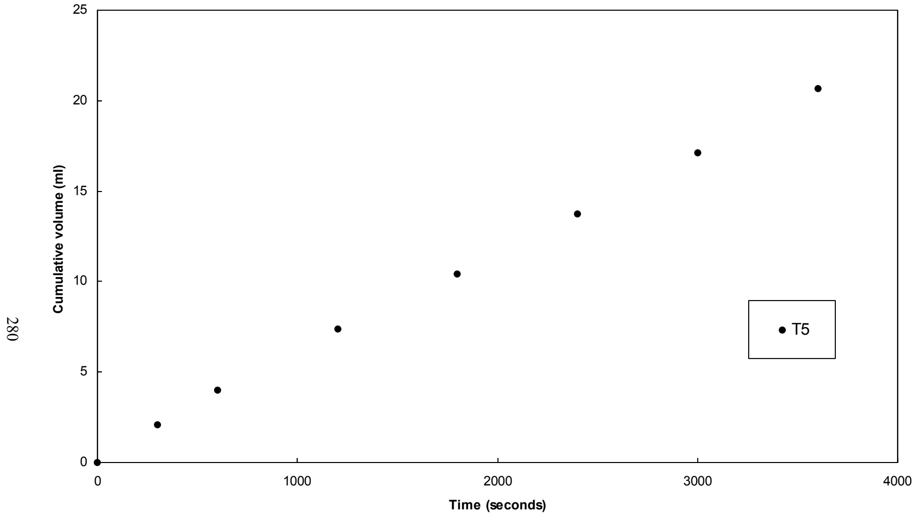
Figure A-9. Constant head piezometer test results, L2D1, W1
