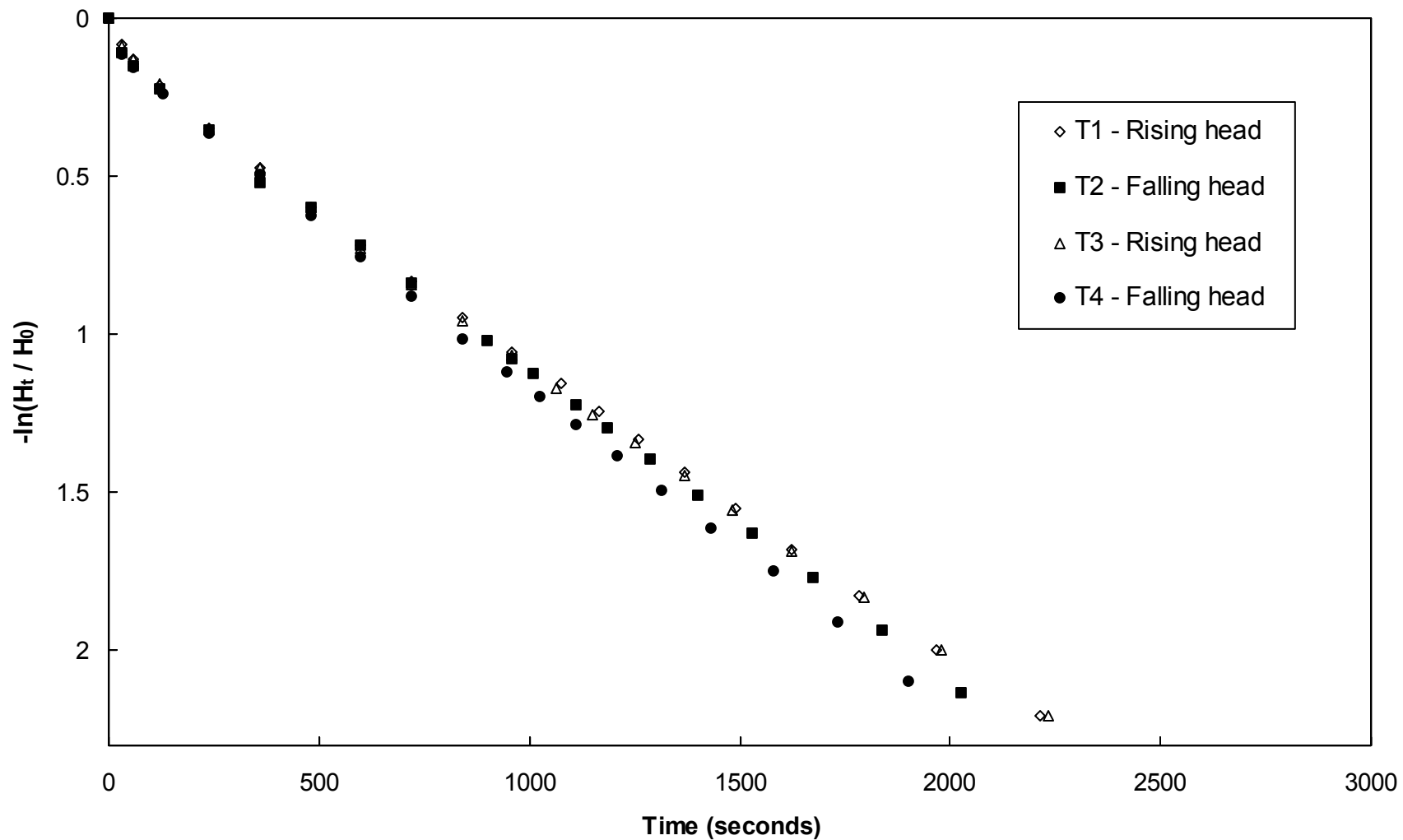
Figure A-14. Variable head piezometer test results, L3D2, W1
