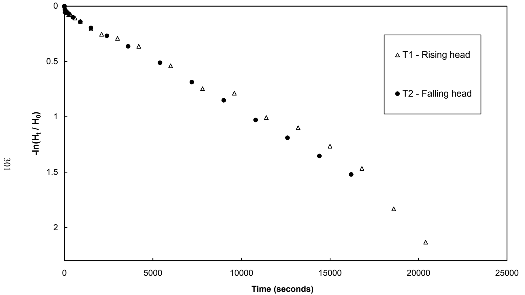
Figure A-30. Variable head piezometer test results, L1D1, W3
