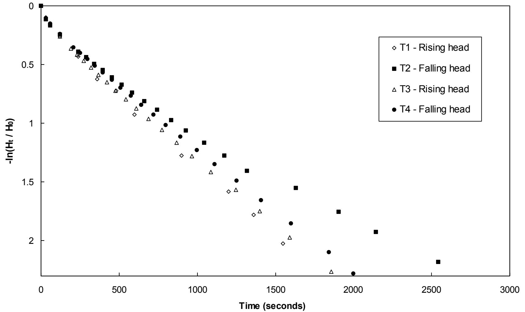
Figure A-8. Variable head piezometer test results, L2D1, W1
