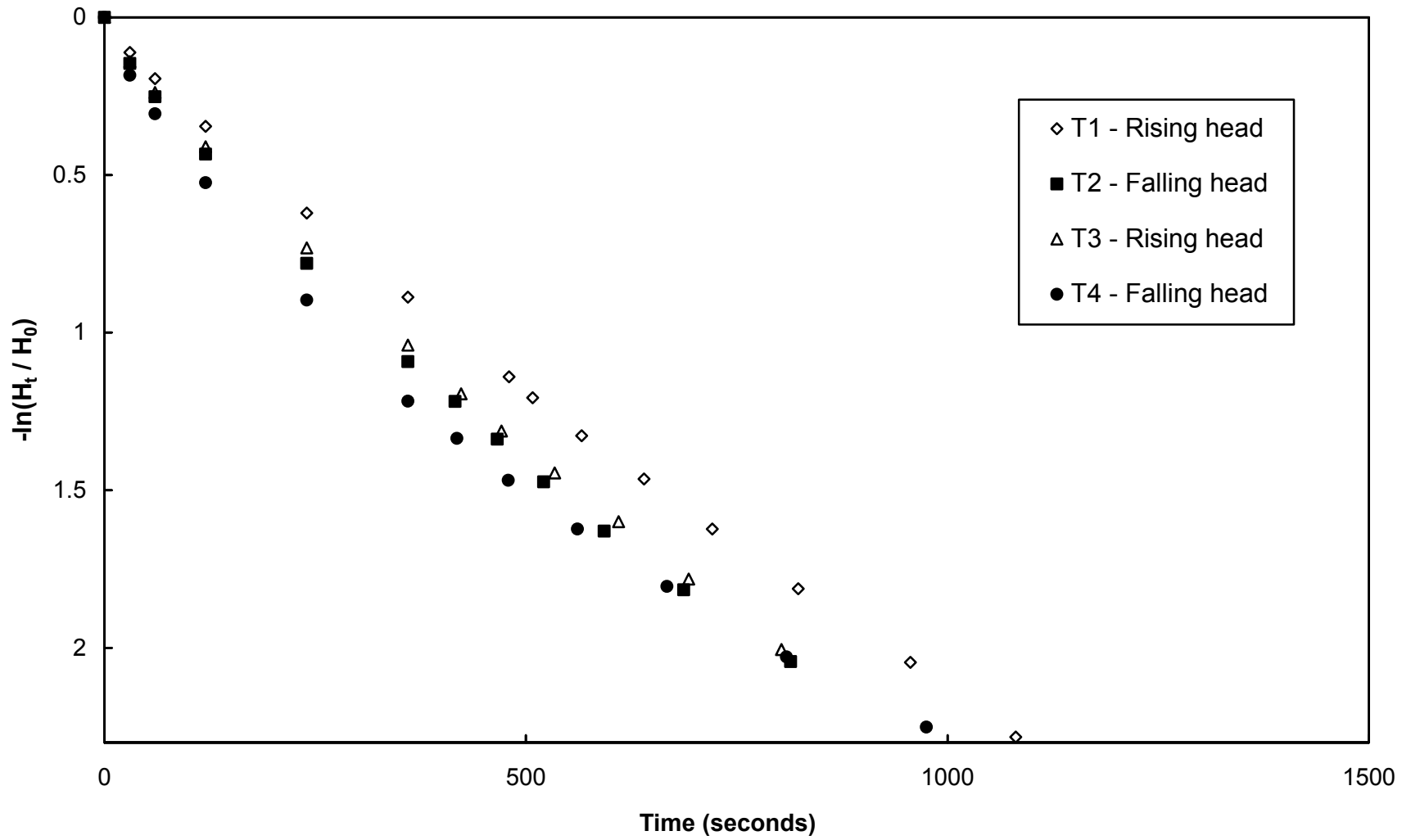
Figure A-28. Variable head piezometer test results, L3D2, W2
