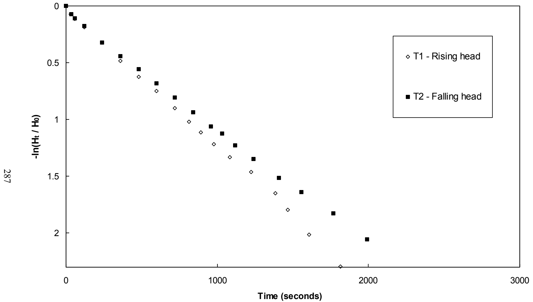
Figure A-16. Variable head piezometer test results, L3D3, W1
