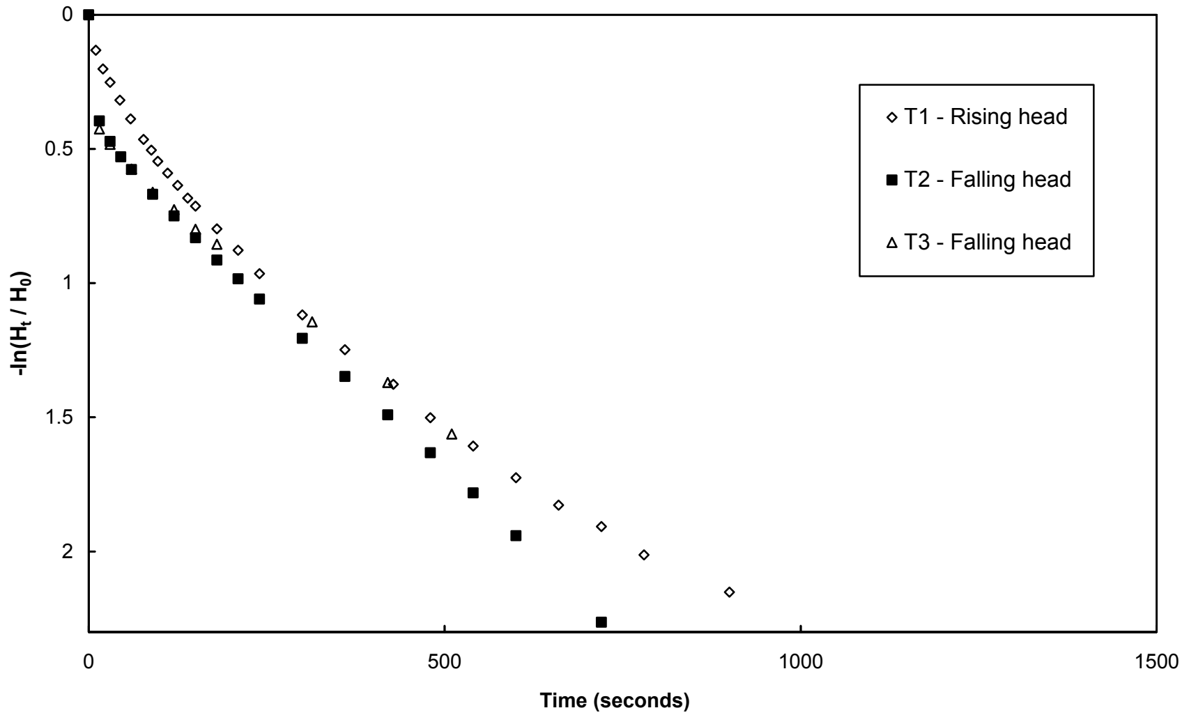
Figure A-6. Variable head piezometer test results, L1D4, W1
