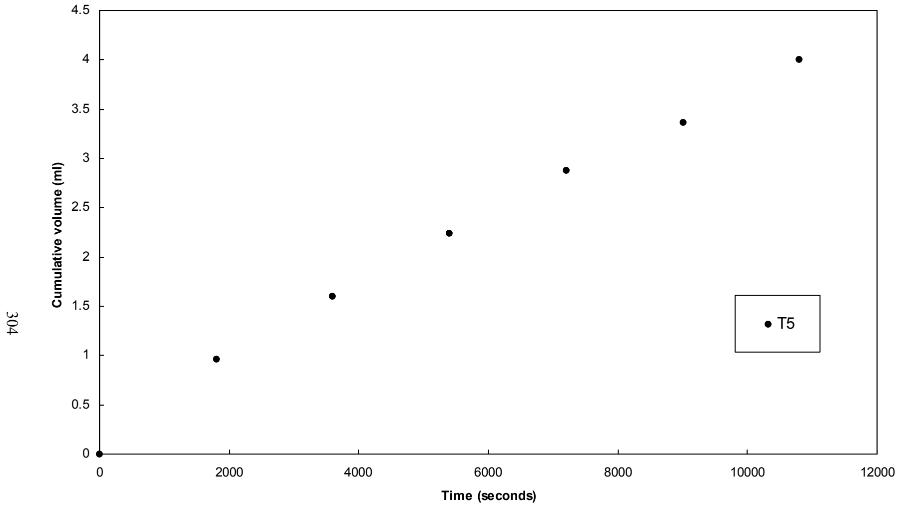
Figure A-33. Constant head piezometer test results, L1D2, W3
