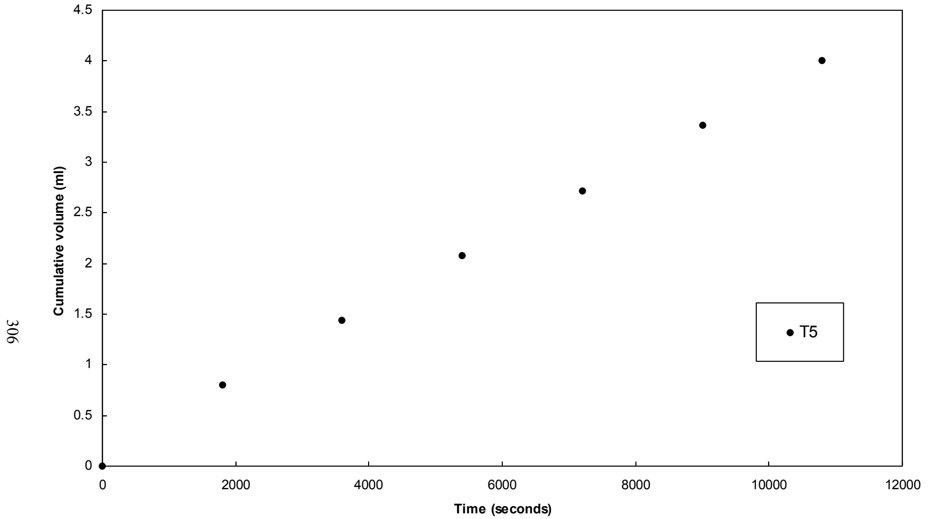
Figure A-35. Constant head piezometer test results, L2D1, W3
