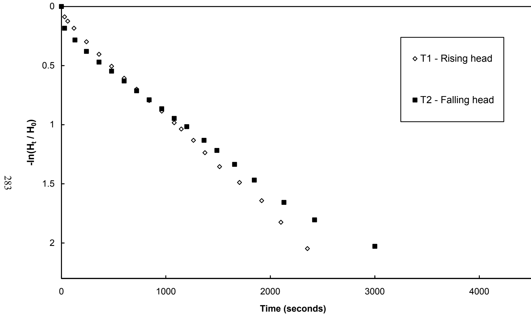
Figure A-12. Variable head piezometer test results, L3D1, W1
