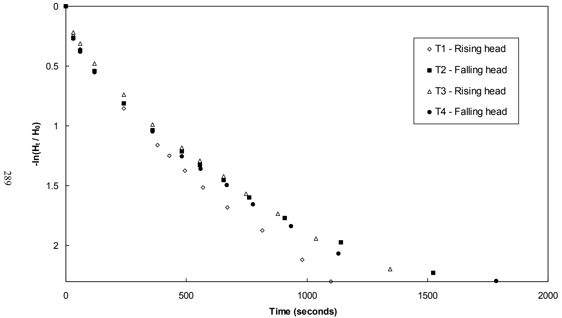
Figure A-18. Variable head piezometer test results, L1D1, W2
