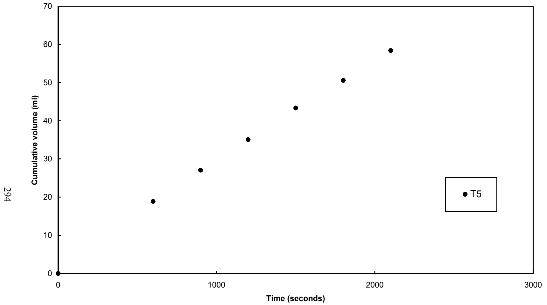
Figure A-23. Constant head piezometer test results, L1D3, W2
