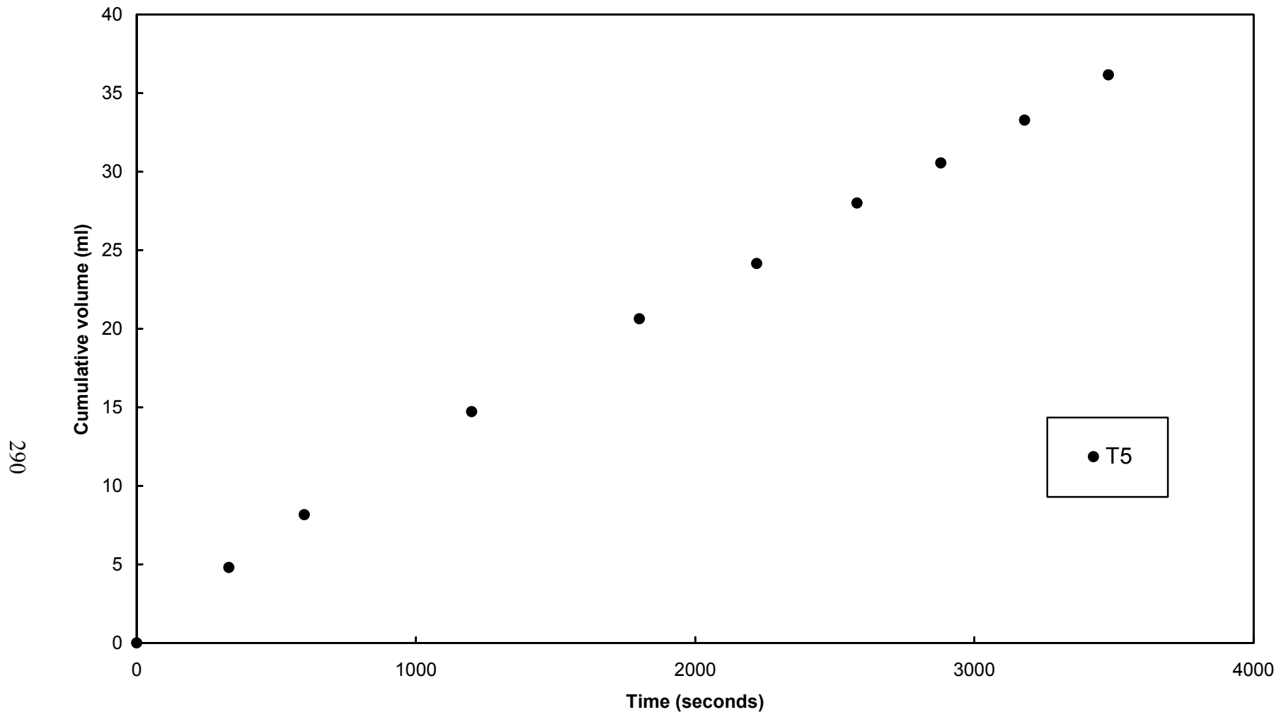
Figure A-19. Constant head piezometer test results, L1D1, W2
