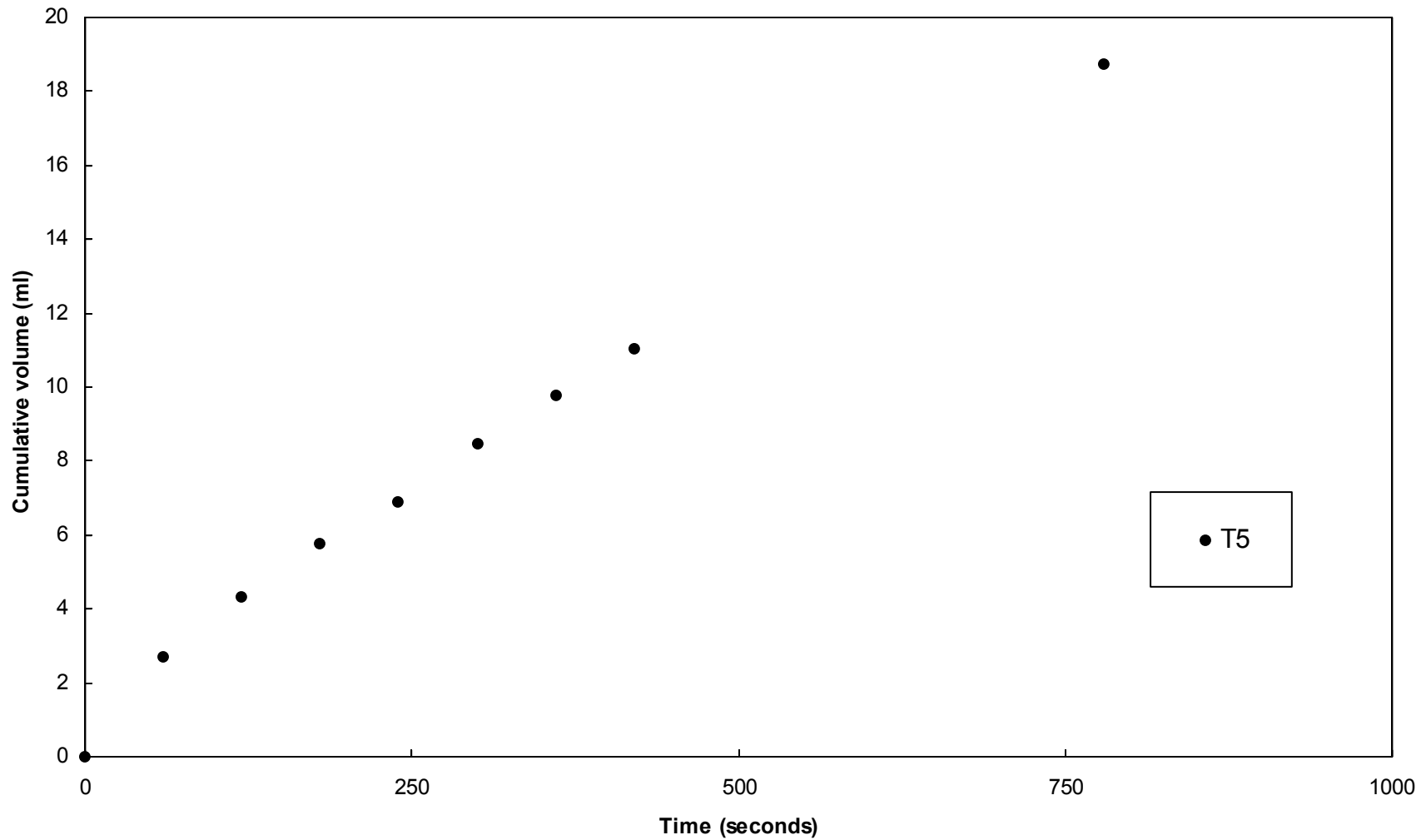
Figure A-7. Constant head piezometer test results, L1D4, W1
