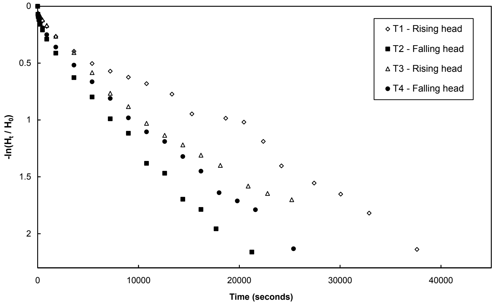
Figure A-36. Variable head piezometer test results, L2D2, W3
