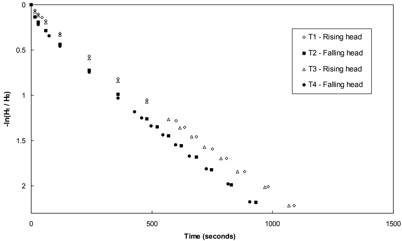
Figure A-10. Variable head piezometer test results, L2D3, W1
