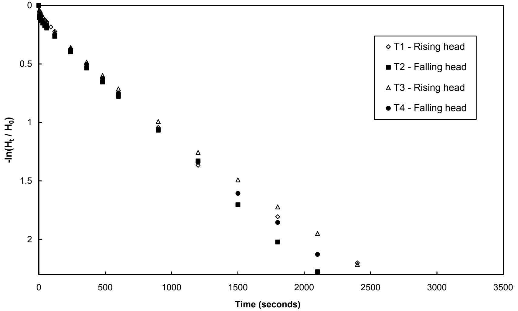
Figure A-1. Variable head piezometer test results, L1D1, W1
