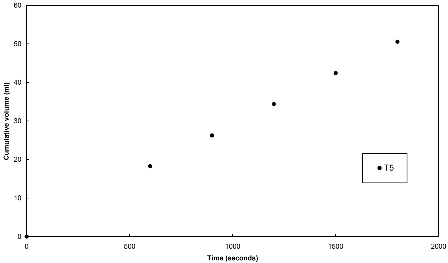
Figure A-25. Constant head piezometer test results, L2D3, W2
