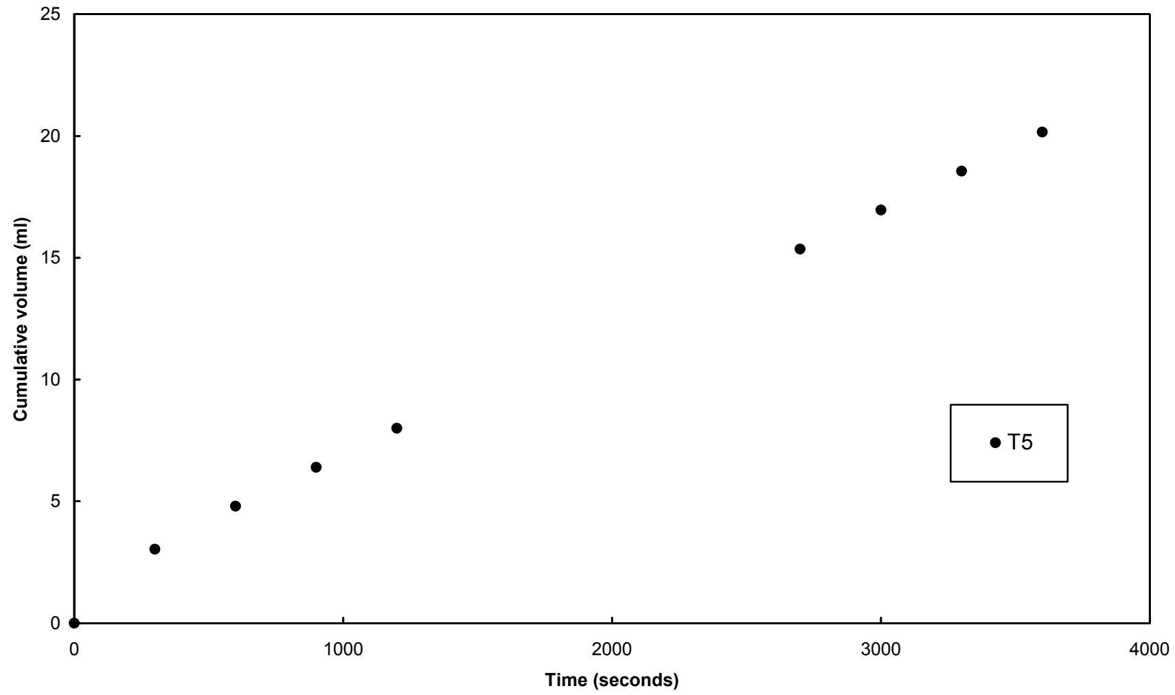
Figure A-13. Constant head piezometer test results, L3D1, W1
