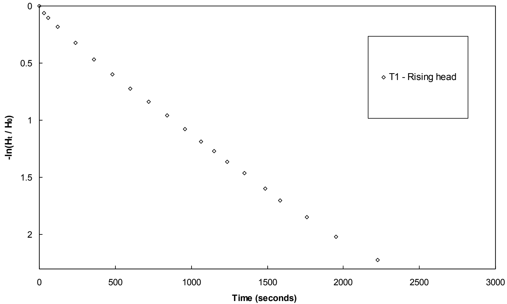
Figure A-5. Variable head piezometer test results, L1D3, W1
