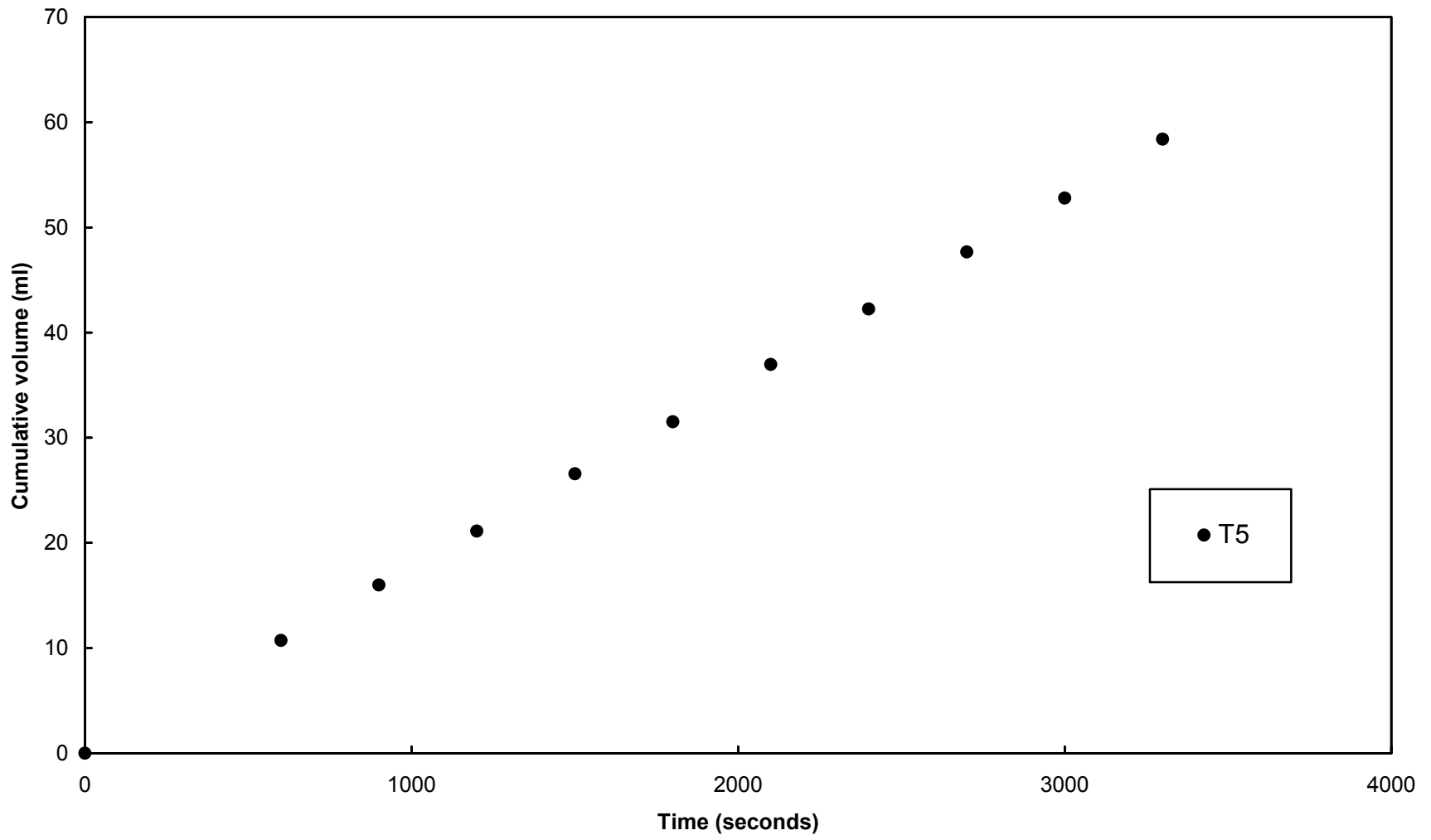
Figure A-11. Constant head piezometer test results, L2D3, W1
