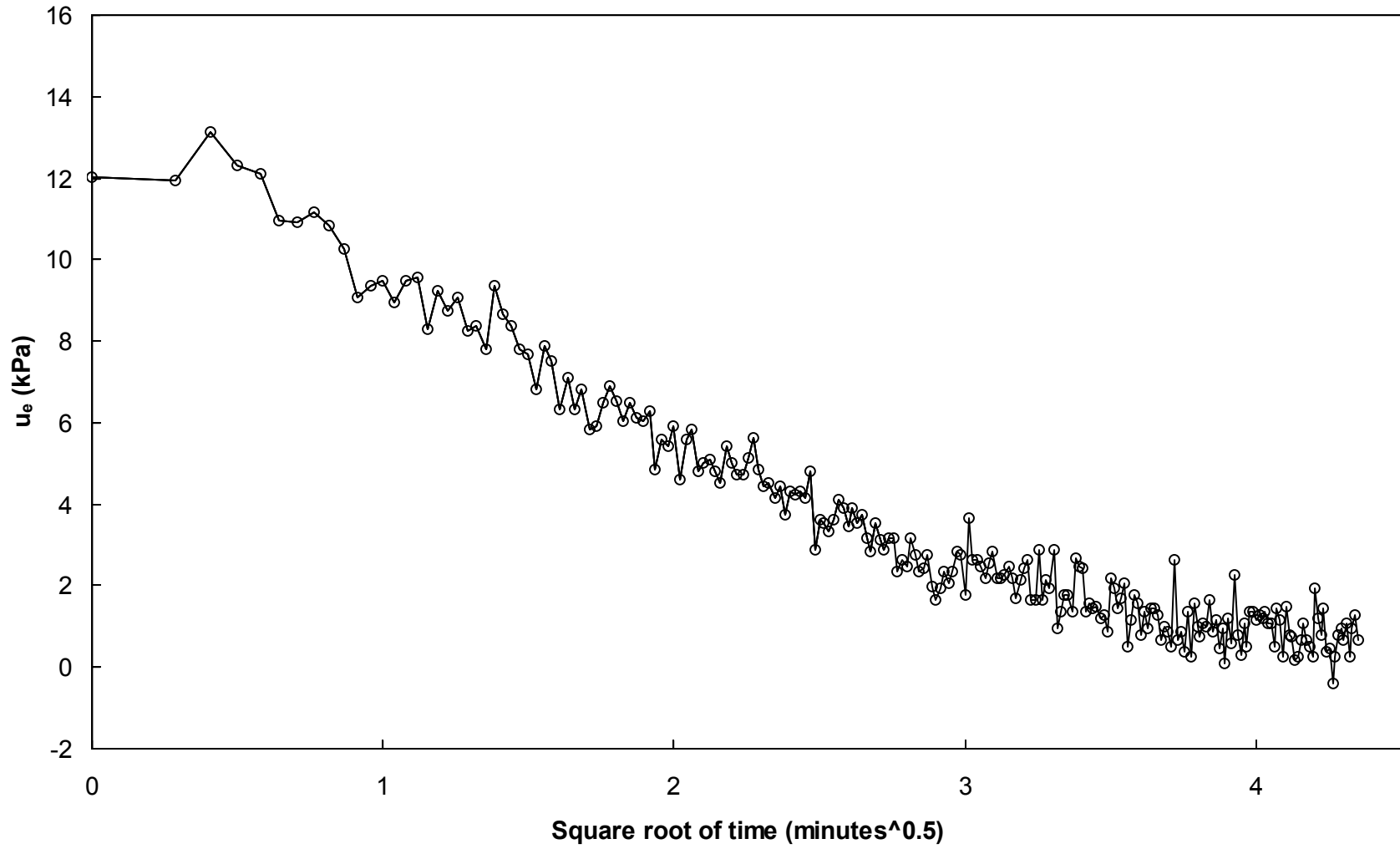
Figure B-4. Dissipation test data for P5 in W1
