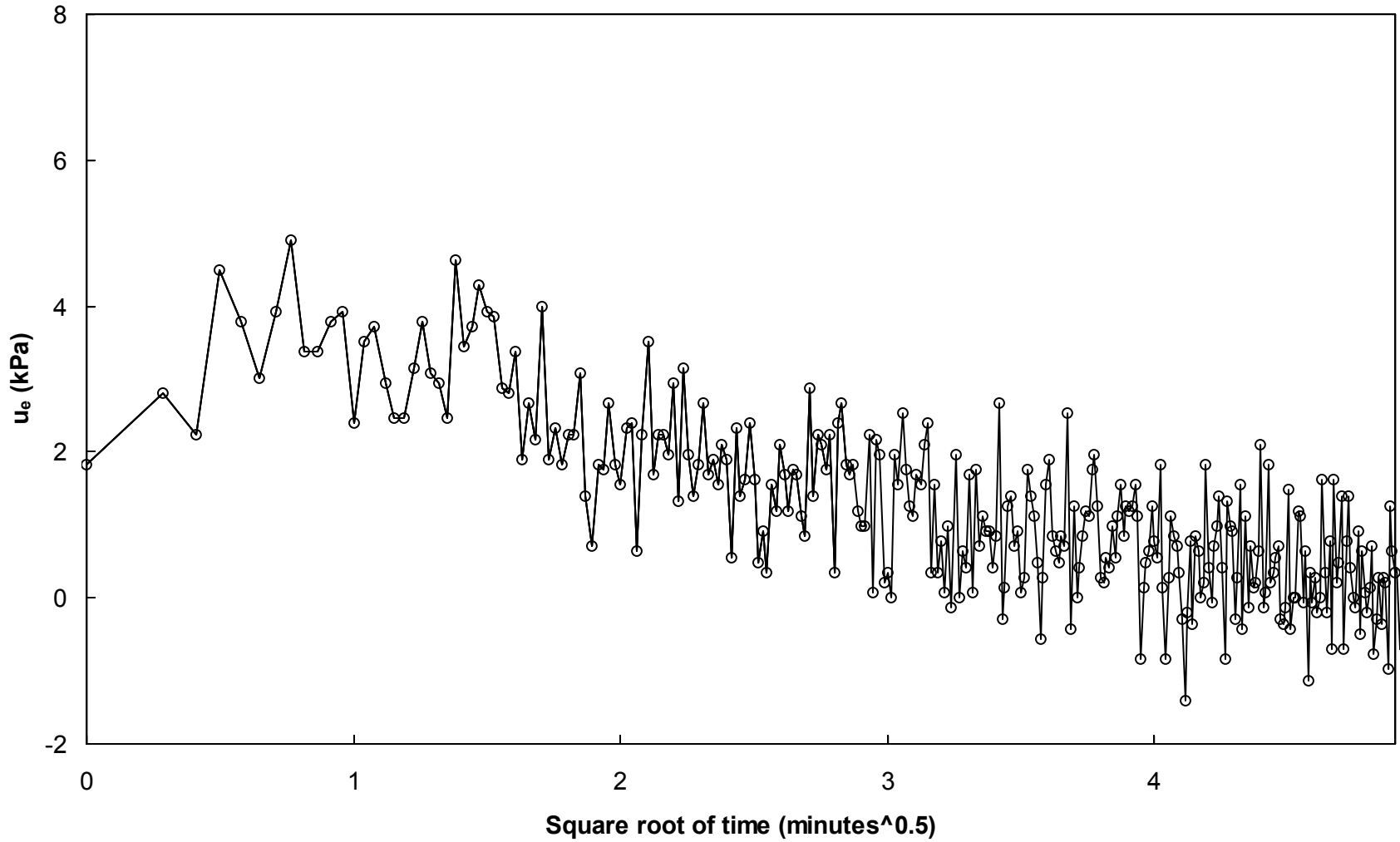
Figure B-1. Dissipation test data for P1 in W1
