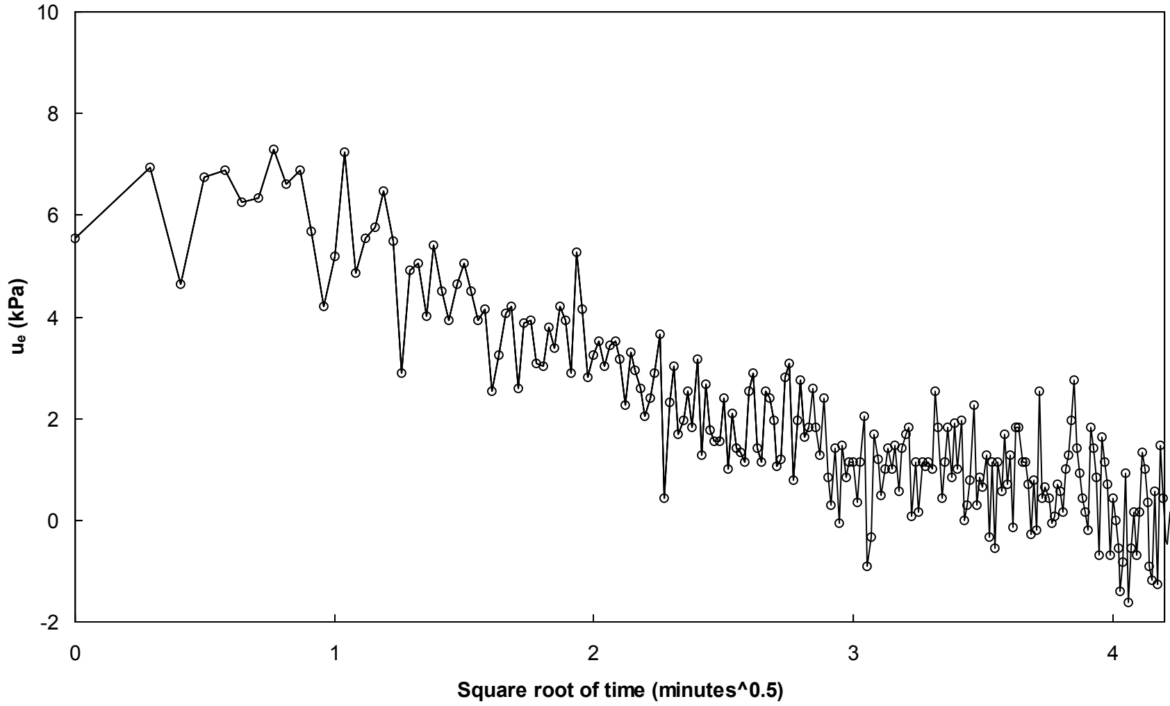
Figure B-2. Dissipation test data for P2 in W1
