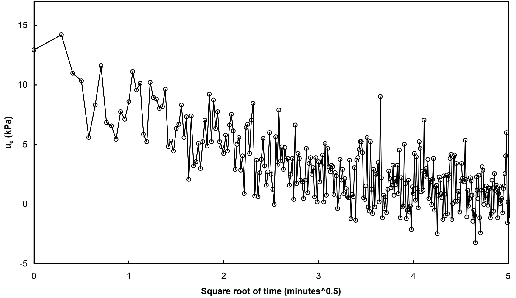
Figure B-3. Dissipation test data for P3 in W1
