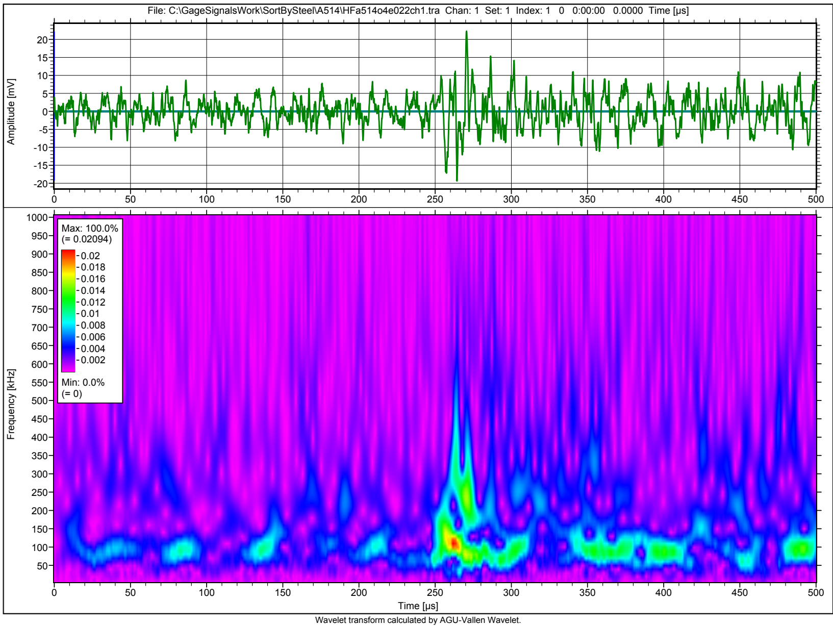
A514, overload 4, event @022 ms, channels 1 and 2
