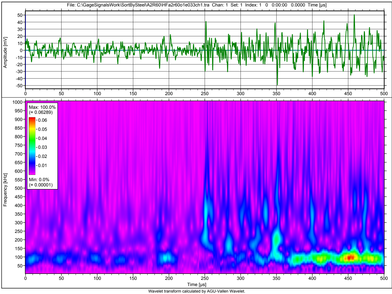
A2r60, overload 1, event @033 ms, channels 1 and 2
