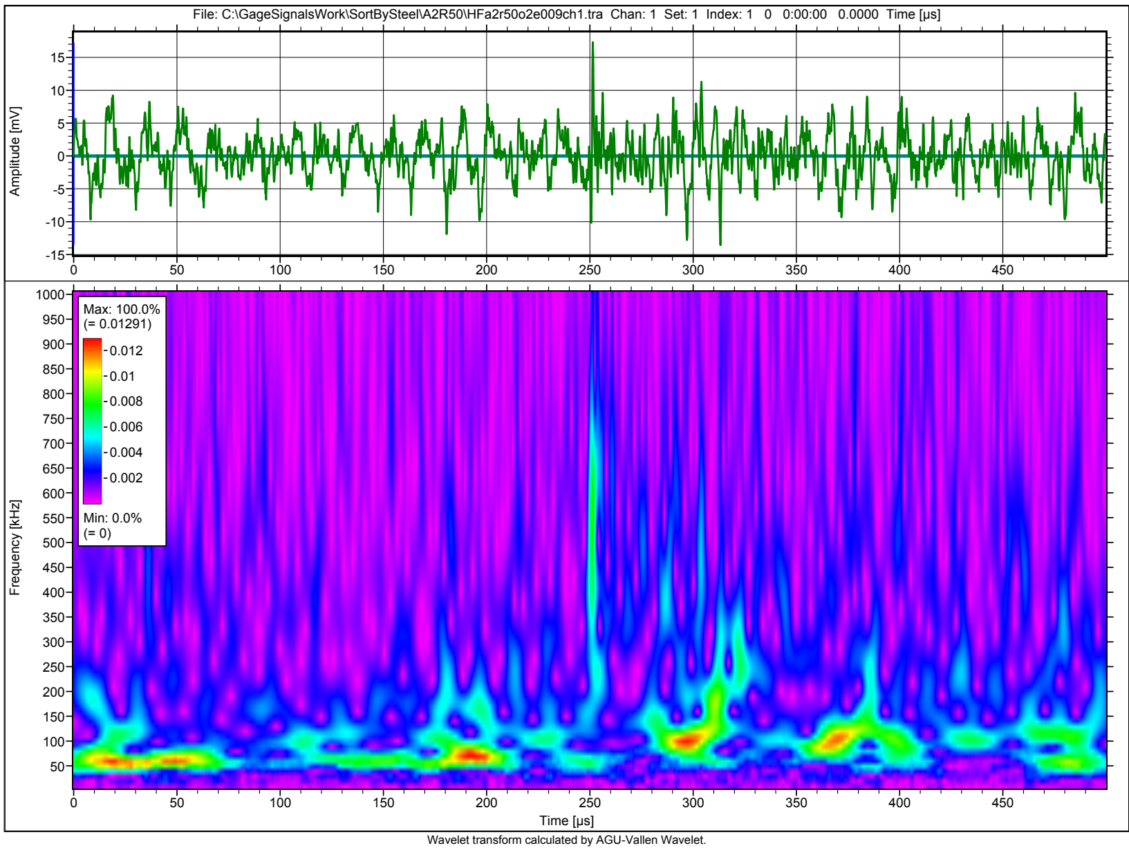
A2r50, overload 2, event @009 ms, channels 1 and 2
