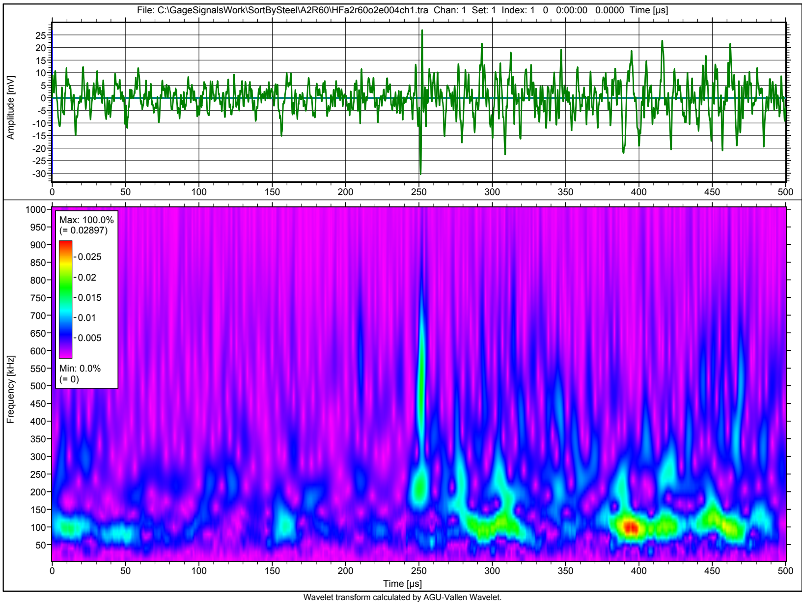
A2r60, overload 2, event @004 ms, channels 1 and 2
