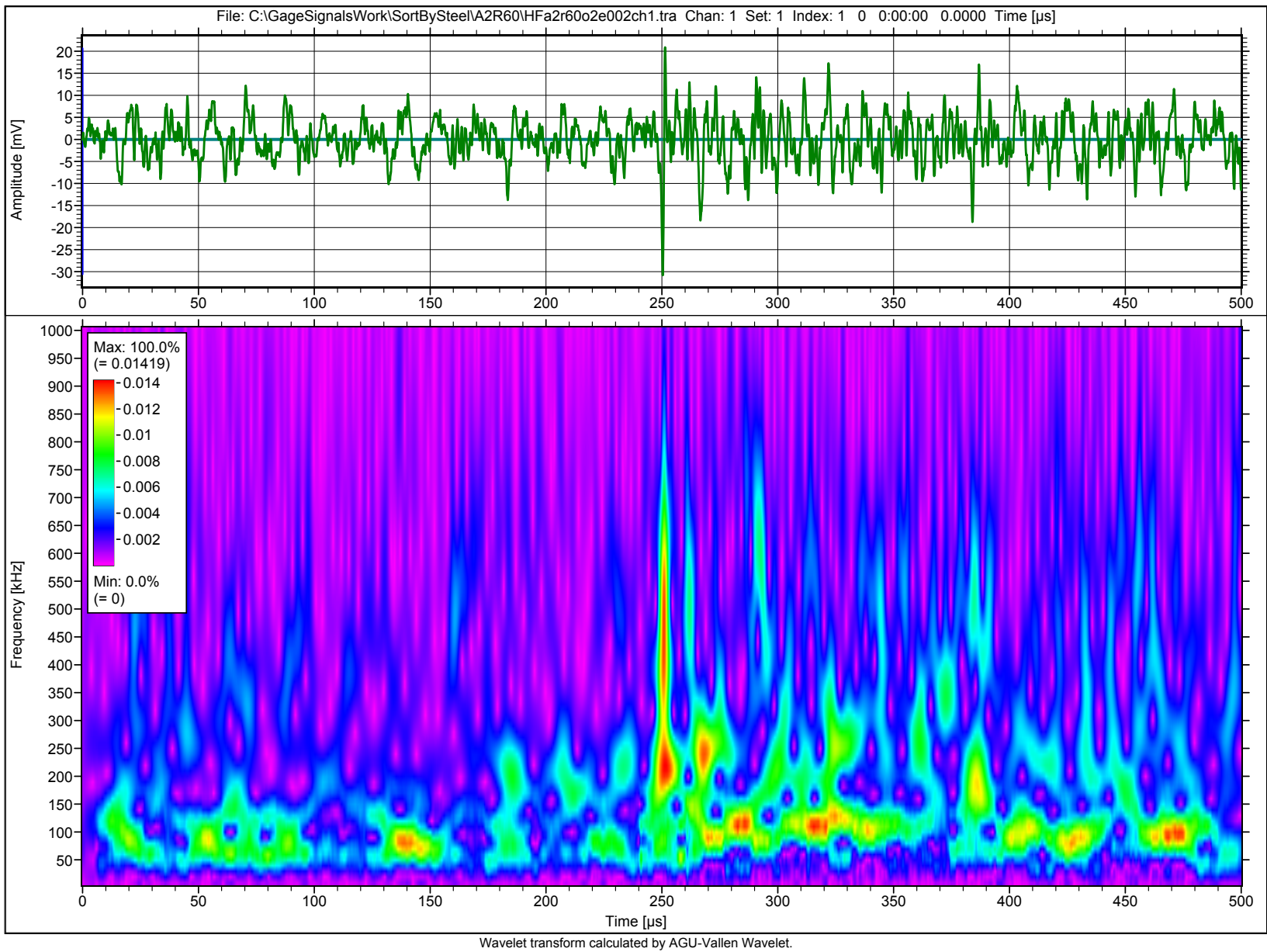
A2r60, overload 2, event @002 ms, channels 1 and 2
