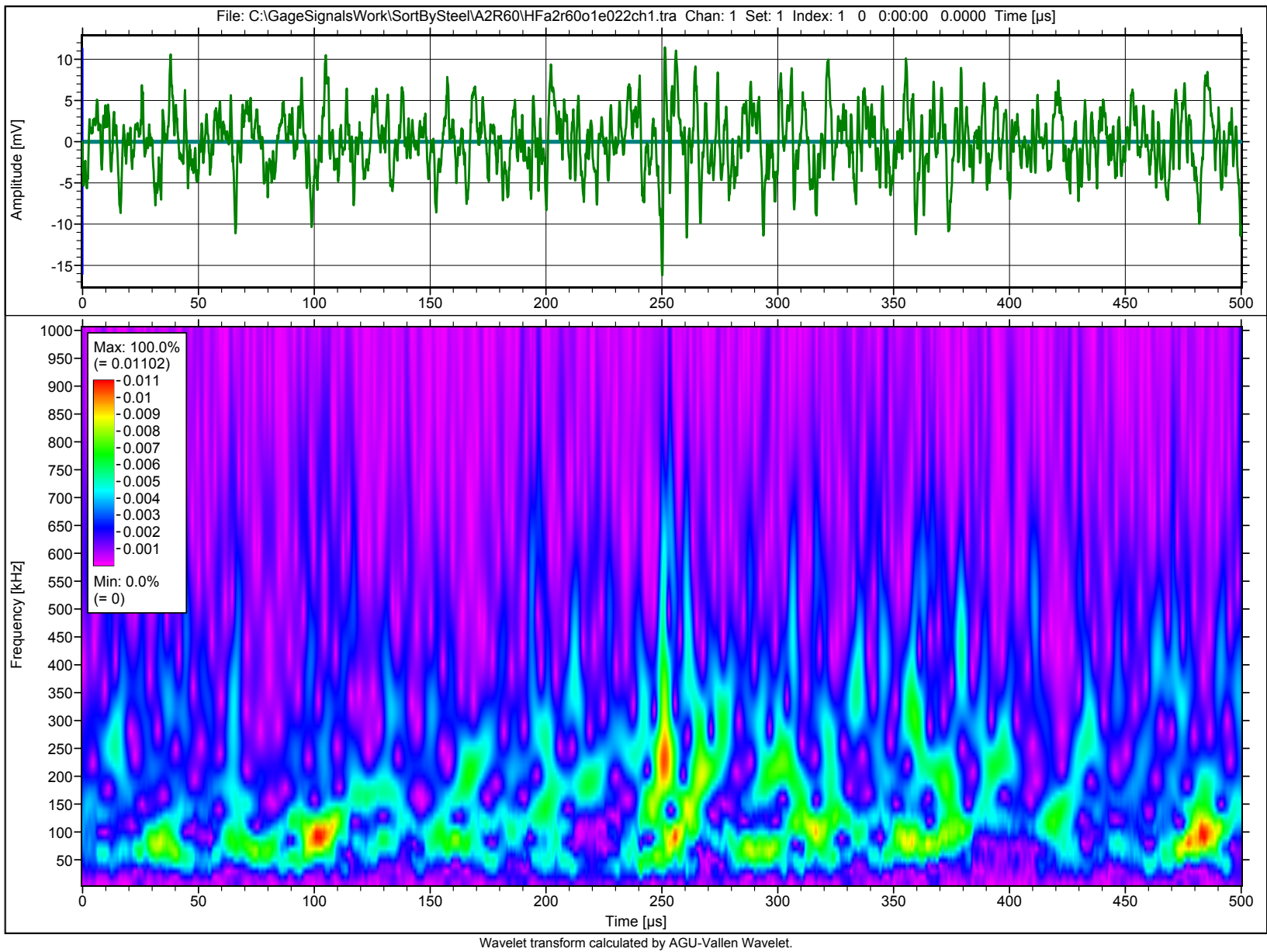
A2r60, overload 1, event @022 ms, channels 1 and 2
