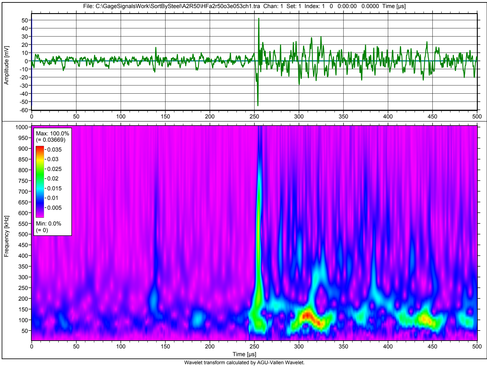
A2r50, overload 3, event @053 ms, channels 1 and 2
