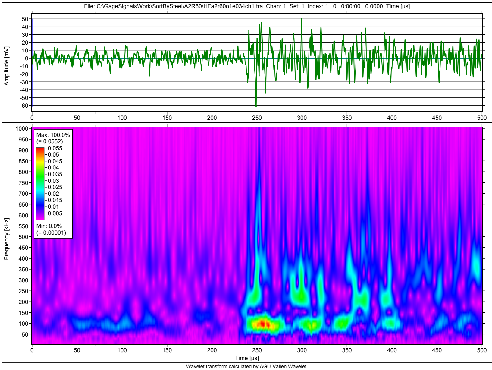
A2r60, overload 1, event @034 ms, channels 1 and 2
