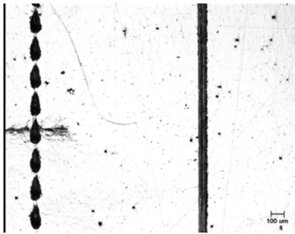
A36, after overload 4, flat
