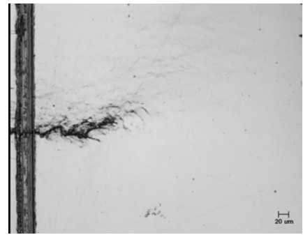
A514, after overload 7, flat
