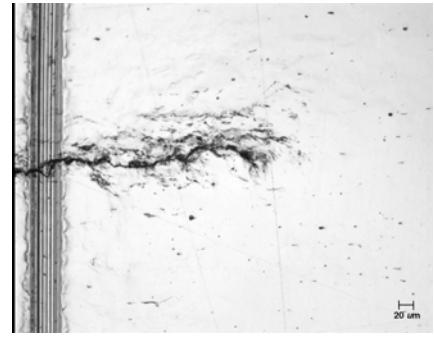
1018, after overload 5, flat
