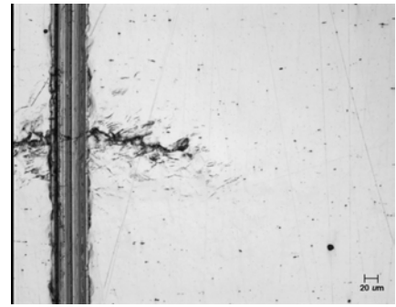
A36, before overload 2, flat
