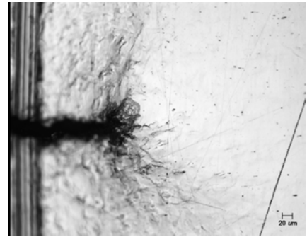
A36, after overload 9, flat
