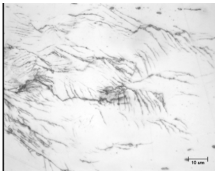
1018, before overload 3, flat
