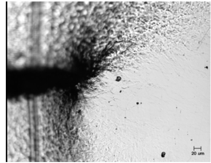
A588, after overload 10, flat
