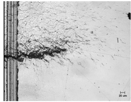
A514, before overload 11, flat
