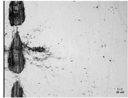
A36, after overload 3, flat
