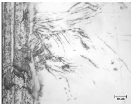
1018, before overload 6, flat
