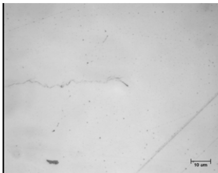
A2r60, before overload 1, flat
