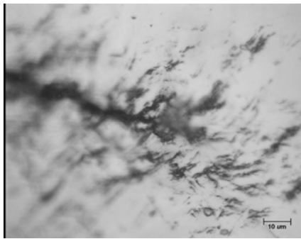
HPS70, after overload 9, flat
