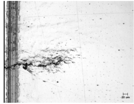
1018, after overload 4, flat
