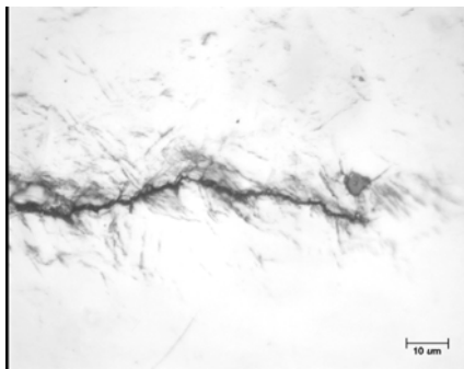
A514, before overload 4, flat
