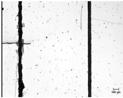
A588, before overload 3, flat
