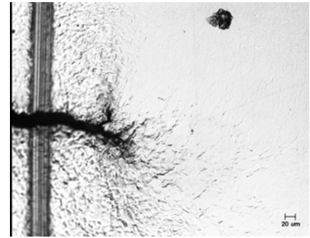
HPS70, after overload 10, flat
