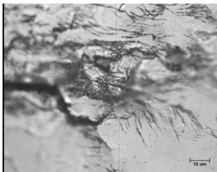
1018, after overload 8, flat
