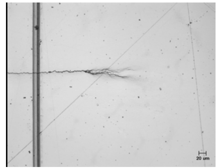
A2r60, after overload 1, flat
