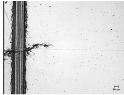
1018, after overload 1, flat
