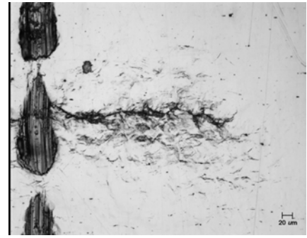
A36, after overload 5, flat
