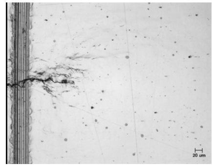
1018, after overload 3, flat
