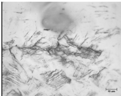
A36, before overload 4, flat
