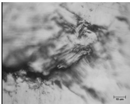
A514, after overload 10, flat
