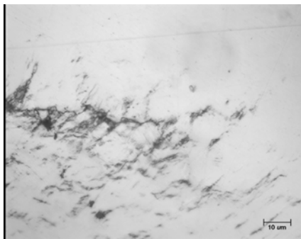
HPS70, before overload 6, flat
