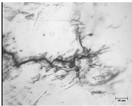
A36, after overload 7, flat
