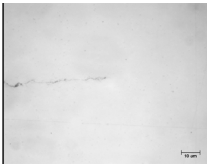
A2r50, before overload 1, flat
