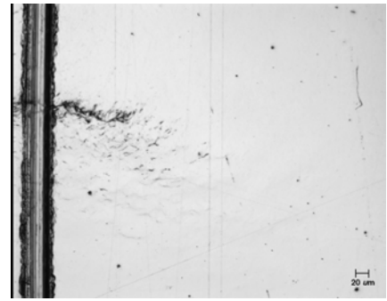
HPS70, before overload 8, flat
