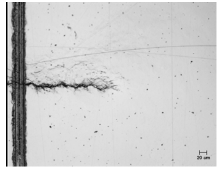
A514, before overload 5, flat
