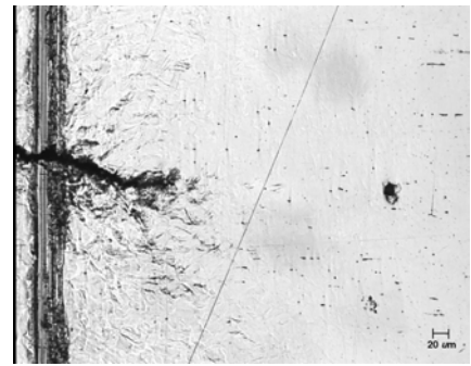
A36, after overload 8, flat
