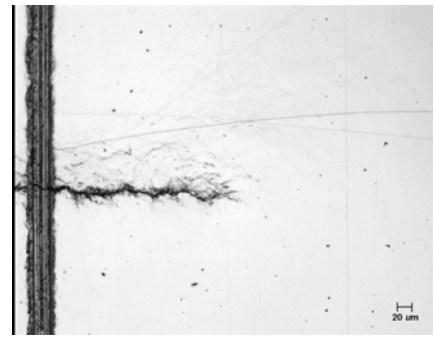
A514, after overload 5, flat
