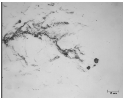
HPS70, before overload 1, flat
