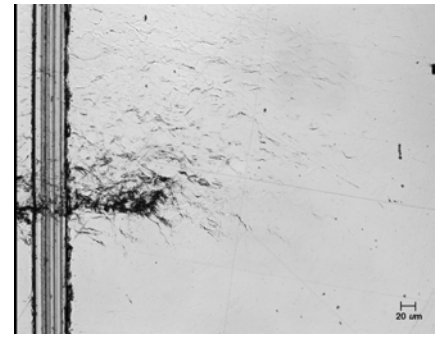
A514, before overload 10, flat
