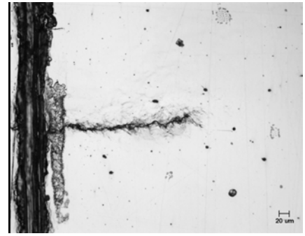
A588, after overload 4, flat
