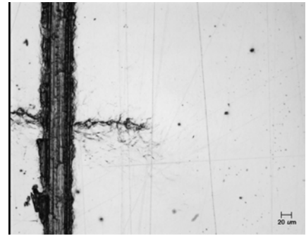
HPS70, after overload 3, flat
