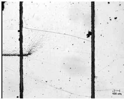
A588, after overload 8, flat
