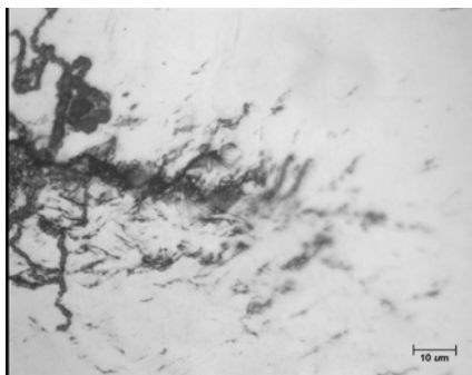
HPS70, after overload 7, flat
