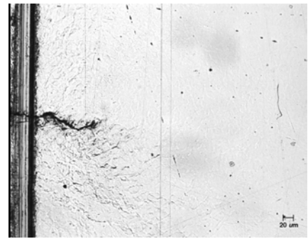
HPS70, after overload 8, flat
