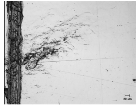
1018, before overload 7, flat
