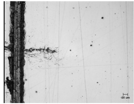
HPS70, before overload 3, flat
