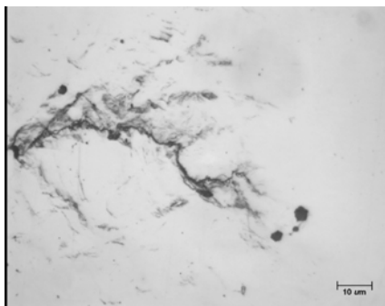
HPS70, after overload 1, flat
