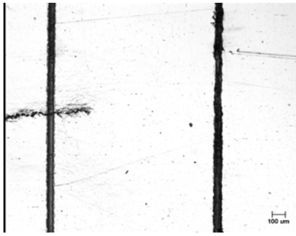
1018, before overload 5, flat
