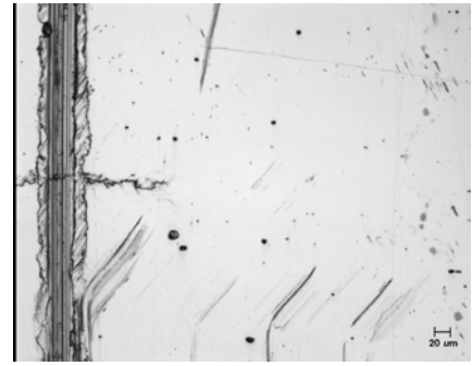
A588, after overload 1, flat
