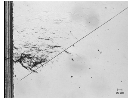
A514, before overload 9, flat
