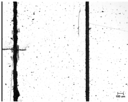
A588, after overload 3, flat
