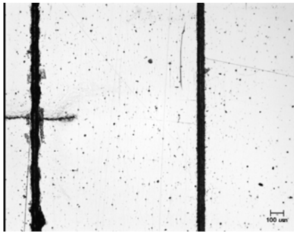
A588, before overload 4, flat
