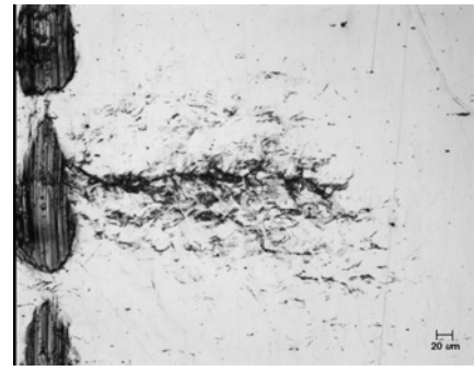
A36, before overload 5, flat
