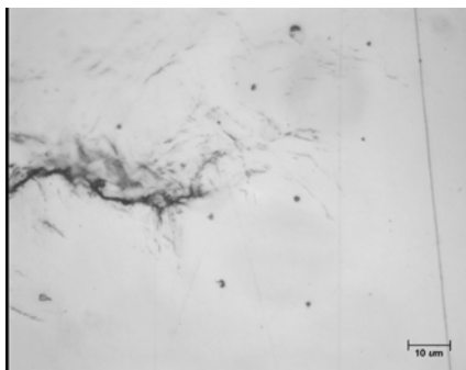
A514, after overload 2, flat
