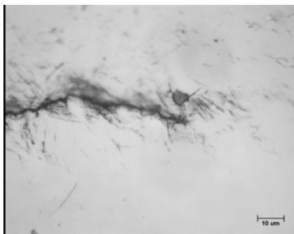
A514, after overload 4, flat
