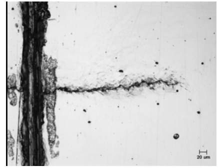
A588, after overload 5, flat
